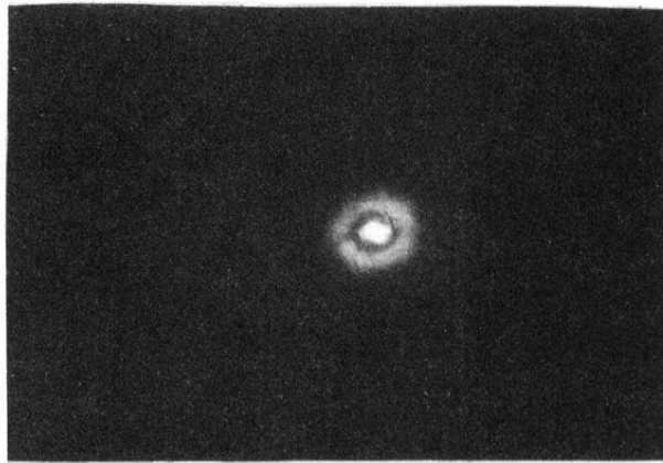
FIG. 7. Far-field pattern of a 138\text{-}\mu\text{m} -thick sample at a pump-laser intensity of 600\text{ W/cm}^2 , (a) with and (b) without a superposed quasistatic electric potential of 4\text{ V} .
