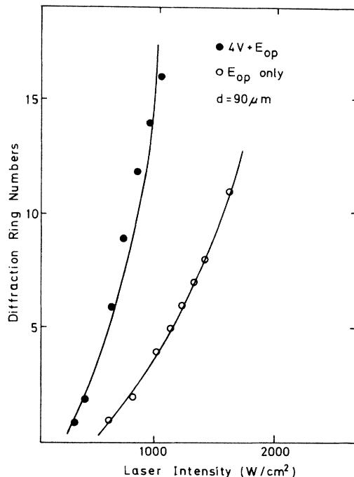
FIG. 6. Number of far-field rings for a 90- \mu m-thick sample is plotted as a function of pump-laser intensity. The solid circles show data with a biased quasistatic electric potential of 4.1 V. The solid curves are drawn freehand as a guide to the eye.
