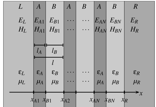
Fig. 1. The stratified one-dimensional N -layer medium and its surroundings. Slabs A and B , which, respectively have physical widths l_A and l_B , together form a single layer of thickness l . Along the principal axis, the x -axis, the interface coordinates have been written. The permittivities and permeabilities of material m = L, A, B, R are, respectively given by \epsilon_m and \mu_m . Also indicated is the labeling of the electric ( E ) and magnetic ( H ) field amplitudes in the various homogeneous subspaces of the system.
