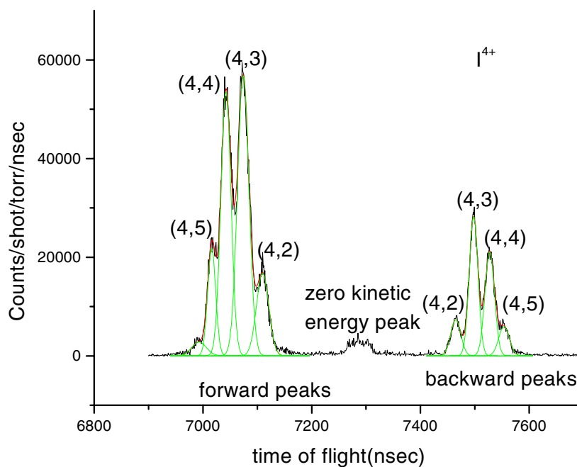
Figure 2. Typical TOF spectrum. (This figure is in colour only in the electronic version)
