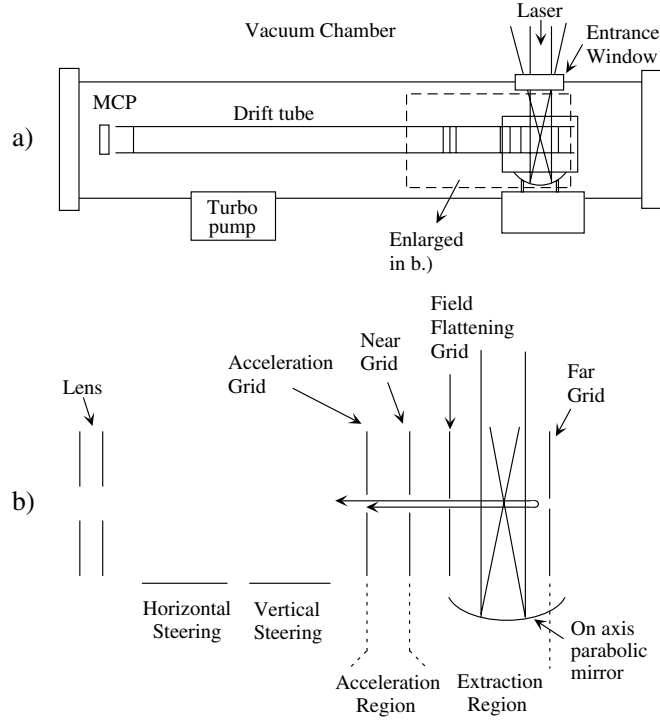
Figure 1. (a) Time of flight chamber. (b) Detail of electrostatic grids.
