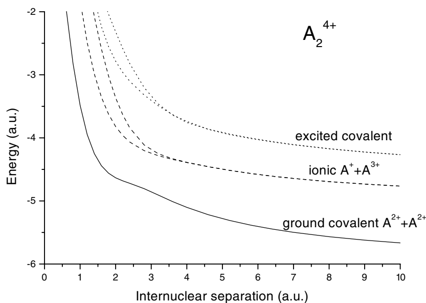
Figure 7. Covalent and ionic PE curves of a 1D molecule calculated using the procedure (see footnote 3). The ground covalent state of the molecule is represented by the full curve, the lowest lying ionic states by the broken curves and the excited covalent states by the dotted curves.
