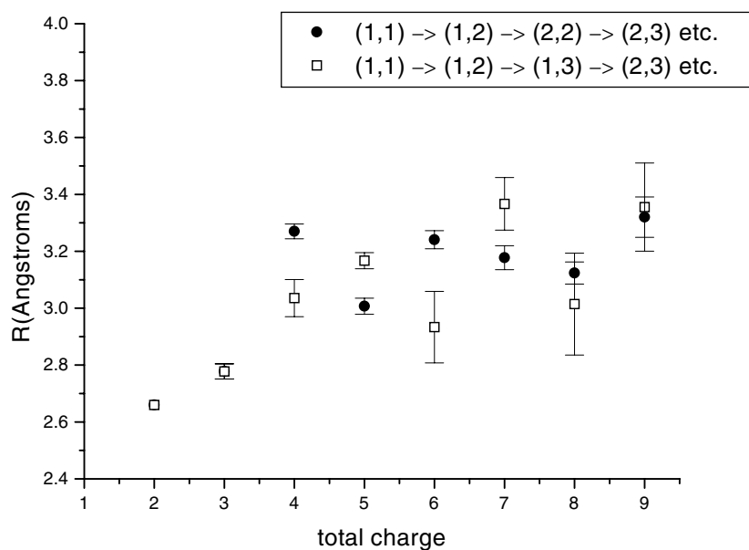
Figure 3. Internuclear separation at ionization (one-electron) for the symmetric and asymmetric pathways as a function of the total charge on the molecule. Error bars in our data reflect the uncertainty in \Delta t (see equation (4)) determined by fitting the various peaks in the TOF spectrum (see figure 2, for example).
