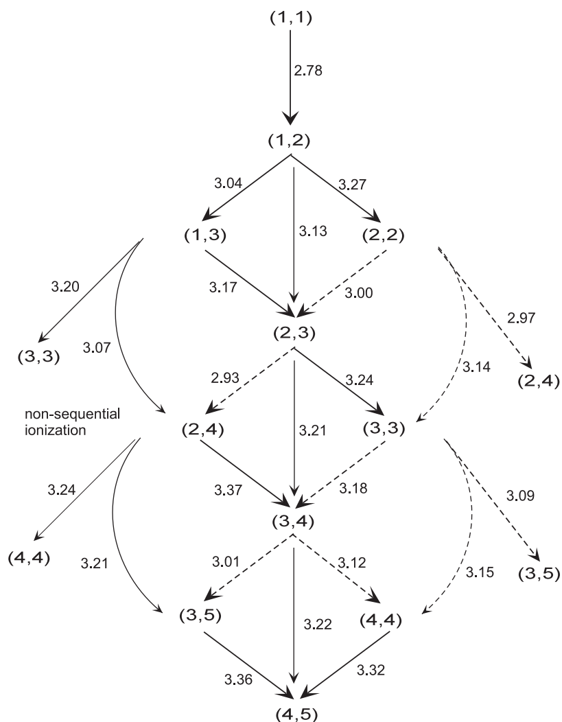
Figure 8. One- and two-electron ionization pathways in molecular iodine.
