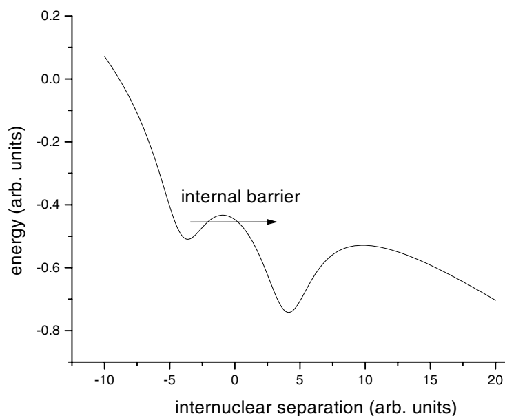
Figure 6. Schematic of process A where the electrons in the upper well tunnel through the small internal barrier at R_c .
