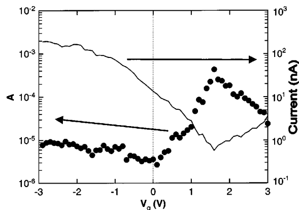
FIG. 3. The scaled noise (circles) and the drain current (line) for a typical device plotted versus the gate bias applied to the Si substrate. The noise has a minimum near V_g=0 and rises rapidly for positive gate biases. The noise peaks at the bias point ( V_g=1.6 V), at which the network inverts to n -type conduction.
