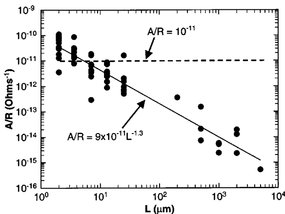
FIG. 2. The same data as in Fig. 1 plotted as A/R versus the electrode spacing L . The dashed line represents A/R=10^{-11} (Ref. 12) and the solid line is a least-squares power-law fit to the data. A clear relationship between the level of 1/f noise and the device size is established.
