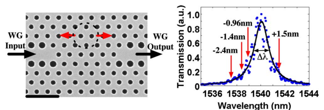
FIG. 1. (Color online) Left: SEM of cavity region. The innermost holes were shifted s=0.16a . Scale bar: 1 \mu\text{m} . Right: Cavity resonance with arrows indicating various detuning regions where pump-probe measurements were carried out.
