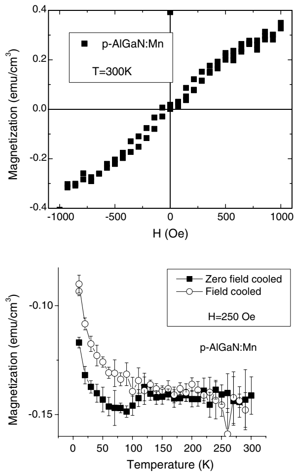
Figure 23. 300 K magnetization as a function of field (top) and field-cooled (FC) and zero field-cooled (ZFC) magnetization (bottom) versus temperature for AlGaN implanted with 3 \times 10^{16} Mn + annealed at 1000 °C for 2 min.
