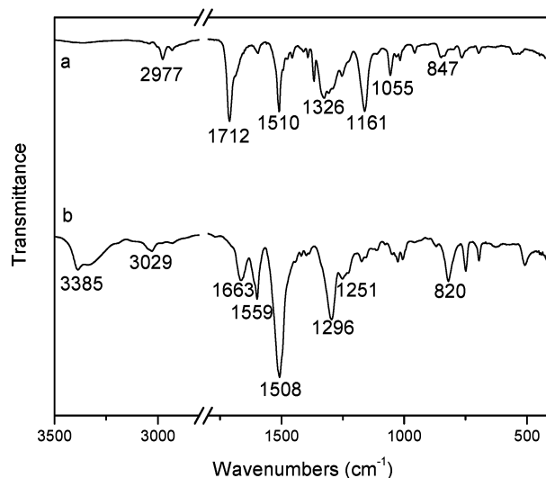
Figure 3. FTIR spectra of (a) t -Boc-protected polymer 2 and (b) polymer 2.
