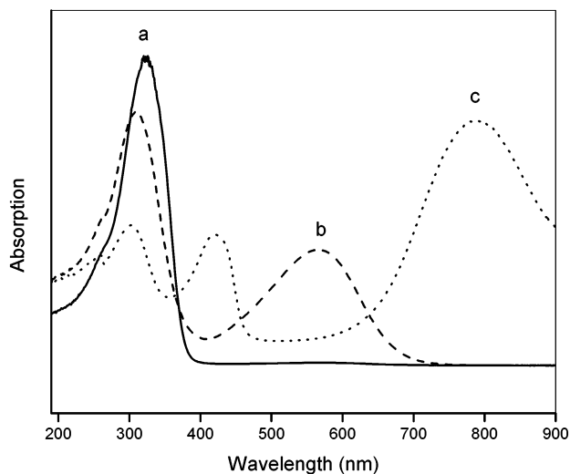
Figure 4. UV-vis spectra of polymer 2 in DMF solution: (a) reduced, (b) oxidized, and (c) doped with sulfuric acid.
