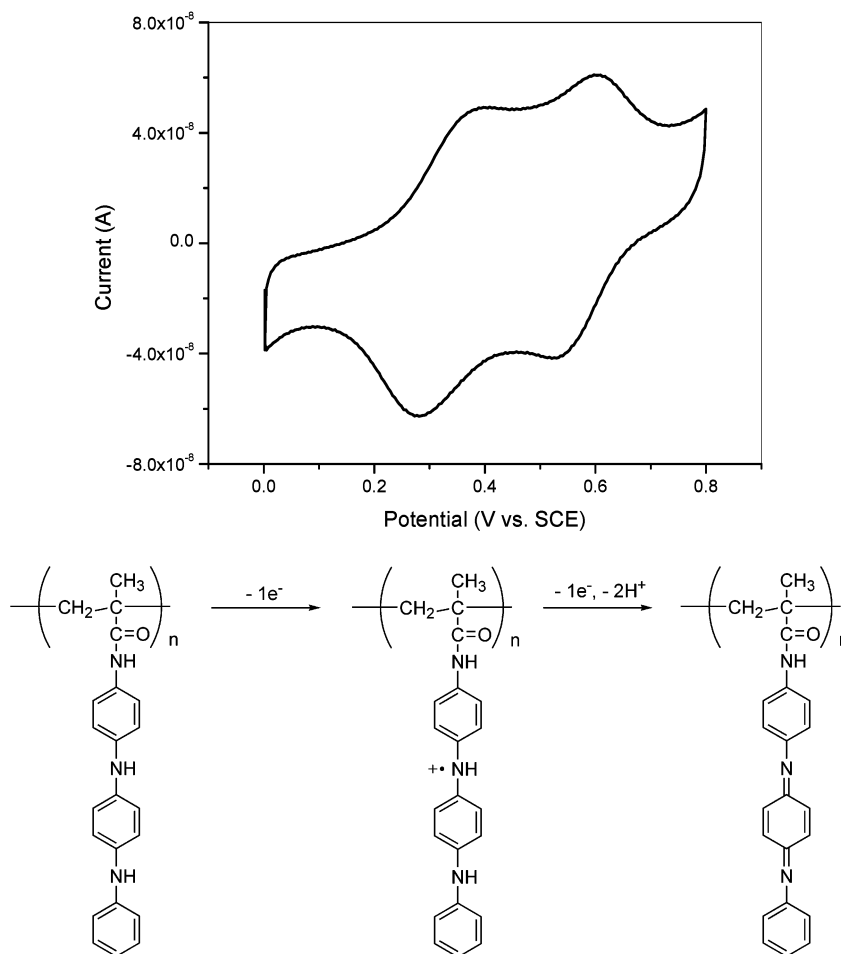
Figure 5. Cyclic voltammogram of polymer 1 , measured in aqueous \text{H}_2\text{SO}_4 (1.0 M) with scan rate of 100 mV/s. The proposed oxidation mechanism is shown below.
