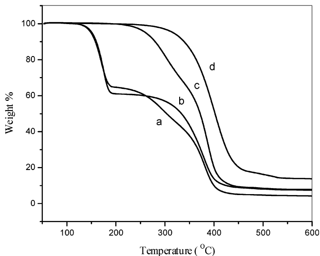
Figure 2. TGA thermograms of (a) t -Boc-protected polymer 1, (b) t -Boc-protected polymer 2, (c) polymer 1, and (d) polymer 2, carried out in a nitrogen atmosphere.
