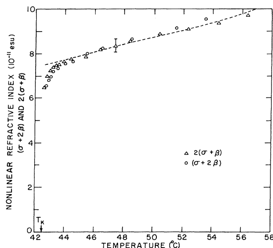
FIG. 2. Nonlinear refractive indices 2(\sigma + \beta) and \sigma + 2\beta as a function of temperature. The dashed curve is a theoretical curve obtained from Eq. (4) by assuming \nu = \nu_0 \exp(2800^\circ\text{K}/T) and \Delta\chi a constant.
