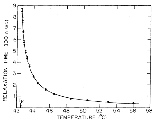
FIG. 1. Relaxation time \tau of the order parameter as a function of temperature. The solid curve is the theoretical curve obtained for \tau = \nu/a(T - T^*) with T^* = 314.7^\circ\text{K} and \nu = \nu_0 \exp(2800^\circ\text{K}/T) . The dots are the experimental data points.
