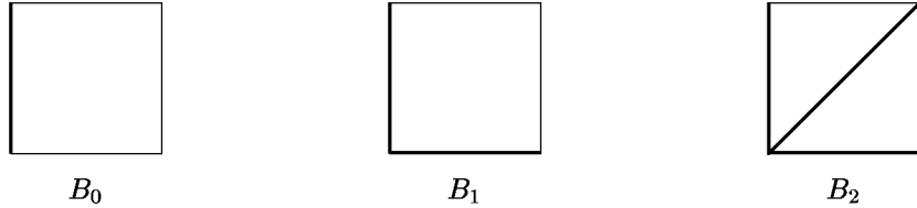
FIGURE 17. Three arc systems.
