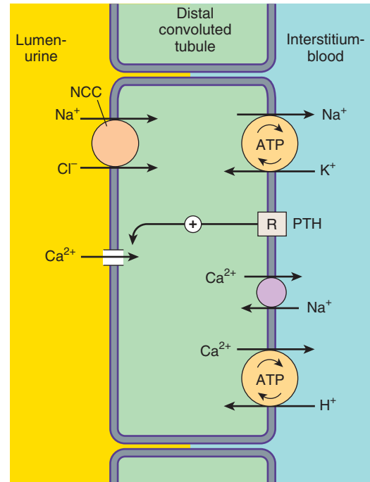
FIGURE 15-4 Ion transport pathways across the luminal and basolateral membranes of the distal convoluted tubule cell. As in all tubular cells, \text{Na}^+/\text{K}^+ -ATPase is present in the basolateral membrane. NCC is the primary sodium and chloride transporter in the luminal membrane. R, parathyroid hormone (PTH) receptor.
