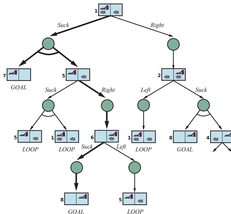
Figure 4.10 The first two levels of the search tree for the erratic vacuum world. State nodes are OR nodes where some action must be chosen. At the AND nodes, shown as circles, every outcome must be handled, as indicated by the arc linking the outgoing branches. The solution found is shown in bold lines.
