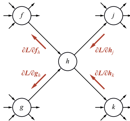
Figure 22.6 Illustration of the back-propagation of gradient information in an arbitrary computation graph. The forward computation of the output of the network proceeds from left to right, while the back-propagation of gradients proceeds from right to left.
