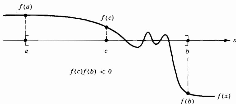
Figure 3.1(b) Bisection method selects right subinterval
