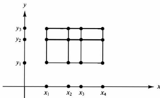
Figure 6.15 A Cartesian grid of nodes
