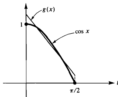
Figure 6.11 Approximating \cos x on the interval [0, \pi/2]
