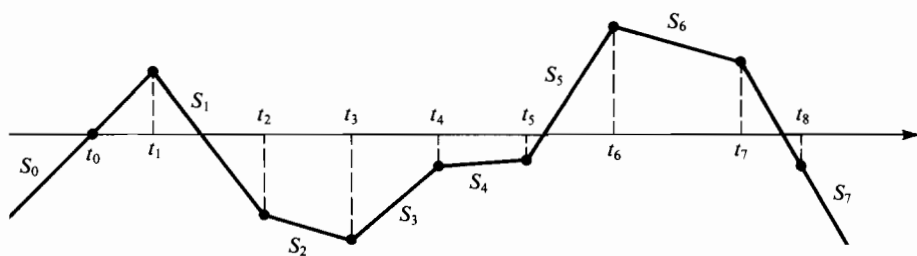
Figure 6.3 A spline of degree 1
