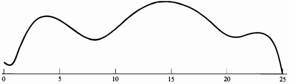
Figure 6.4(b) Spline curve with low tension ( \tau = 0.1 )
