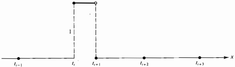
Figure 6.7 The B-spline B_i^0
