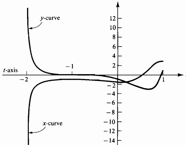
Figure 8.3 Solution curves for Example 3
