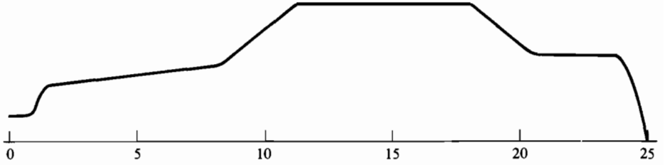
Figure 6.4(a) Spline curve with high tension ( \tau = 10 )
