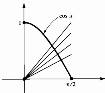
Figure 6.10 Approximating \cos x by \lambda x
