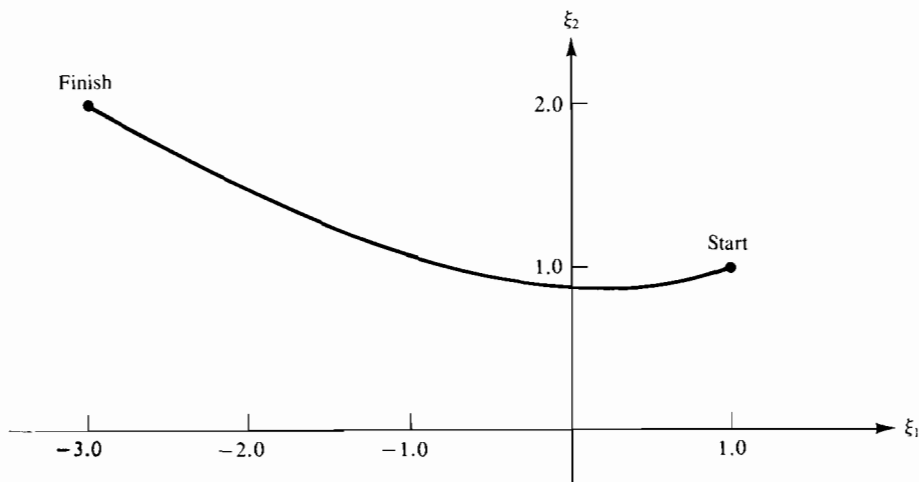
Figure 3.7 The path generated in Example 2
