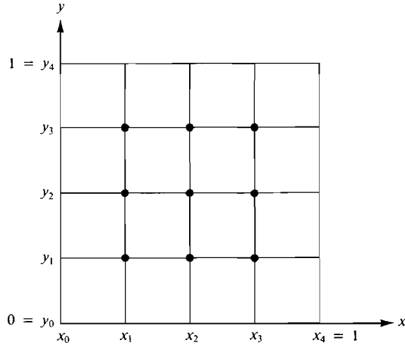
Figure 9.4 Mesh on unit square
