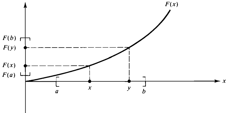
Figure 3.6 Graphical example of contractive mapping
