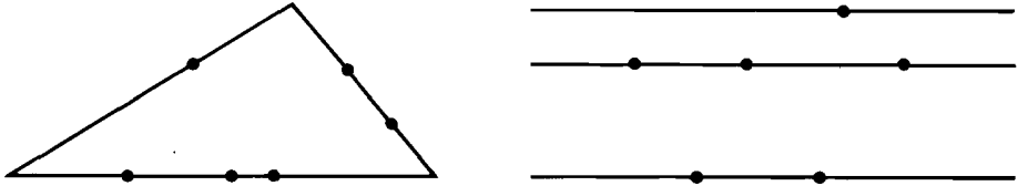
Figure 6.16 Node sets for interpolation by \Pi_2(\mathbb{R}^2)
