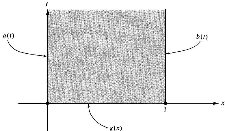
Figure 9.2 Solution domain
