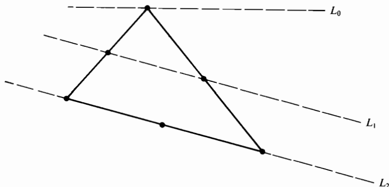
Figure 6.20 Applying Theorem 2
