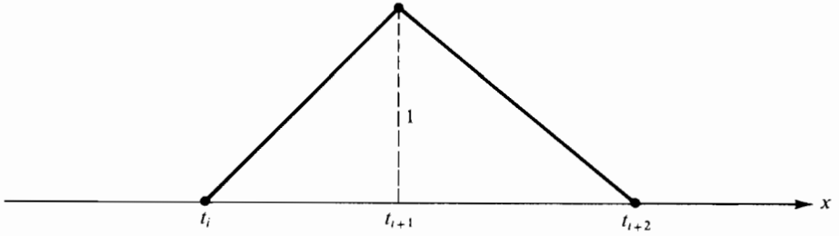
Figure 6.8 The B-spline B_i^1
