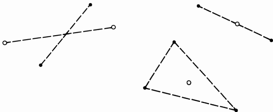
Figure 6.12 Critical points in a best approximation
