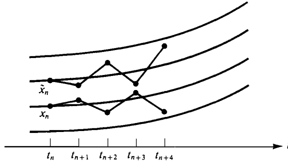
Figure 8.2 Effect of changing initial conditions
