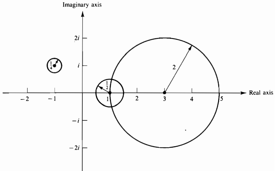
Figure 5.1 Gershgorin disks
