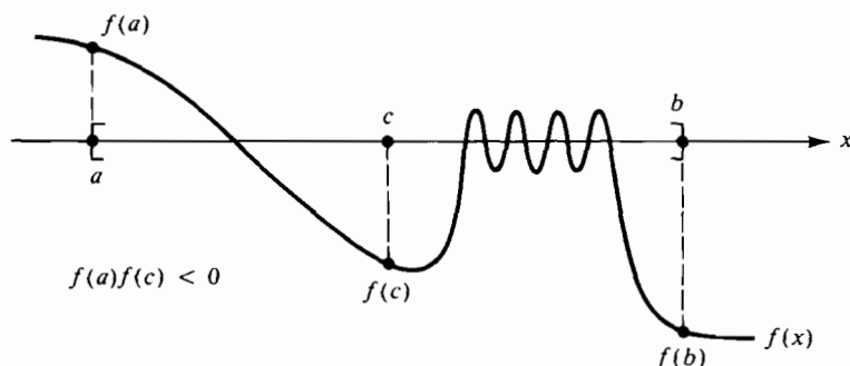
Figure 3.1(a) Bisection method selects left subinterval
