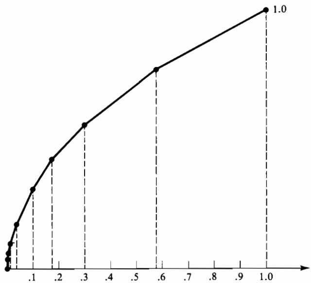
Figure 6.23 Adaptive spline approximation of degree 1
