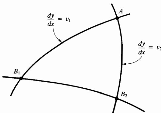
Figure 9.10 Characteristic curves AB_1 and AB_2
