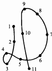
Figure 6.6 Script letter from eleven knots
