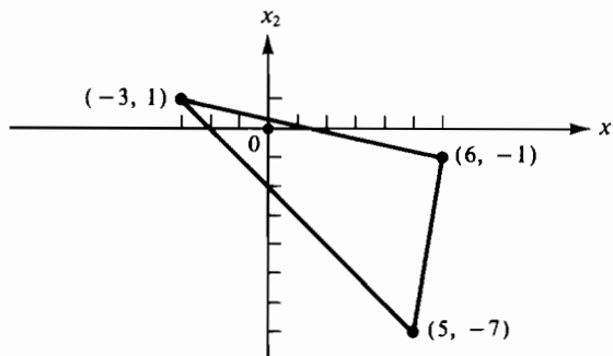
Figure 6.14 Zero in the hull of three points
