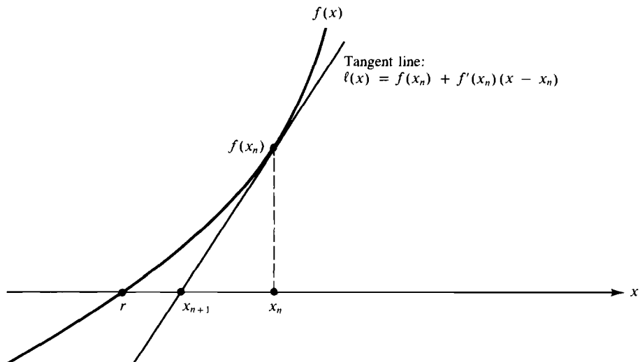
Figure 3.3 Geometric interpretation of Newton's method
