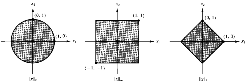
Figure 4.1 Unit cells in \mathbb{R}^2 for three norms
