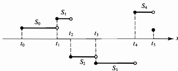
Figure 6.2 A spline of degree 0
