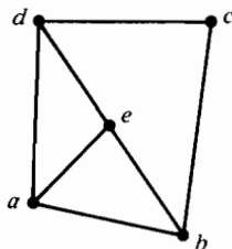
Figure 9.6 An improper triangulation
