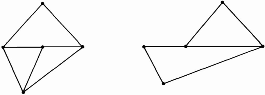
Figure 6.18 Illegal triangulations
