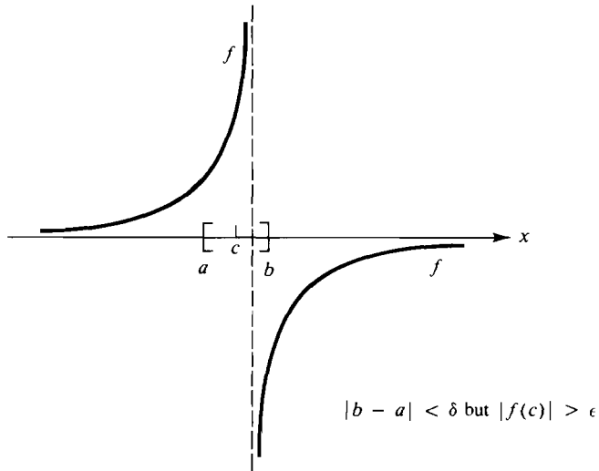
Figure 3.2(b) Criterion |f(c)| < \epsilon failure
