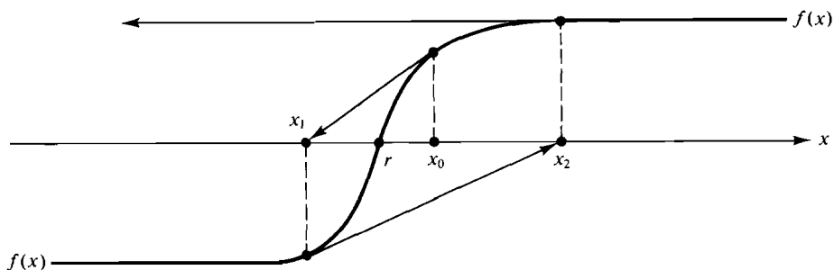
Figure 3.4 Example of nonconvergence of Newton's method
