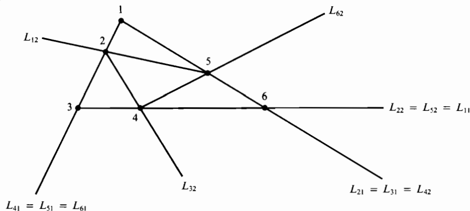
Figure 6.17 Illustrating Theorem 3
