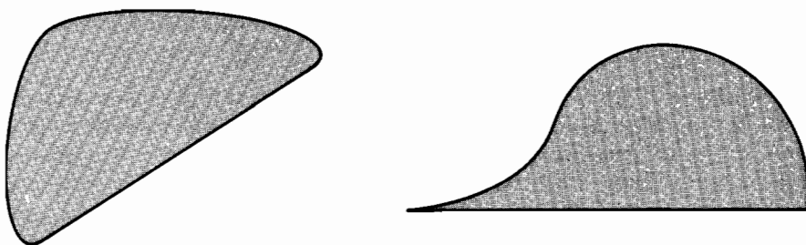
Figure 6.13 A convex set and a nonconvex set
