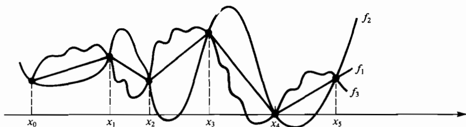
Figure 7.1 Three continuous functions through six points
