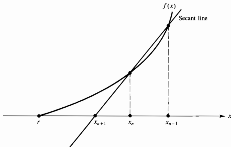
Figure 3.5 Geometric interpretation of secant method
