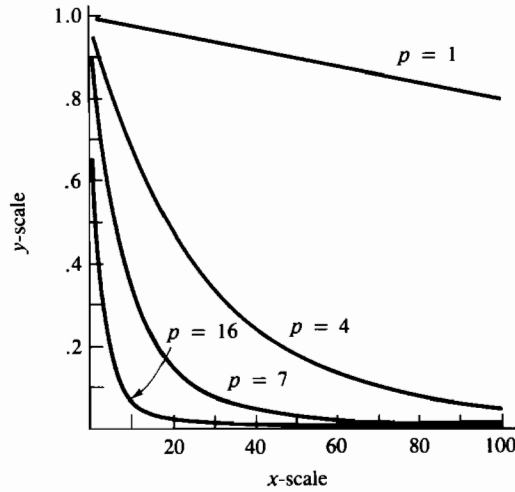
Figure 9.14 Reduction of error in 100 iterations
