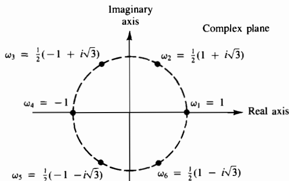
Figure 6.1 The 6 sixth roots of unity
