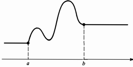
Figure 6.9 Extension of f
