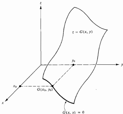
Figure 1.1 Surface G intersects xy -plane showing curve G(x, y) = 0
