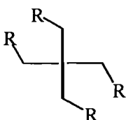
( S_4 )
