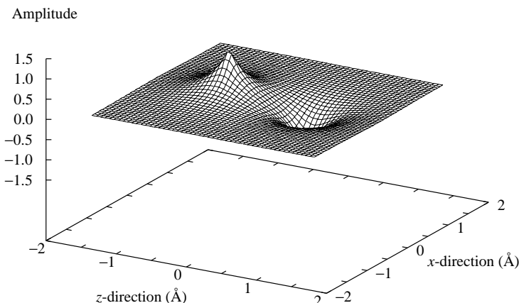
Figure 10.4. The third SCVB orbital for the \text{He}_2^+ ion. The orbital amplitude is given in the x - z plane.
