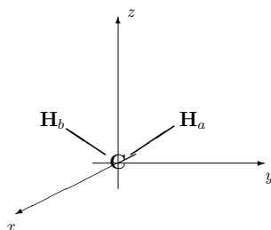
Figure 13.1. Orientation of the CH 2 diradical.
