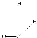
Figure 16.7. The true saddle point for the dissociation of \text{H}_2\text{CO} . This figure is drawn to scale as accurately as possible.
