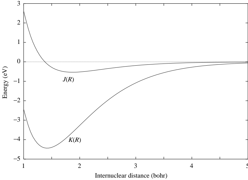
Figure 2.4. The relative sizes of the J(R) and K(R) integrals.
