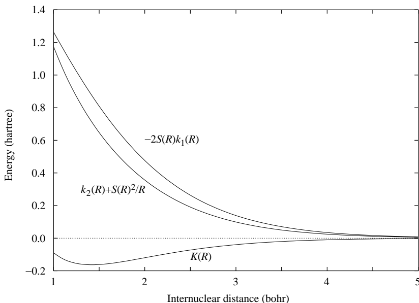
Figure 2.6. Comparison of the sizes of k_2 + S^2/R and -2k_1S that comprise the positive and negative terms in the exchange integral.
