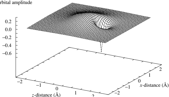
Figure 10.6. The first SCVB orbital for the BeH molecule and associated with the Be nucleus. This has the general appearance of an s - p hybrid pointed toward the H atom, and we denote it the inner hybrid, h_i . The orbital amplitude is given in the x - z plane, which contains the nuclei.
