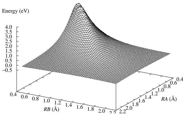
Figure 14.3. The difference between the energy surfaces for the conversion of 2\text{H}_2 \rightarrow 2\text{H}_2 in D_{2h} geometries and 3\text{H}_2 \rightarrow 3\text{H}_2 in D_{3h} geometries. The energy is per \text{H}_2 molecule. NB We have changed the aspect from that of Figs. 14.1 and 14.2.
