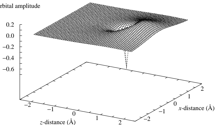
Figure 10.7. The second SCVB orbital for the BeH molecule and associated with the Be nucleus. This has the general appearance of an s - p hybrid pointed away from the H atom, and we denote it the outer hybrid, h_o . The orbital amplitude is given in the x - z plane, which contains the nuclei.
