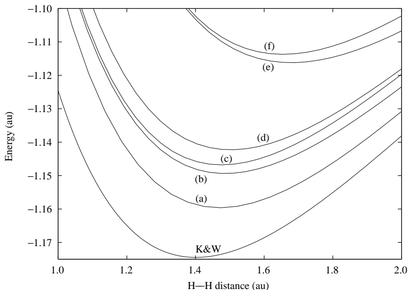
Figure 2.9. A detailed view of the adiabatic energies of the \text{H}_2 molecule with the DZP basis.
