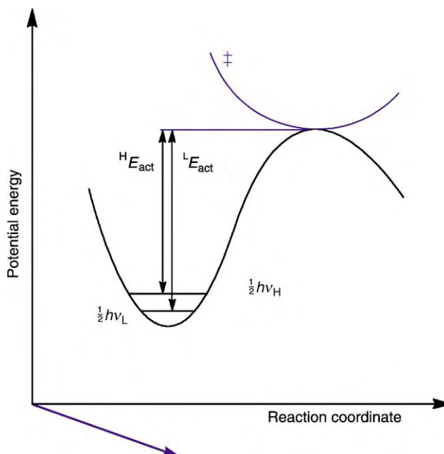
FIGURE 2 Energy diagram representing the origin of KIE on cleaving a C–H or C–L bond (H = 1 H, L = 2 H or 3 H). In this picture, a stretching mode in the reactant has been converted to a translational mode in the transition state.
