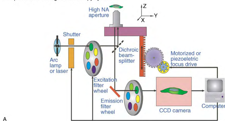
Image deconvolution
