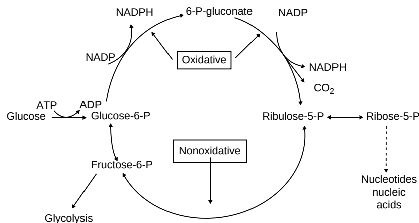
FIGURE 1 Depiction of the pentose phosphate pathway as a cycle composed of oxidative and nonoxidative segments.
