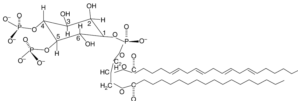
FIGURE 1 Structure of phosphatidylinositol-4,5-bisphosphate. The structure shows PtdIns-4,5-P 2 , which contains an inositol head group connected to a diacylglycerol via a phosphodiester linkage. The fatty acid moiety is typically stearyl-arachidonyl. The inositol head group can be phosphorylated at one of three positions, D-3, D-4, and D-5. Shown are phosphate groups at the D-4 and D-5 position in PtdIns-4,5-P 2 . Phosphoinositide 3-kinases phosphorylate the D-3 position of PtdIns-4,5-P 2 to produce PtdIns-3,4,5-P 3 .
