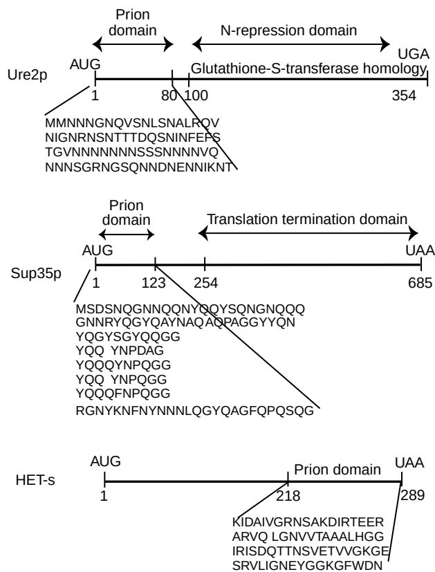
FIGURE 2 Prion domains of Ure2p, Sup35p, and HET-s. While the prion domains of Ure2p and Sup35p are rich in N and Q, that of HET-s is rich in neither.
