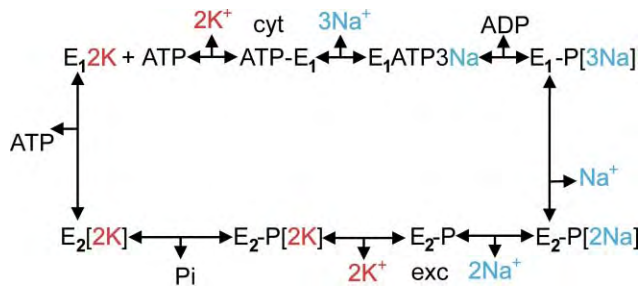
FIGURE 1 \text{E}_1 - \text{E}_2 reaction cycle of the \text{Na}^+/\text{K}^+ pump with ping-pong sequential cation translocation. [\text{Na}^+] or [\text{K}^+] ions within brackets are occluded or tightly bound and prevented from exchanging with medium cations.
