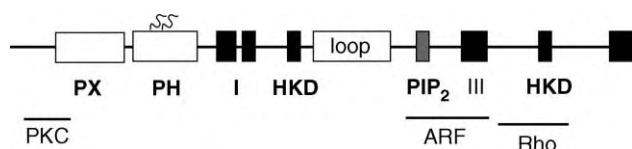
FIGURE 3 PLD structure. Mammalian PLD contains catalytic domains (HKD, I, III, and C-terminus), a PI4,5P 2 interacting motif (PIP 2 ), and PX and PH-membrane association domains. The PH domain is palmitoylated in PLD1. PLD1's activators Rho, ARF, and PKC interact with PLD1 within the regions depicted to activate it.
