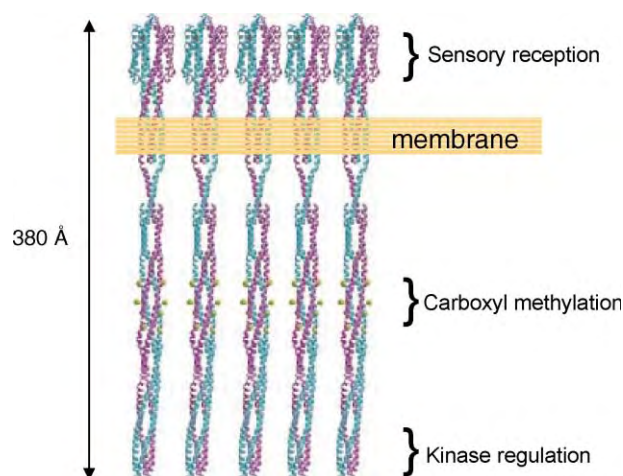
FIGURE 1 Model of the chemotaxis receptor fibers. Transmembrane methylatable receptors are employed as sensors in bacterial chemotaxis.
