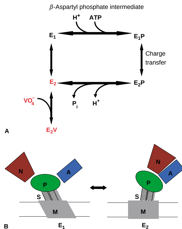
FIGURE 2 (A) The H^+ -ATPase reaction cycle. See text for explanation. VO_4^- , vanadate, a potent P-type ATPase inhibitor. (B) Major domain movements that occur during conversion of the ATPase from the E_1 (cation-bound) to the E_2 (cation-free) conformation. N, nucleotide-binding domain; P, phosphorylation domain; A, actuator domain; S, stalk region; M, membrane sector formed by 10 transmembrane helices.
