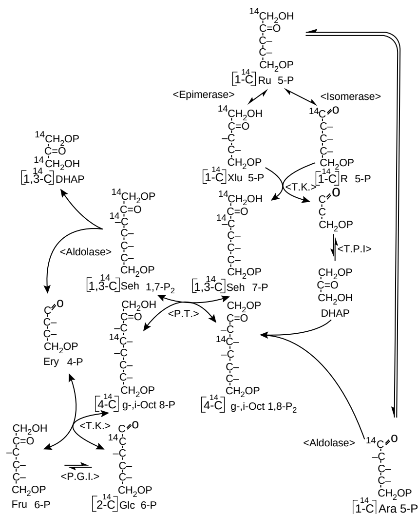
FIGURE 4 The proposed reaction sequence of the nonoxidative segment of the L-type pentose pathway. The [1-^{14}\text{C}] -ribulose 5-P substrate is the labeled product of the Figure 1 scheme and the reactions display the theoretical and the found distributions of ^{14}\text{C} -isotope from pentose 5-P substrate into labeled Glc, triose and Oct intermediates, and products. The epimerase, isomerase, and TK enzymes are the same catalysts that operate in the F-type pathway. New enzymes are arabinosephosphate isomerase that interconverts arabinose and ribulose 5-phosphates, aldolase, triosephosphate isomerase (EC 5.3.1.1), glucosephosphate isomerase and D-glycero-D-ido-octulose 1,8-bisphosphate: D-alto-Heptulose 7-phosphotransferase, called phosphotransferase (PT) (see Arora, K. K., Cortis, P. A., Bleakley, P. A., and Williams, J. F. (1985) Identification and measurement of D-glycero-D-ido-octulose 1,8-bisphosphate: D-alto heptulose 7-phosphotransferase enzyme in tissues with L-type pentose phosphate pathway activity. Int. J. Biochem. 17, 1329–1337). Besides new enzymes and intermediates, the L-type pathway is distinguished from the F-type pathway by the formation of Glc 6-P labeled in the 2 position by flux and in positions 4 and 6 by group-transfer enzyme exchanges involving the [1,3-^{14}\text{C}] -DHAP product. The triosephosphate formed by the F-type pathway is unlabeled.
