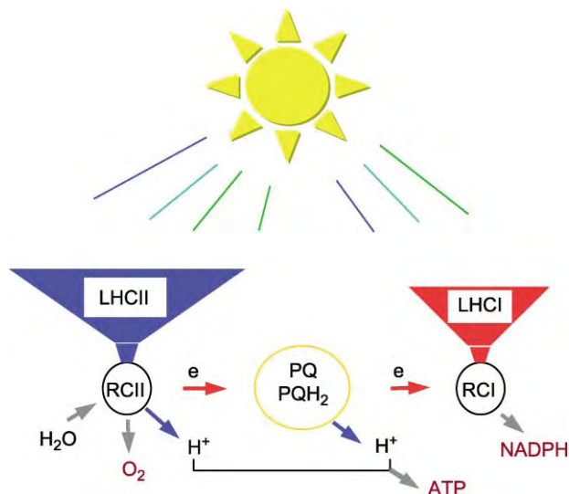
FIGURE 1 Photosynthetic electron transfer. LHCI and LHCII – light harvesting antenna of photosystem I and II, respectively; RCI and II – reaction centers; e – electrons; PQ and PQH 2 – intermediate electron carrier plastoquinone in oxidized and reduced form; H + – protons.
