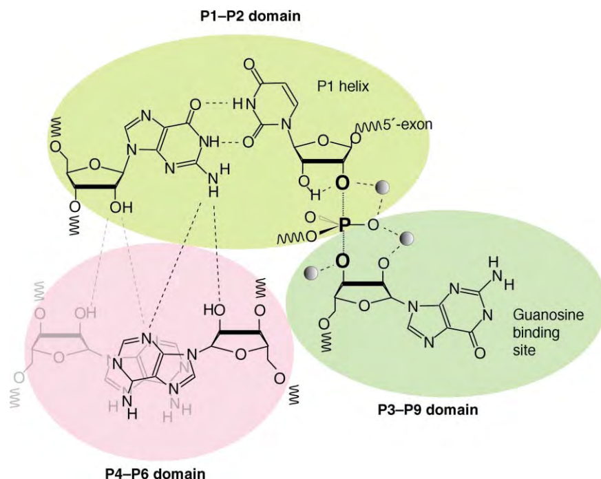
FIGURE 4 Interactions between the three domains in the transition state. Near the transition state for the ribozyme reaction, the bond between the 5' exon and the intron is partially broken and the bond between the guanosine substrate and the intron is partially formed. Three magnesium ions help orient the substrates and stabilize the transition state, facilitating catalysis. The G·U wobble at the 5' splice site is shaded yellow. The guanosine bound in the guanosine-binding site is shaded green. Adenosines within the P4–P6 domain involved in positioning the G·U wobble are shaded pink. Magnesium ions that participate in catalysis are drawn as spheres. Hydrogen bonds and metal interactions are indicated by dashed lines, and partial bonds are indicated by dotted lines.
