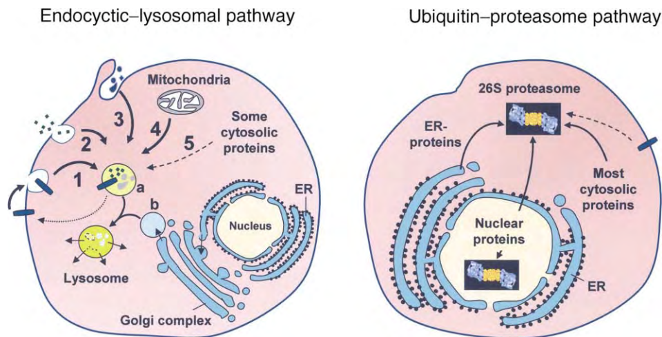
FIGURE 1 Pathways of protein breakdown in mammalian cells. Most intracellular proteins in the cytosol, nucleus, and endoplasmic reticulum (ER) are degraded by the ubiquitin–proteasome pathway (right panel). Extracellular and autophagocytized proteins and most membrane proteins are broken down within the endocytic–lysosomal compartment (left panel). Substrates are delivered to this pathway by receptor-mediated endocytosis (1), pinocytosis (2), phagocytosis (3), autophagy (4), and a selective process for some cytosolic proteins containing specific amino acid motifs (5). Some internalized membrane proteins are recycled back to the plasma membrane (dotted arrows). After the internalized material is enclosed in vesicles (a), the vesicle fuses with primary lysosomes (b), derived from the Golgi complex and ER, to form secondary lysosomes where final degradation takes place. Degradation products are transported across the lysosomal membrane into the cytosol. Some plasma membrane proteins are broken down by the ubiquitin–proteasome pathway, and some cytosolic proteins are degraded in lysosomes (dashed arrows). Although worn out mitochondria are cleared by autophagy, mitochondrial proteins are selectively broken down by their own ATP-dependent proteases.
