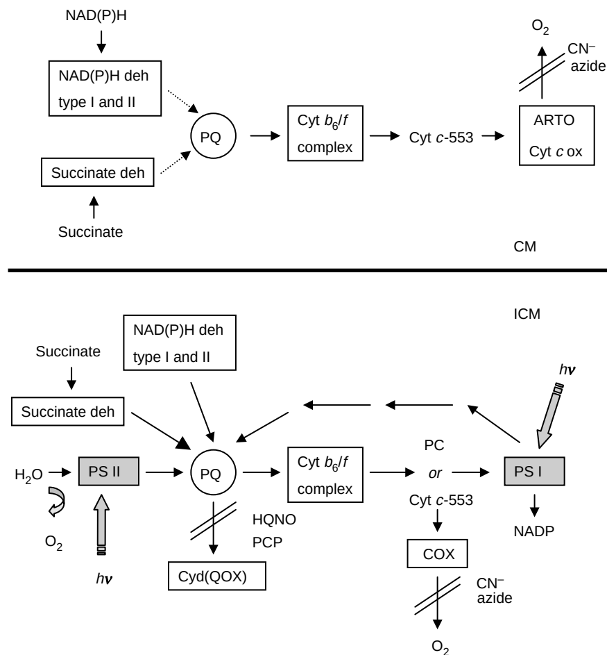
FIGURE 3 Working model of photosynthetic and respiratory electron transport chains in Synechocystis sp. strain PCC 6803 in CM and ICM. Membrane-bound redox complexes are indicated as rectangular boxes. Dotted arrows (CM redox chain) symbolize the lack of evidence for electron flow while the thickness of arrows (ICM redox chain) symbolize their relative activities. HQNO, 2-heptyl-4-hydroxy-quinoline-N-oxide; PCP, pentachlorophenol; CN^- , cyanide anion; PC, plastocyanin; PQ, plastoquinone pool; h\nu , radiant energy; see text for further details.
