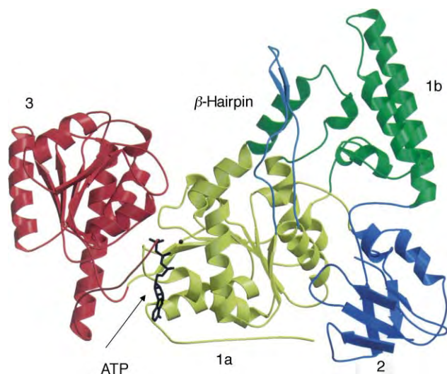
FIGURE 3 Structure of UvrB. Domains 1a, 1b, 2, and 3 are shown in yellow, green, purple and red, respectively. The \beta -hairpin bridging the gap between domains 1a and 1b is shown in cyan. The ATP molecule bound at the interface between domains 1 and 3 is indicated. (Reprinted from Theis, K., Chen, P. J., Skorvaga, M., Van Houten, B., and Kisker, C. (1999). Crystal structure of UvrB Provides insight into the mechanism of nucleotide excision repair. EMBO J. 18(24), 6899–6907, with permission of Oxford University Press.)
