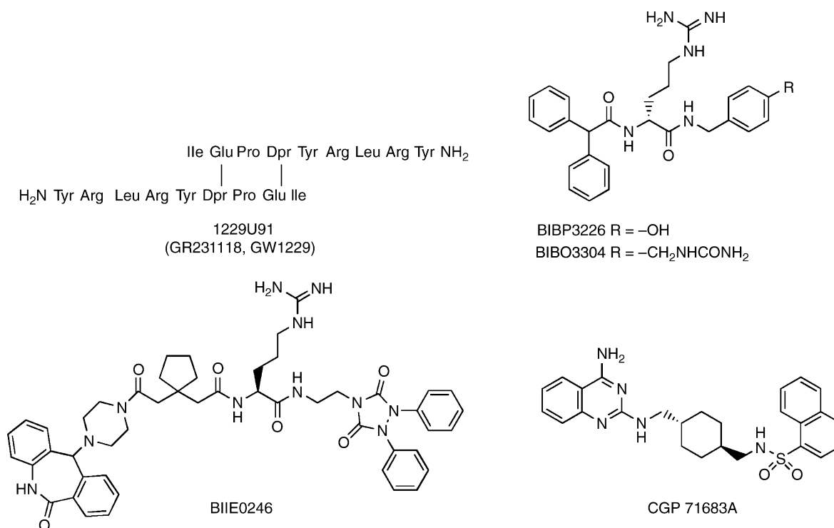
FIGURE 1 Structures of standard NPY receptor antagonists.
