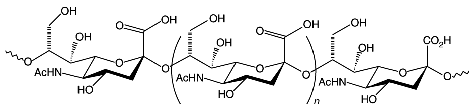
FIGURE 1 Structure of \alpha 2,8 -polysialic acid.
