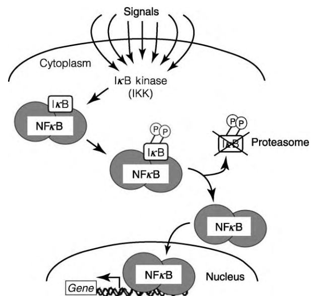
FIGURE 2 The NFκB signal transduction pathway. Under most circumstances, NFκB dimers (e.g., p50-RelA) are located in the cytoplasm of cells bound to inhibitory IκB proteins. Upon receiving an inducing signal, an IκB kinase (IKK) is activated. Active IKK phosphorylates IκB, and phosphorylated IκB then serves as a substrate for the ubiquitin-proteasome degradation pathway. Free NFκB can then enter the nucleus to increase or decrease specific target gene transcription. The system is eventually returned to its resting state through an auto-regulatory system, in that NFκB turns on expression of the gene encoding IκB, and newly synthesized IκB then resequences NFκB in the cytoplasm.
