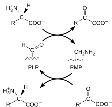
FIGURE 2 The transamination reaction by which amino groups are transferred from one carbon skeleton (in the form of an α-oxoacid) to another to form or to degrade an amino acid.
