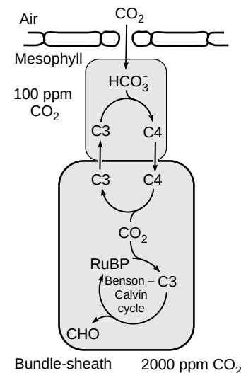
FIGURE 5 A simplified scheme for the mechanism of \text{C}_4 photosynthesis, showing how the \text{C}_4 cycle shuttles \text{C}_4 acids into bundle-sheath, where they are decarboxylated to raise the \text{CO}_2 concentration in the vicinity of Rubisco and thereby suppress photorespiration.
