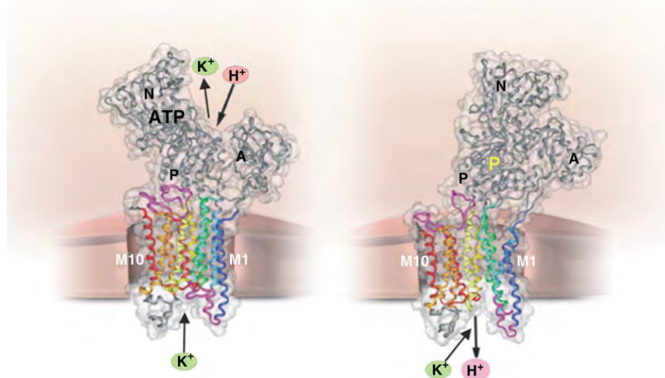
FIGURE 1 Proposed structure of the gastric H^+,K^+ -ATPase \alpha -subunit in E_1 (left) and E_2 (right) conformations. There are three lobes in the cytoplasmic domain: N (ATP binding), P (phosphorylation), and A (activation) regions. With binding of H^+ and MgATP to the E_1 form there is transient association of the N and P lobes with phosphorylation of asp386 and a conformational change to E_2P so that the A domain associates with the P domain. This change is transmitted to the membrane domain in the region of TM6 (dark yellow) and H^+ binding to the cation binding domain in the middle of the membrane domain is followed by release of H^+ and binding of K^+ from the luminal surface. There is then dephosphorylation and reformation of the E_1 conformation with release of K^+ to the cytoplasm.
