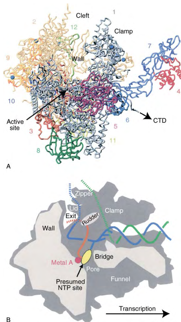
FIGURE 1 RNA polymerase II structures. (A) Ribbon model of yeast RNA polymerase II. The 12 subunits are shown in different colors. The active site metal ion A is depicted as a pink sphere. Zinc ions are shown as cyan spheres. (B) Schematic cut-away view of the pol II core elongation complex. The view is related to the one in (A) by a 90° rotation around a vertical axis. The DNA template and non-template strands are in blue and green, respectively, and the RNA is in red. Four of the bases in the DNA template strand are indicated as sticks protruding from the backbone. The yellow oval depicts the presumed binding site for the incoming nucleoside triphosphate substrate.
