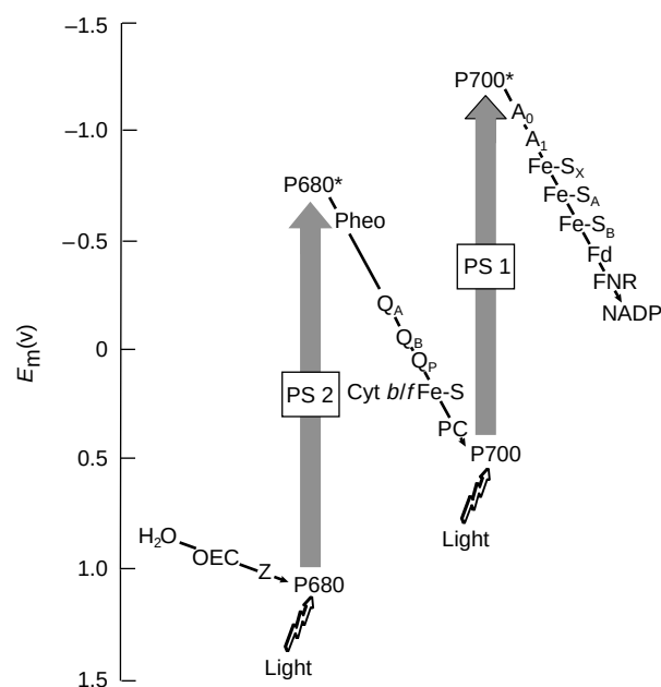
FIGURE 2 The Z-scheme of photosynthetic electron transport, showing the mid-point redox potentials of electron donors, acceptors, and carriers.
