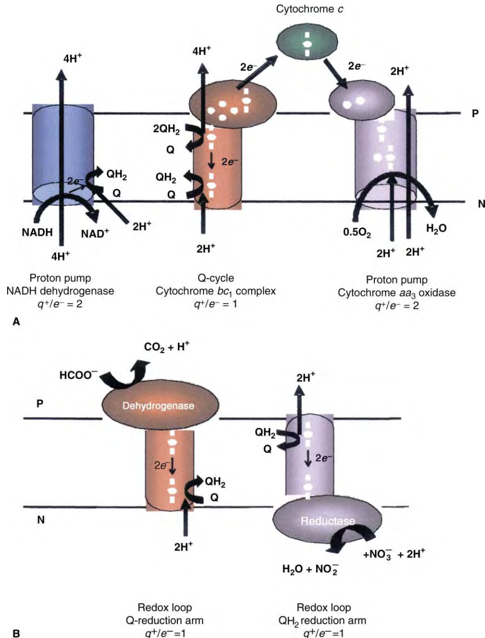
FIGURE 1 Mechanisms of energy conservation in respiration. (A) A basic mammalian mitochondrial electron transport chain illustrating proton pumps and Q-cycle mechanisms of energy conservation. (B) The organization of redox loops using periplasmic electron donors found in some cytochrome bc_1 complex-independent bacterial respiratory systems.
