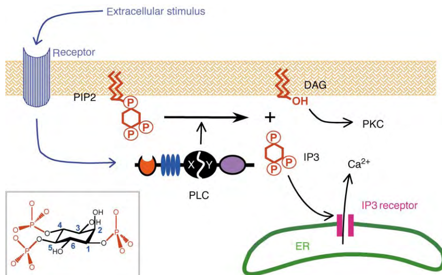
FIGURE 1 A scheme for the action of PLC in the cell. For abbreviations, see text. Inset shows chemical structure of IP3.
