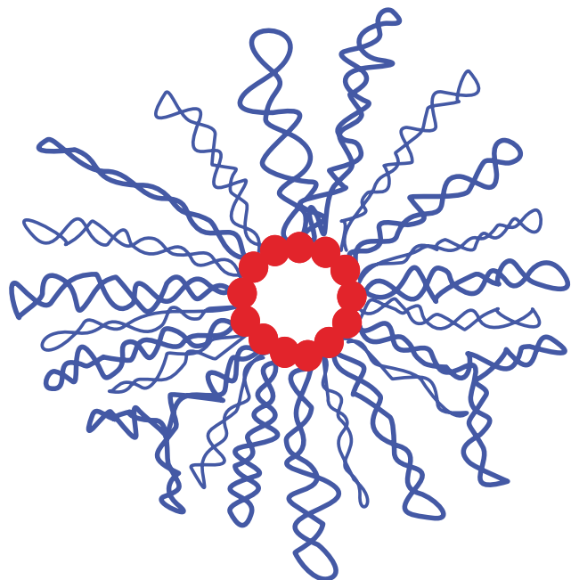
FIGURE 1 Organization of the bacterial nucleoid. A representation of the nucleoid liberated from the cell is shown. The red spheres at the core represent the nucleoprotein complexes that define the ends of the supercoiled domains. These complexes are thought to be composed of nucleoid-associated proteins and possibly topoisomerases. The blue ribbons represent the DNA making up the supercoiled domains. A typical nucleoid from E. coli has between 50 and 100 of these.
