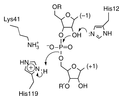
FIGURE 4 Catalytic mechanism of ribonuclease A. Histidine is particularly well suited to act as a general acid–base catalyst because its pK_a is close to physiologic pH. In RNase A, histidines 12 and 119 act as general base and acid, deprotonating the nucleophile and protonating the leaving group of the transesterification, respectively. Deprotonation of the 2'-OH makes it a better nucleophile, and protonation of the 5'-oxo leaving group lowers the energy of the product state. Lysine 41 (which has a positively charged side chain at physiologic pH) counteracts the increased negative charge at the scissile phosphate during the transition state, and thus helps lower the activation energy of the reaction.
