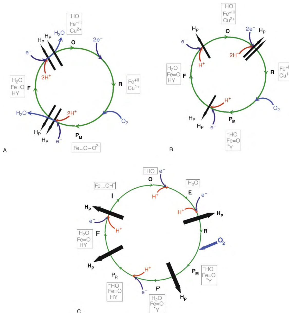
FIGURE 4 Catalytic cycles of cytochrome c oxidase. Classical, now obsolete cycle with only four states. The P-state erroneously has a peroxide anion bound to the heme a_3 -iron; two protons are pumped during the P to F-, and during the F to O transitions under consumption of two protons each. It is clear now, that only one proton is consumed during each transition. (A) Adaptation of the classical cycle to recent findings. Two protons are taken up already during the initial two-electron reduction of the enzyme, and two protons are pumped in this phase (under turnover conditions). The P_M -state contains a oxoferryl-iron, a tyrosine radical and a hydroxide in the binuclear center, only one proton is pumped during the P to F-, and during the F to O transitions. (B) A recent cycle with two P and two F-states. The protonations of the hydroxides in the binuclear sites of the P-states leads to proton pumping, each electron uptake is accompanied by a charge compensating proton uptake. Tyrosine radicals are present in the two-electron reduced states, tyrosines in the three-electron reduced states. One proton is pumped during the second reduction step, which could now be experimentally demonstrated. One electron is pumped during the F to O-transition as a result of the protonation of the oxo-group at the heme a_3 iron. (C)
