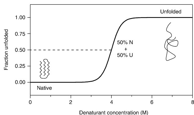
FIGURE 1 A cooperative protein unfolding–refolding transition. In a typical experiment, the native protein is incubated in solutions with increasing concentrations of denaturant such as urea or guanidinium chloride, and the fraction of unfolded molecules is determined by monitoring a spectroscopic signal, such as UV absorbance, fluorescence, or circular dichroism. For small monomeric proteins, the transition is usually highly cooperative, so that only the fully folded and unfolded forms are significantly populated and the fraction unfolded represents the relative concentrations of the two forms.
