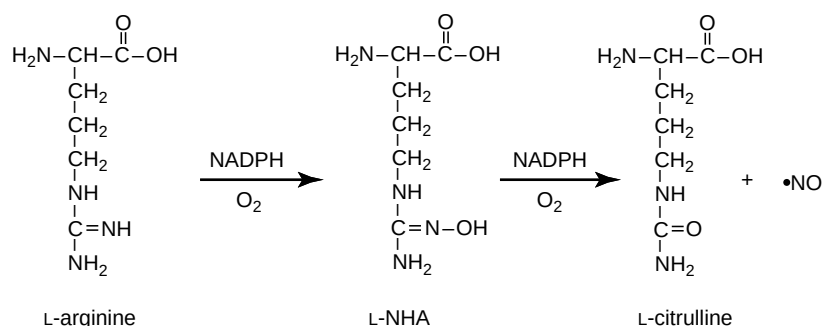
FIGURE 2 The reaction catalyzed by nitric oxide synthase. The substrate for the reaction is the amino acid L-arginine, which is converted to L-NHA and then to citrulline and \bullet\text{NO} . Although it has never been shown, it is assumed that the stereochemistry of citrulline at the \alpha -carbon remains unchanged.
