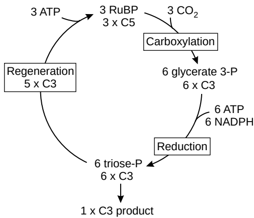
FIGURE 4 A simplified scheme for the Benson–Calvin cycle, showing the carboxylation of RuBP by Rubisco, reduction of glyceralate 3-P to triose-P, and regeneration of the initial acceptor from triose-P.
