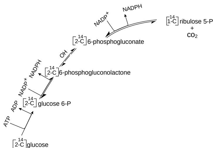
FIGURE 1 Reactions of the oxidative segment of the pentose pathway showing the conversion of [2\text{-}^{14}\text{C}] -glucose to \text{CO}_2 and [1\text{-}^{14}\text{C}] -ribulose 5-phosphate. Glucose is phosphorylated by hexokinase and oxidatively decarboxylated by the concerted actions of glucose 6-phosphate dehydrogenase, water at pH 7.4 or lactonase and 6-phosphogluconate dehydrogenase (see glossary for equation).
