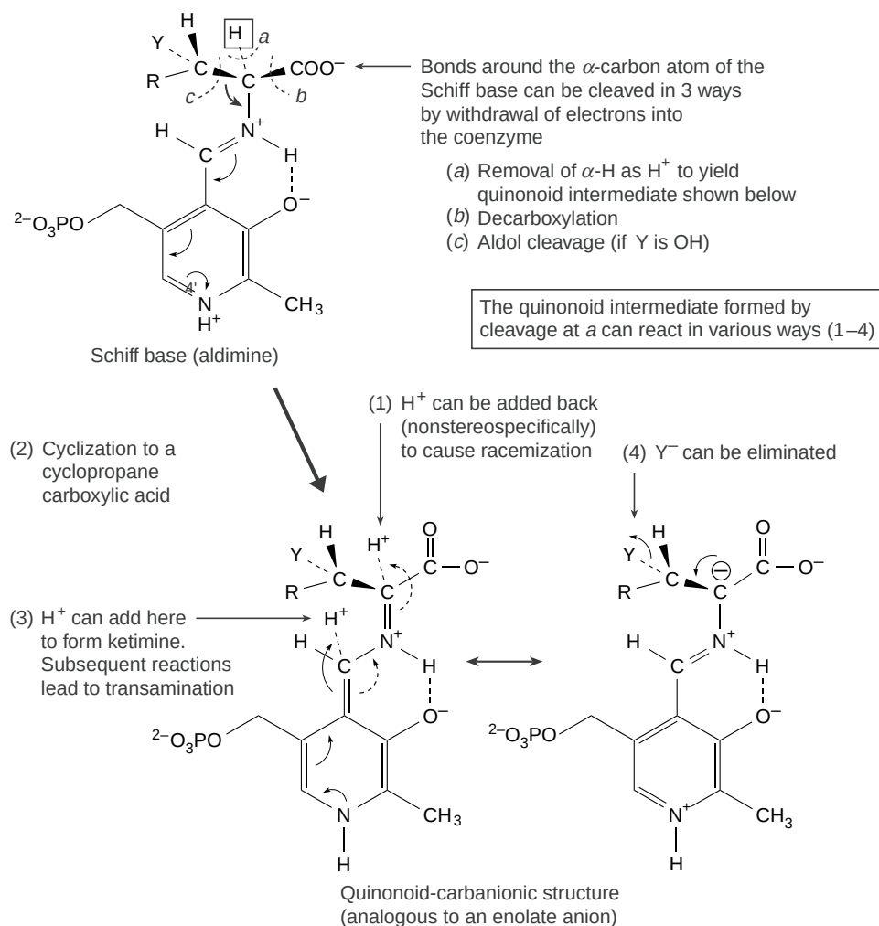
FIGURE 3 The action of pyridoxal phosphate in initiating catalysis of numerous reactions of α-amino acids. Completion of the various reactions requires a large variety of different enzyme proteins.
