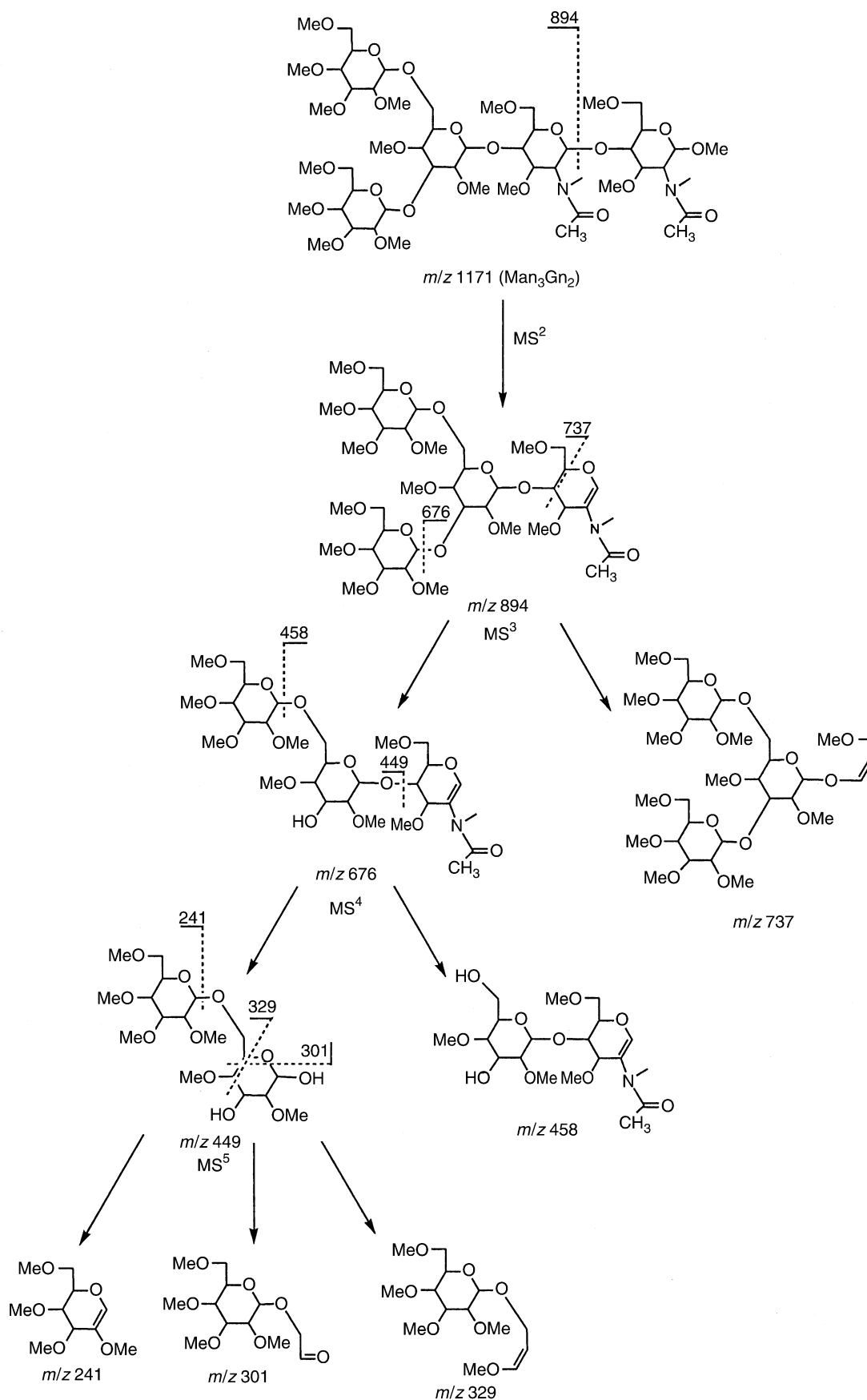
FIGURE 3 Use of \text{MS}^n to dissect a typical N-linked glycan. Selected CID pathways are shown through \text{MS}^5 .
