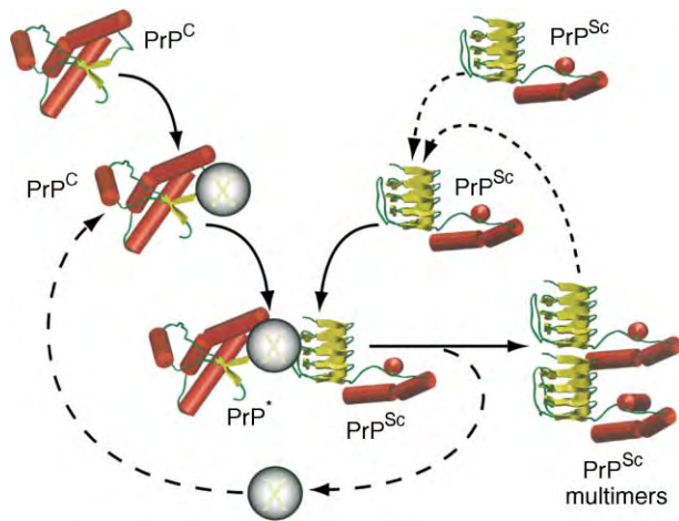
FIGURE 1 Exogenous or endogenous \text{PrP}^{\text{Sc}} initiates \text{PrP}^{\text{Sc}} synthesis by binding to a \text{PrP}^{\text{C}}/\text{X} complex. Facilitated by protein X and directed by the \text{PrP}^{\text{Sc}} template, \text{PrP}^{\text{C}} changes conformation and forms \text{PrP}^{\text{Sc}} . When \text{PrP}^{\text{Sc}} forms, the heteromultimeric complex dissociates, yielding recycled protein X and endogenous \text{PrP}^{\text{Sc}} . The newly generated \text{PrP}^{\text{Sc}} can then facilitate two replication cycles leading to an exponential rise in \text{PrP}^{\text{Sc}} formation.
