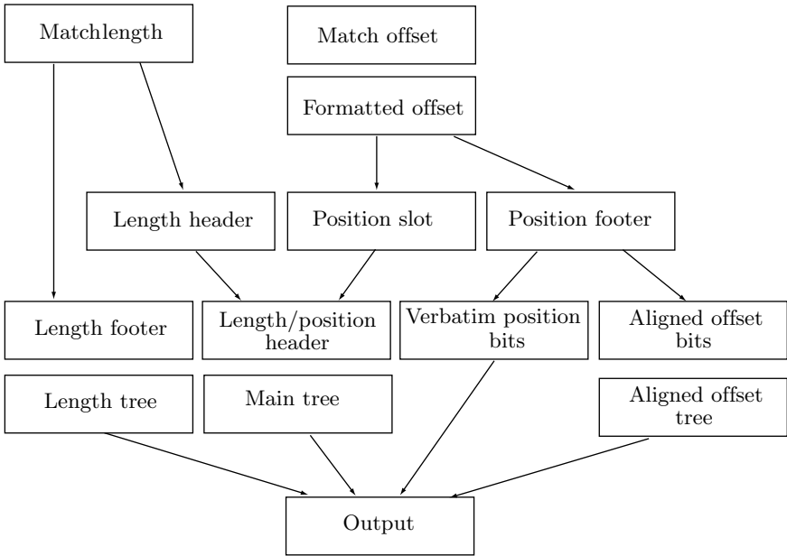
Figure 3.9: LZX Processing of Offsets and Lengths.
