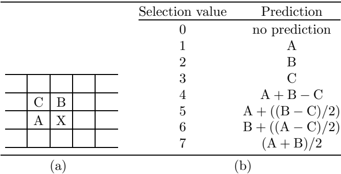
Figure 4.71: Pixel Prediction in the Lossless Mode.
