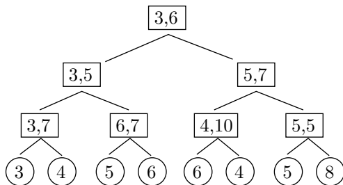
Figure 4.161: A Binary Tree for An 8-Pixel Image.
