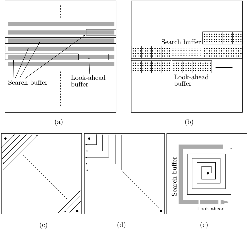
Figure 4.117: Block Matching (LZ77 for Images.)
