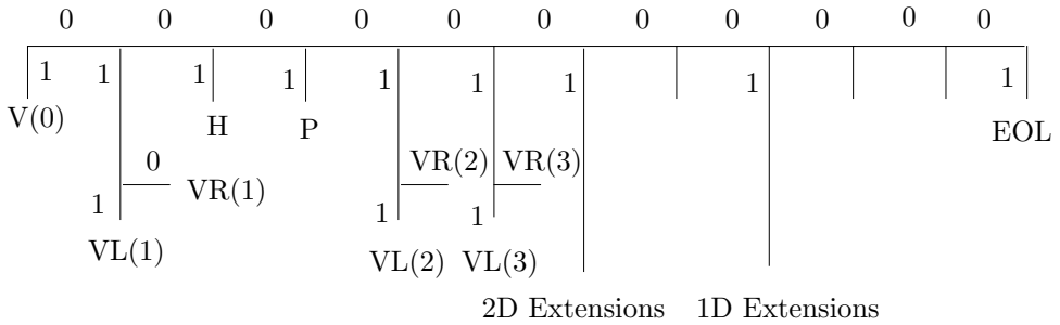
Figure 2.43: Tree of Group 3 Codes.
