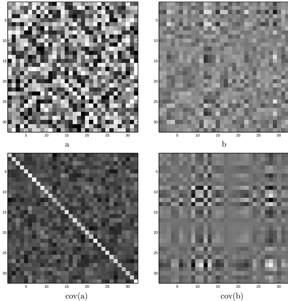
Figure 4.6: Covariance Matrices of Correlated and Decorrelated Values.
