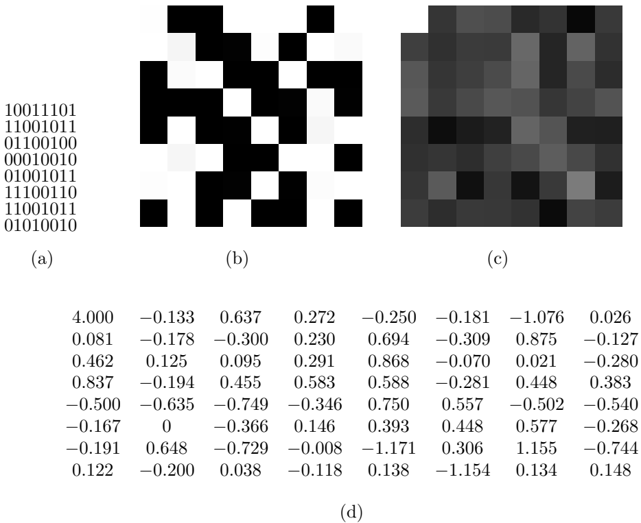
Figure 4.44: An Example of the DCT in Two Dimensions.
