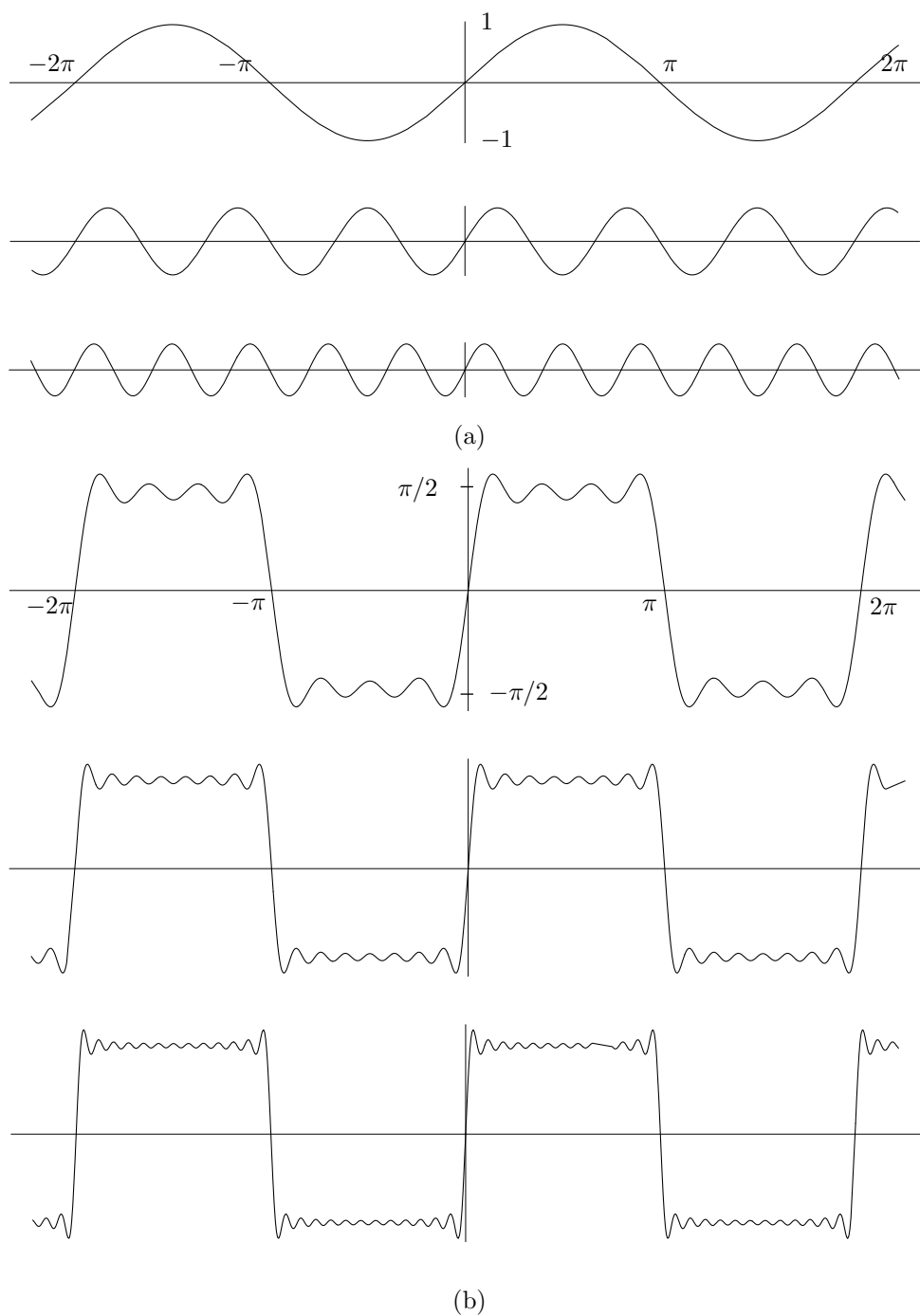
Figure 5.5: The First Three Terms and Three Partial Sums.
