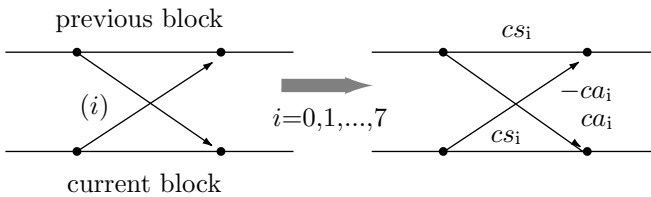
Figure 7.42: Layer III Aliasing Reduction Butterfly.
