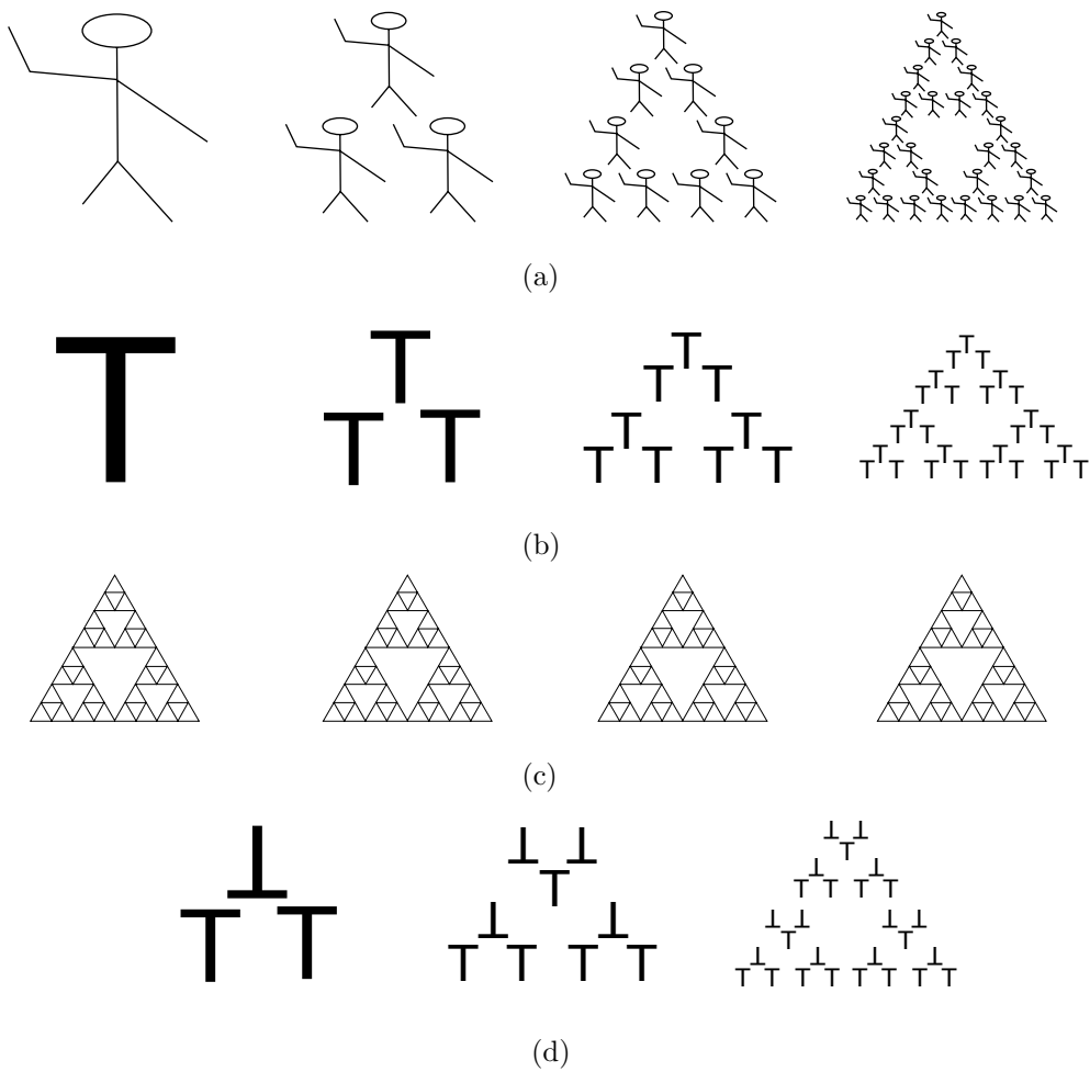
Figure 4.187: Creating the Sierpiński Gasket.
