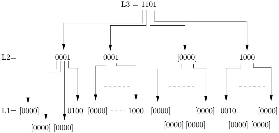
Figure 8.21: Reconstructing L_1 from L_3 .
