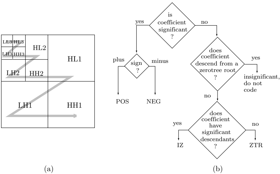
Figure 5.64: (a) Scanning a Zerotree. (b) Classifying a Coefficient.
