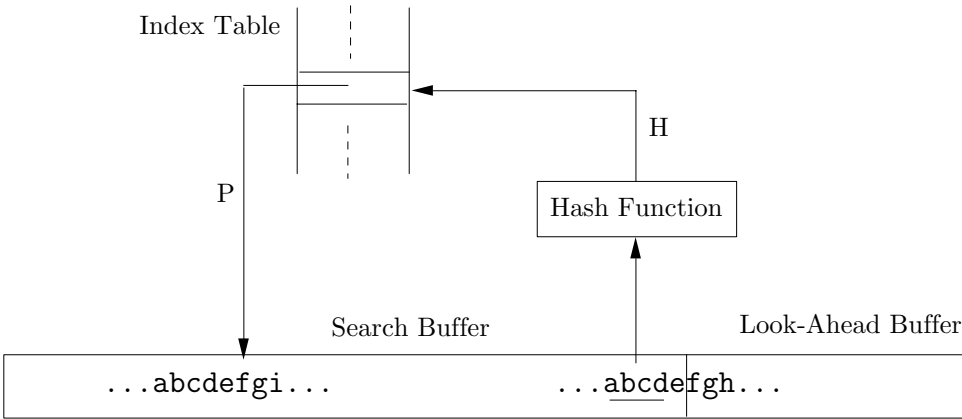
Figure 3.27: The Principle of LZP: Part I.
