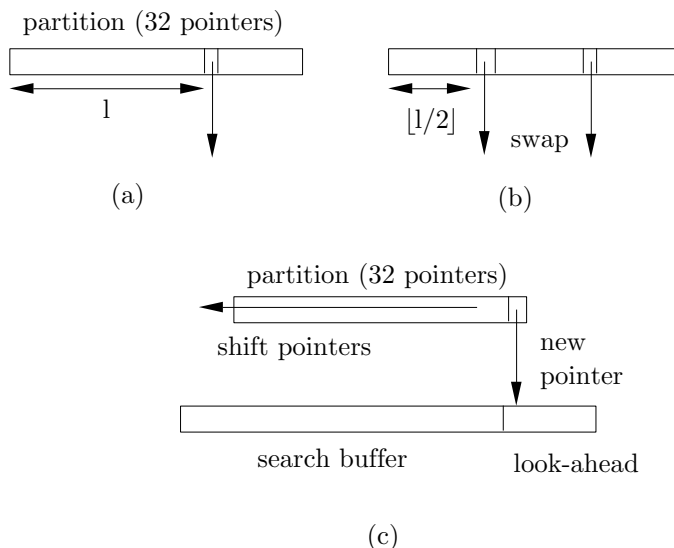
Figure 3.18: Updating an LZW4 Partition.
