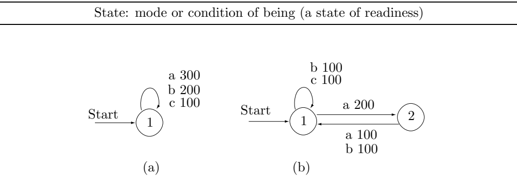
Figure 8.36: Finite-State Models for Data Compression.
