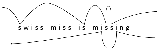
Figure 8.6: Context Searching for Order-1.
