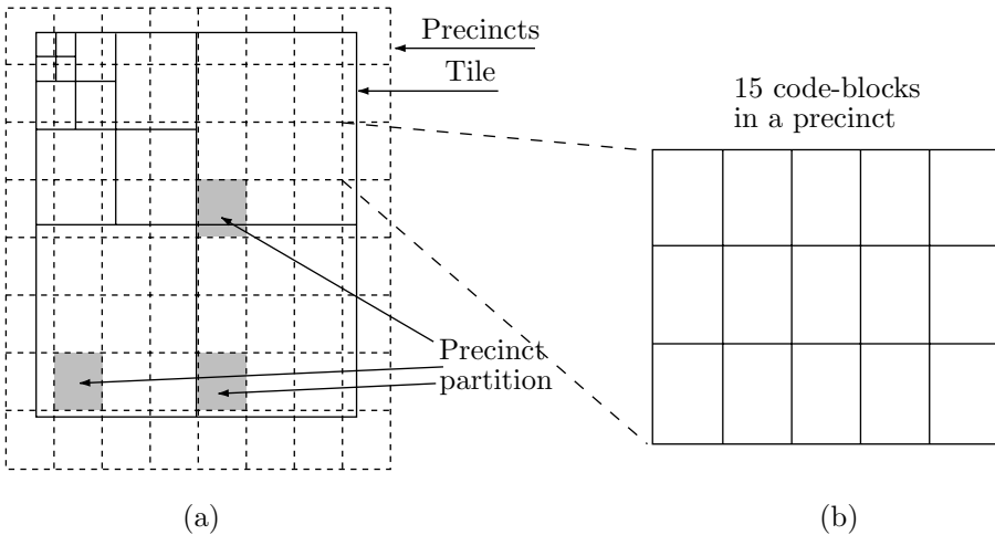
Figure 5.75: Subbands, Precincts, and Code-Blocks.
