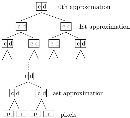
Figure 4.160: Successive Approximation in a Binary Tree.
