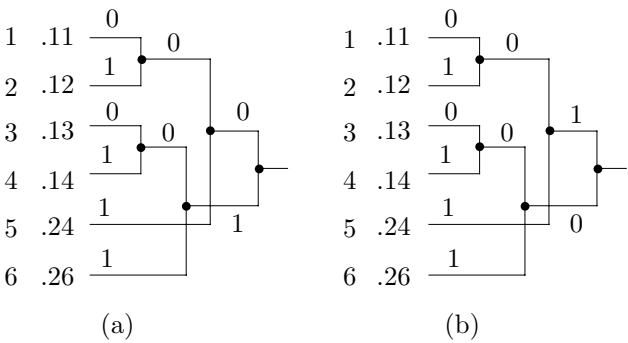
Figure 2.23: Two Huffman Code-Trees.
