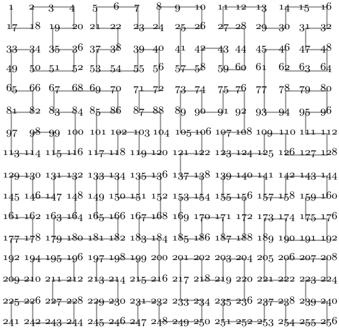
Figure 4.168: Hilbert Scan of 16×16 Blocks.
