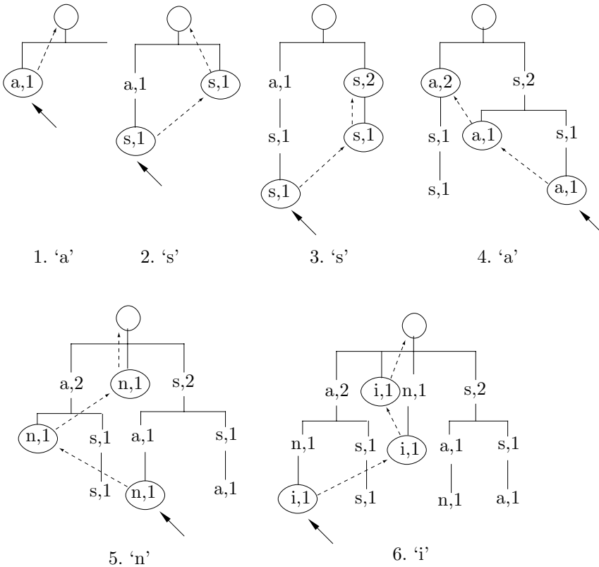
Figure 2.74: Part I. First Six Tries of "assanissimassa".
