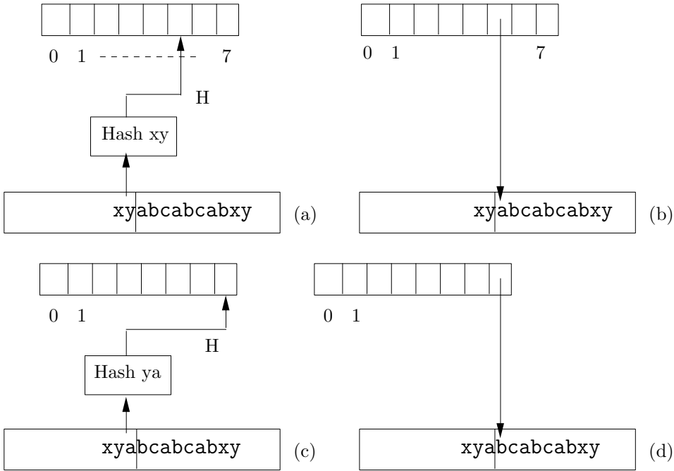
Figure 3.28: LZW Compression of “xyabcbcabxy”: Part I.
