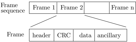
Figure 7.35: Format of Compressed Output.
