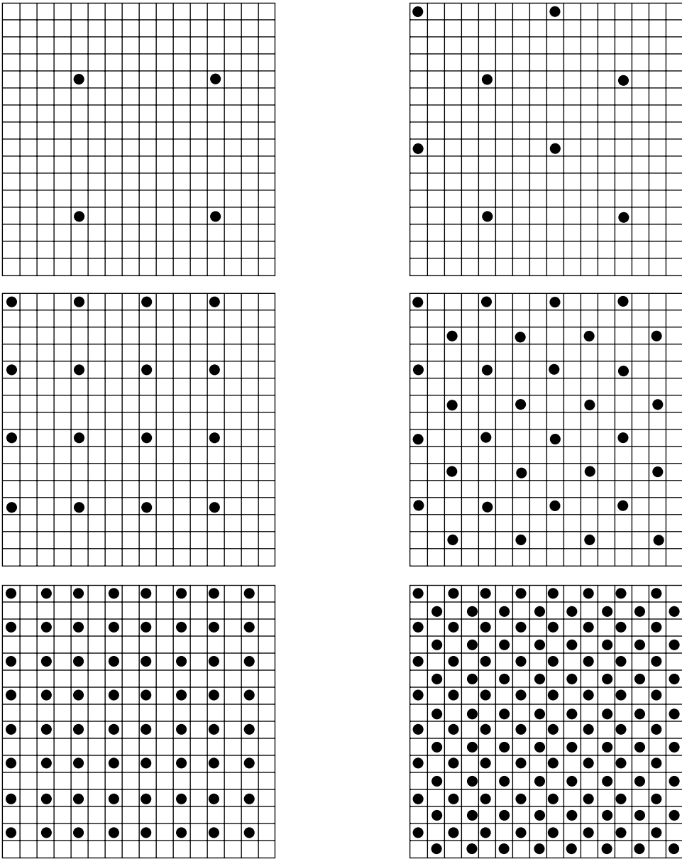
Figure 4.129: Some Levels of a 16 \times 16 Image.
