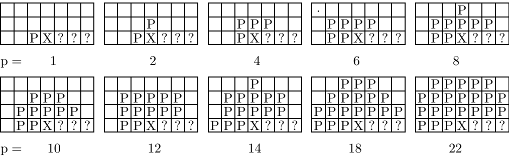
Figure 4.121: Context Pixel Patterns.
