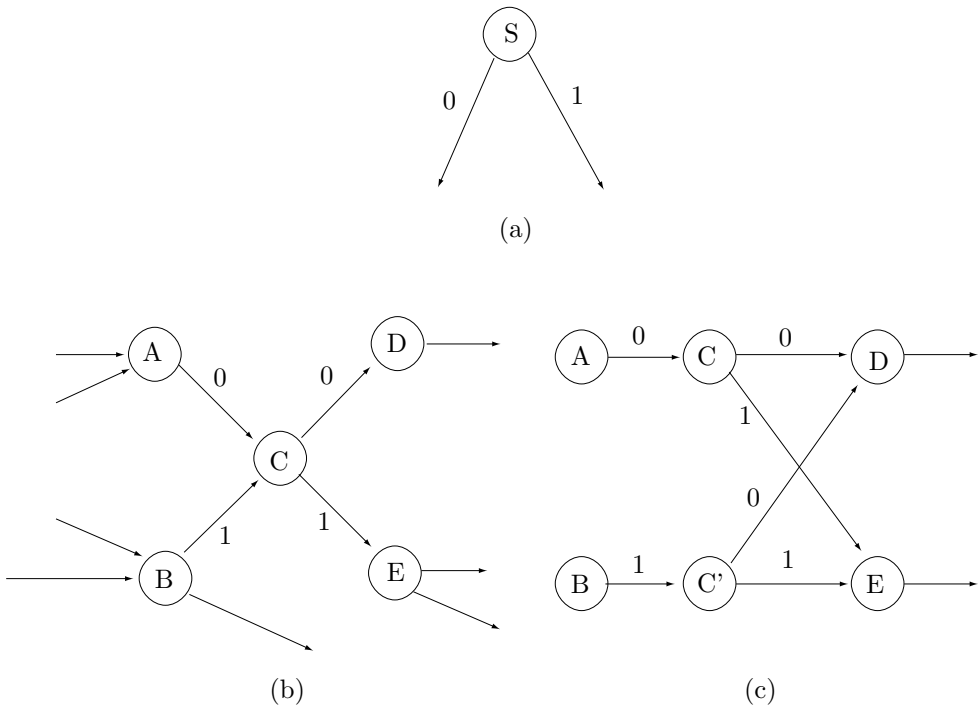
Figure 8.37: The Principles of DMC.
