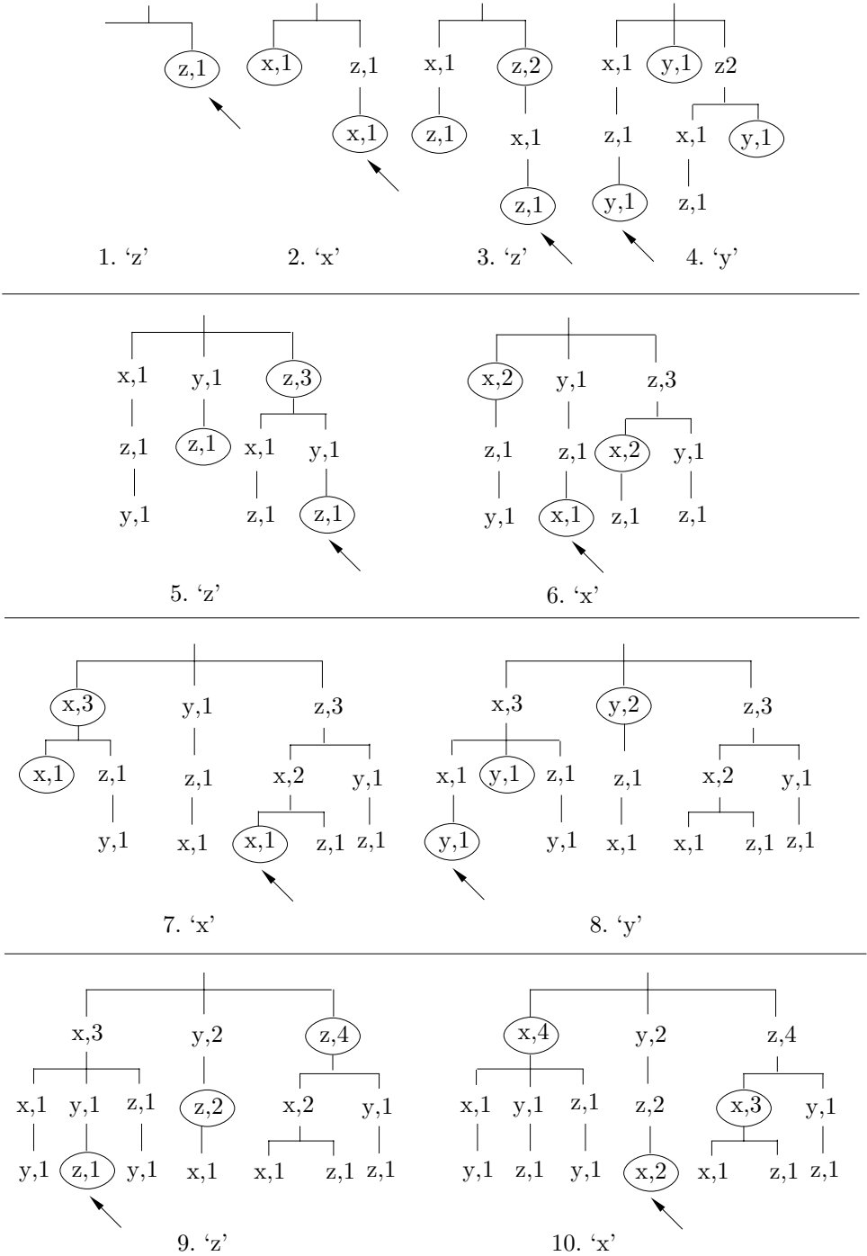
Figure 2.73: Ten Tries of "zxzyzxxxyzx".
