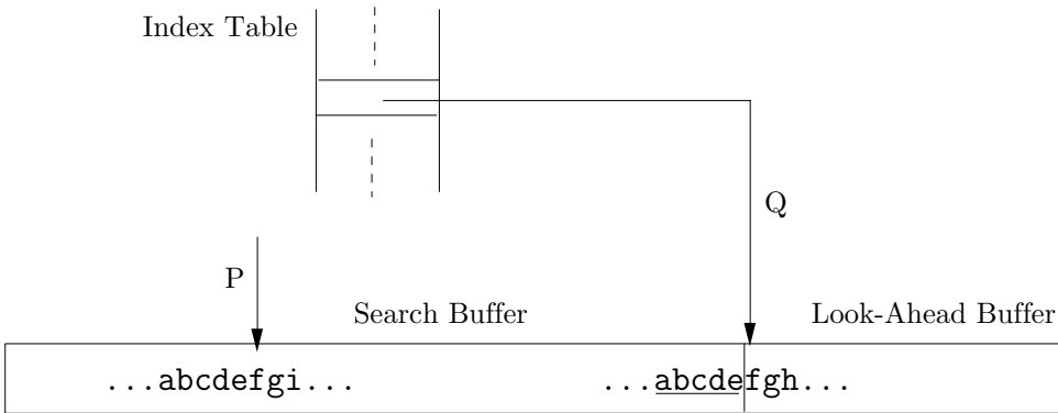
Figure 3.27: The Principle of LZP: Part II.
