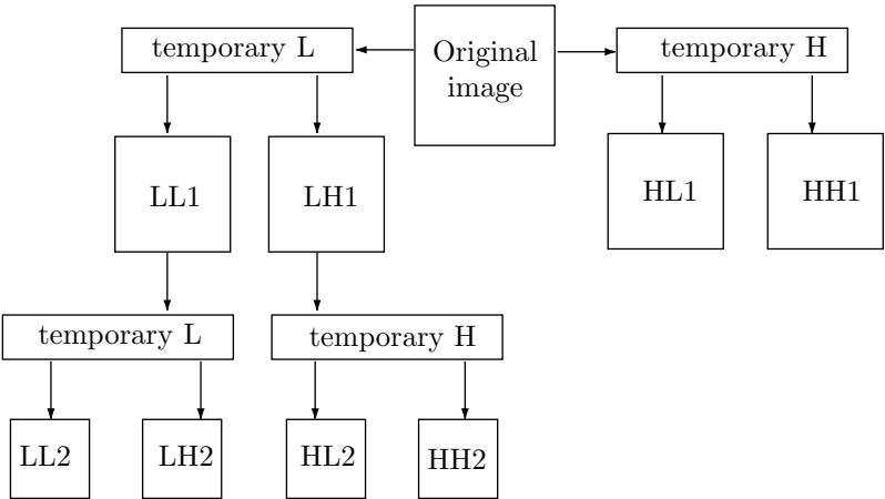
Figure 5.43: Pyramid Wavelet Decomposition.
