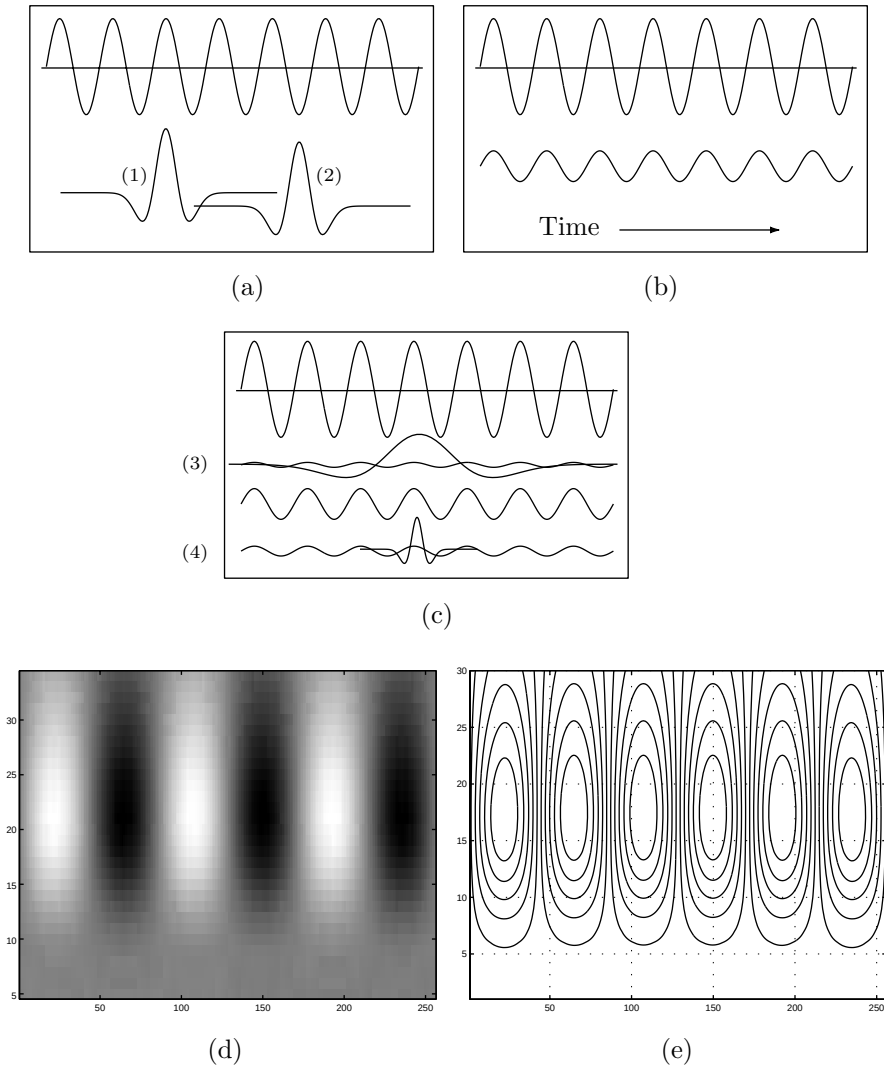
Figure 5.9: The Continuous Wavelet Transform of a Pure Sine Wave.
