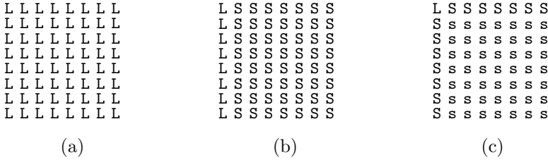
Figure 4.46: The Two-Dimensional DCT as a Double Rotation.
