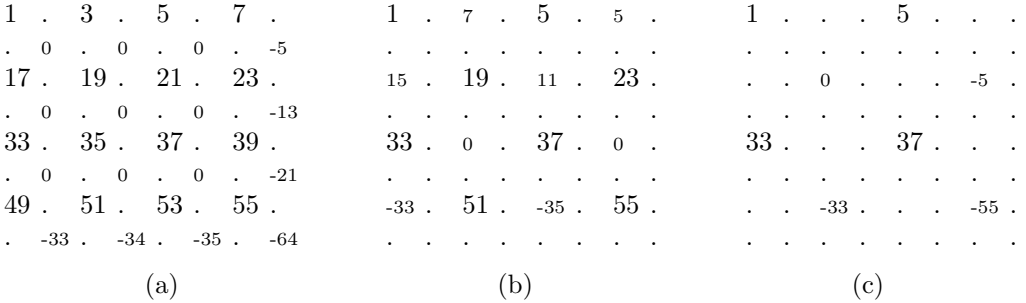
Figure 4.150: (a) Bands L_2 and H_2 . (b) Bands L_3 and H_3 . (c) Bands L_4 and H_4 .
