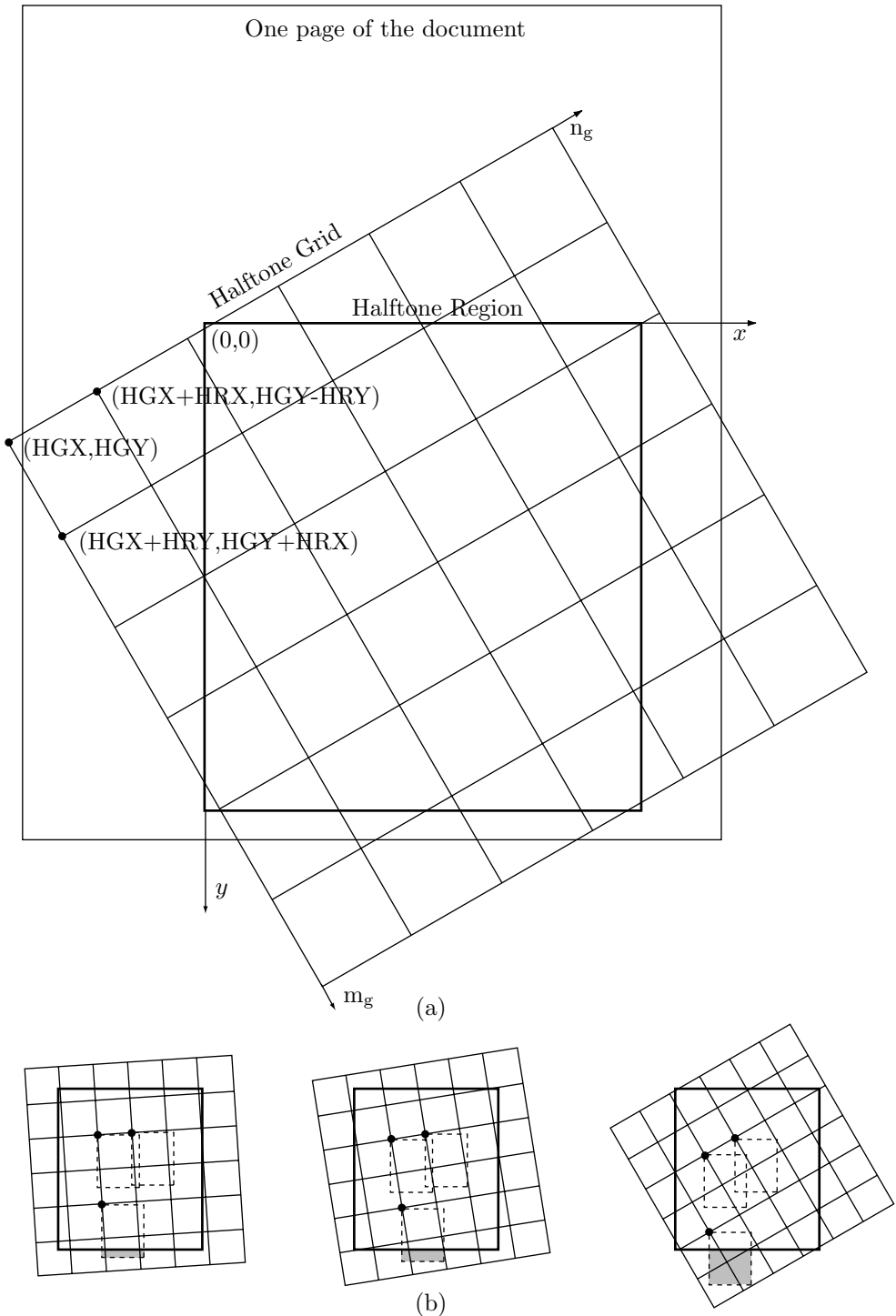
Figure 4.106: Halftone Grids and Regions.
