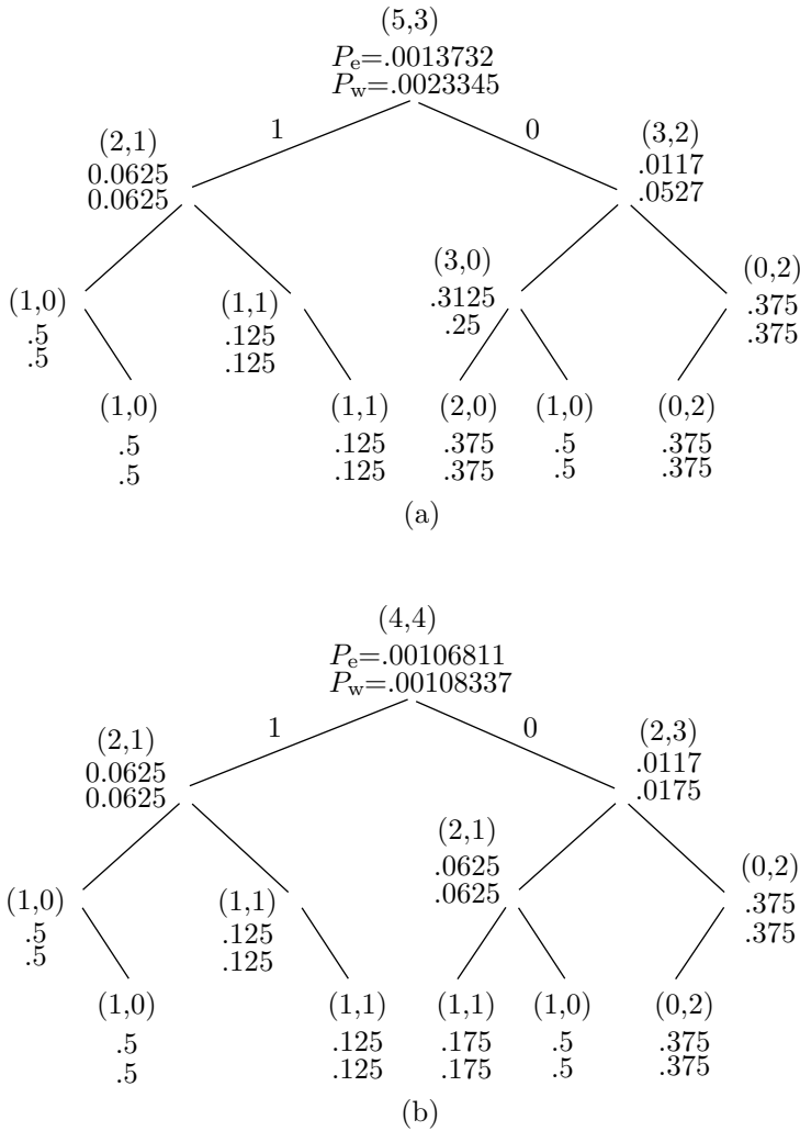
Figure 2.82: Context Trees for b_t = 0, 1 .
