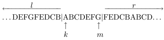
Figure 5.72: Extending a Row of Pixels.
