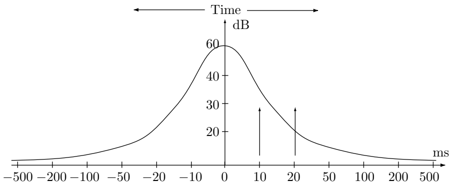
Figure 7.6: Threshold and Masking of Sound.
