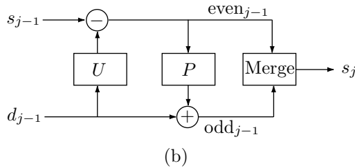
Figure 5.48: The Lifting Scheme. (a) Forward Transform. (b) Reverse Transform.
