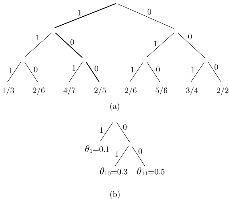
Figure 2.80: Two Suffix Trees.
