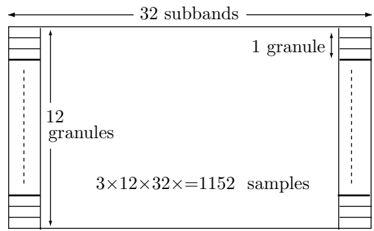
Figure 7.36: Organization of Layer II Subband Signals.
