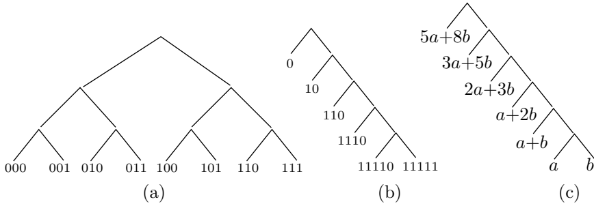
Figure 2.26: Shortest and Tallest Huffman Trees.
