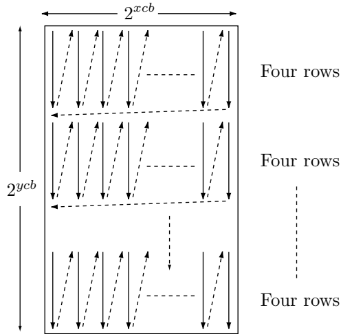
Figure 5.76: Stripes in a Code-Block.
