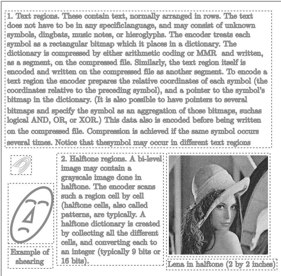
Figure 4.99: Typical JBIG2 Regions.
