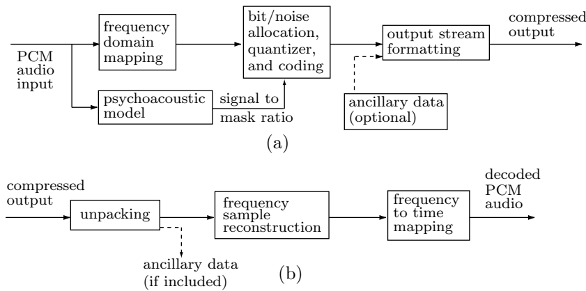
Figure 7.26: MPEG Audio: (a) Encoder and (b) Decoder.
