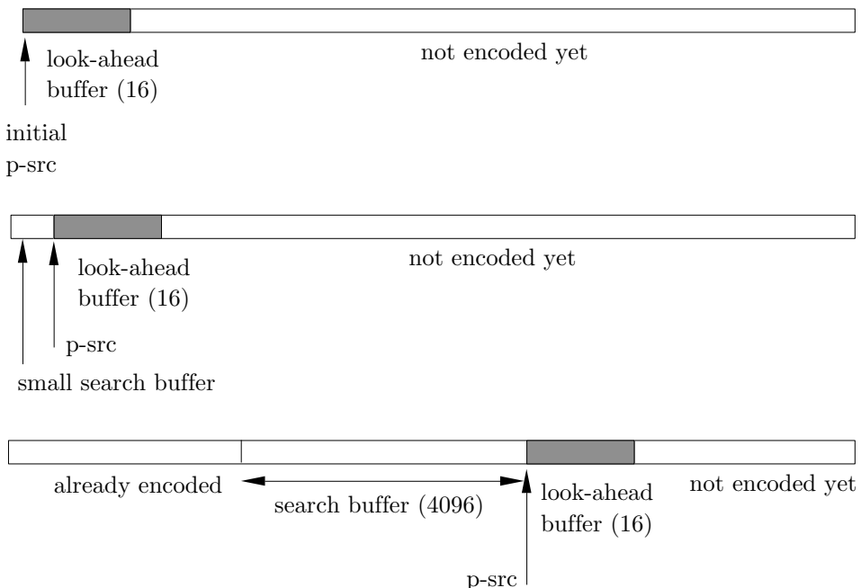
Figure 3.13: Sliding the LZRW1 Search- and Look-Ahead Buffers.
