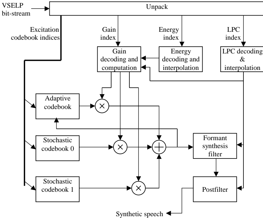
Figure 13.3 Block diagram of the IS54 VSELP decoder.
