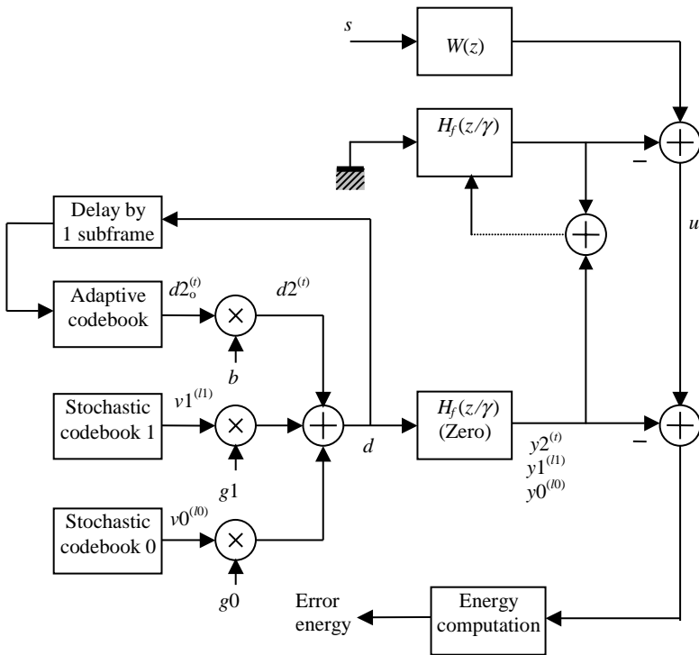
Figure 13.1 Signals involved in the IS54 encoder.
