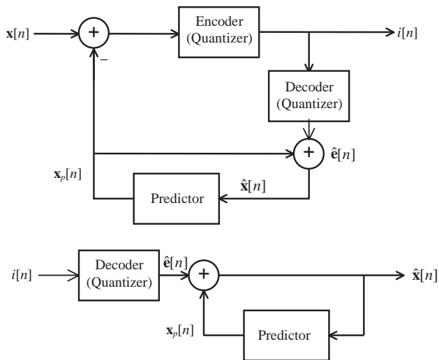
Figure 7.19 PVQ encoder (top) and decoder (bottom).
