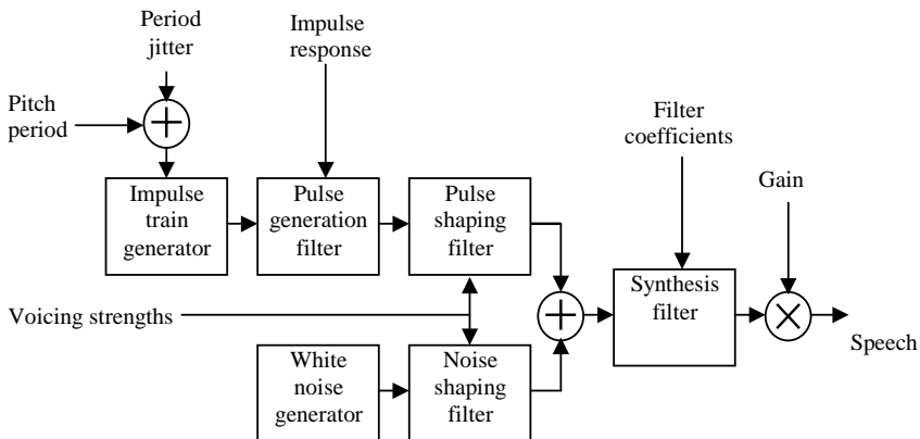
Figure 17.1 The MELP model of speech production.
