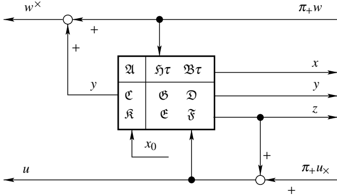
Figure 8.2 Right coprime factor
