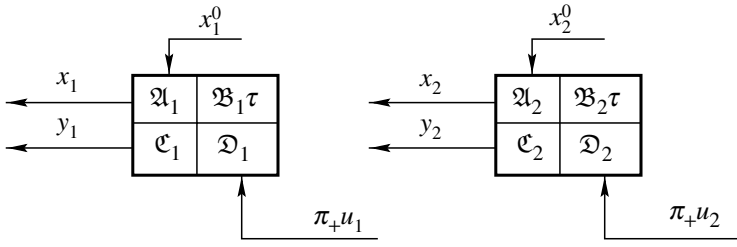
Figure 2.3 Cross-product (the union of two independent systems)
