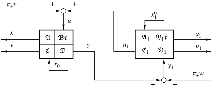
Figure 8.5 Dynamic stabilization
