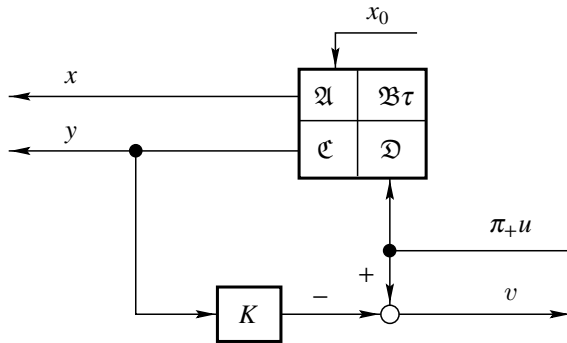
Figure 7.16 Original system with one extra output
