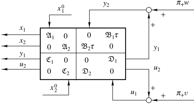
Figure 7.12 Dynamic feedback in block form
