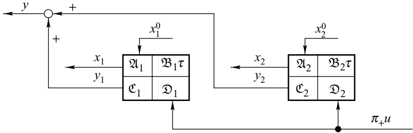
Figure 2.9 Parallel connection
