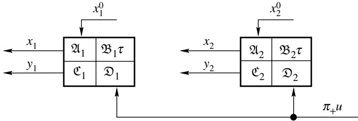
Figure 2.7 T-junction
