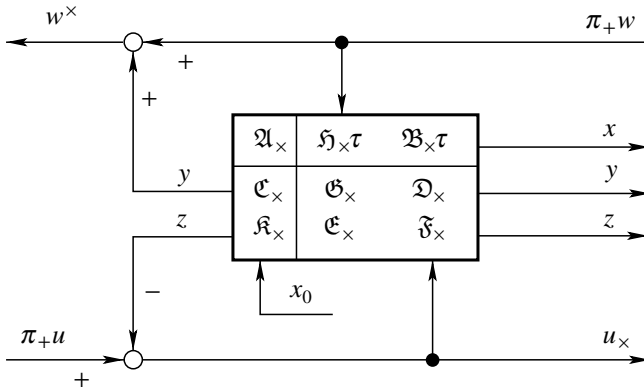
Figure 8.4 Cancellation of state feedback
