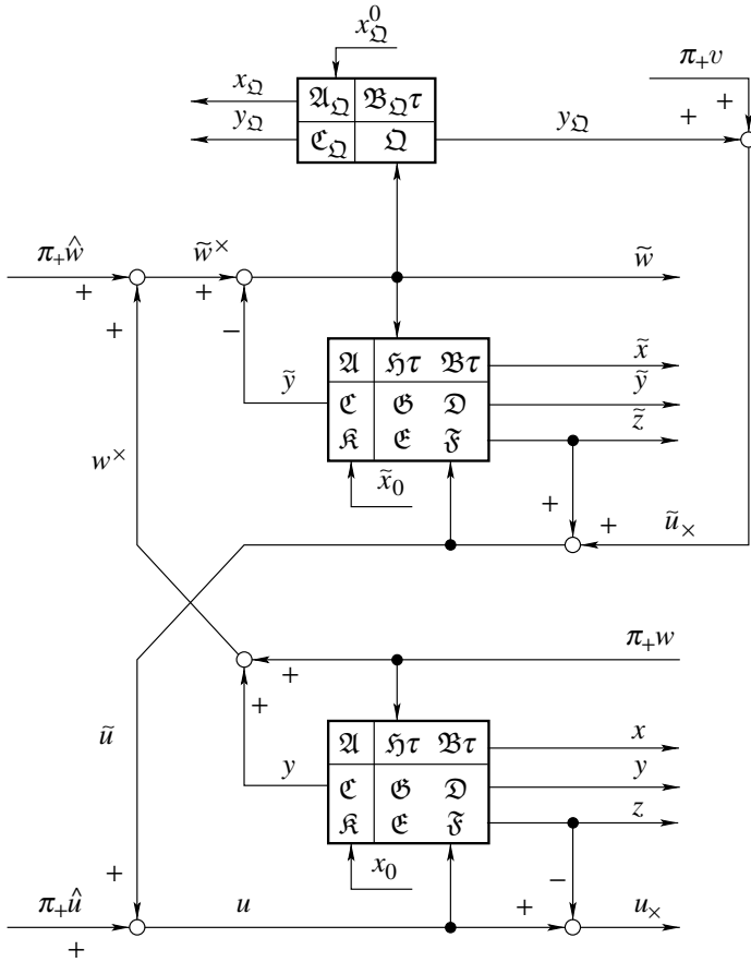
Figure 8.10 Youla parametrization
