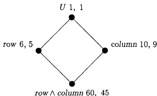
Fig. 2. Hasse diagram for the plot structure in (1)
