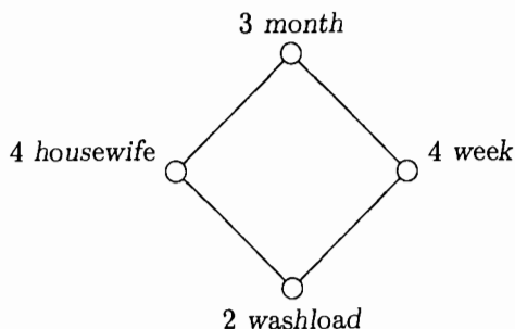
Fig. 8. Poset of pre-factors in the simple orthogonal block structure (3)
