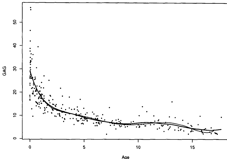
Fig. 1. Two smooth curves fitted to the concentration of the chemical GAG in the urine of 314 children aged 0–18 years.
