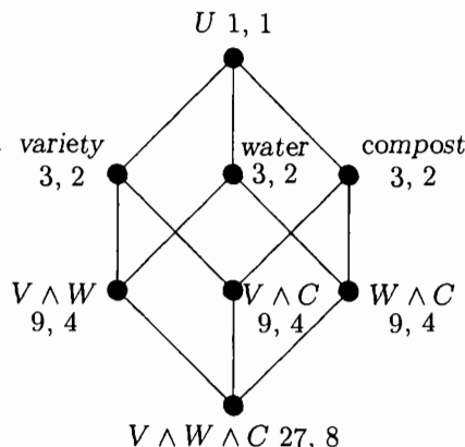
Fig. 5. Hasse diagram for the treatment structure in (4)
