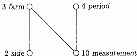
Fig. 10. A poset that cannot be obtained from iterated crossing and nesting
