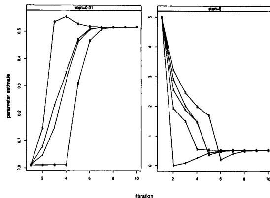
Fig. 1. Lamb weight data: estimates for sire variance component for 5 algorithms: 1=standard AI; 2=EM/AI; 3=PXEM/AI; 4=local EM/AI; 5=local PXEM/AI. First 10 iterations only. (a) start values \sigma_s^2 = .01 , \sigma_e^2 = 1 and (b) start values \sigma_s^2 = 5 , \sigma_e^2 = 1
