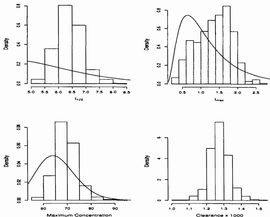
Fig. 3. Histogram representations of posterior distributions for the log-linear inverse polynomial model; solid curves denote the lognormal prior distributions.
