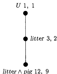
Fig. 3. Hasse diagram for the plot structure in (2)
