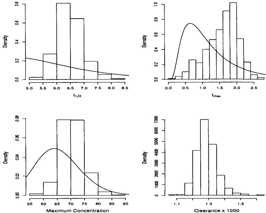
Fig. 2. Histogram representations of posterior distributions for the compartmental model; solid curves denote the lognormal prior distributions.
