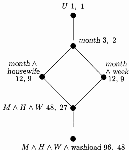
Fig. 4. Hasse diagram for the plot structure in (3)
