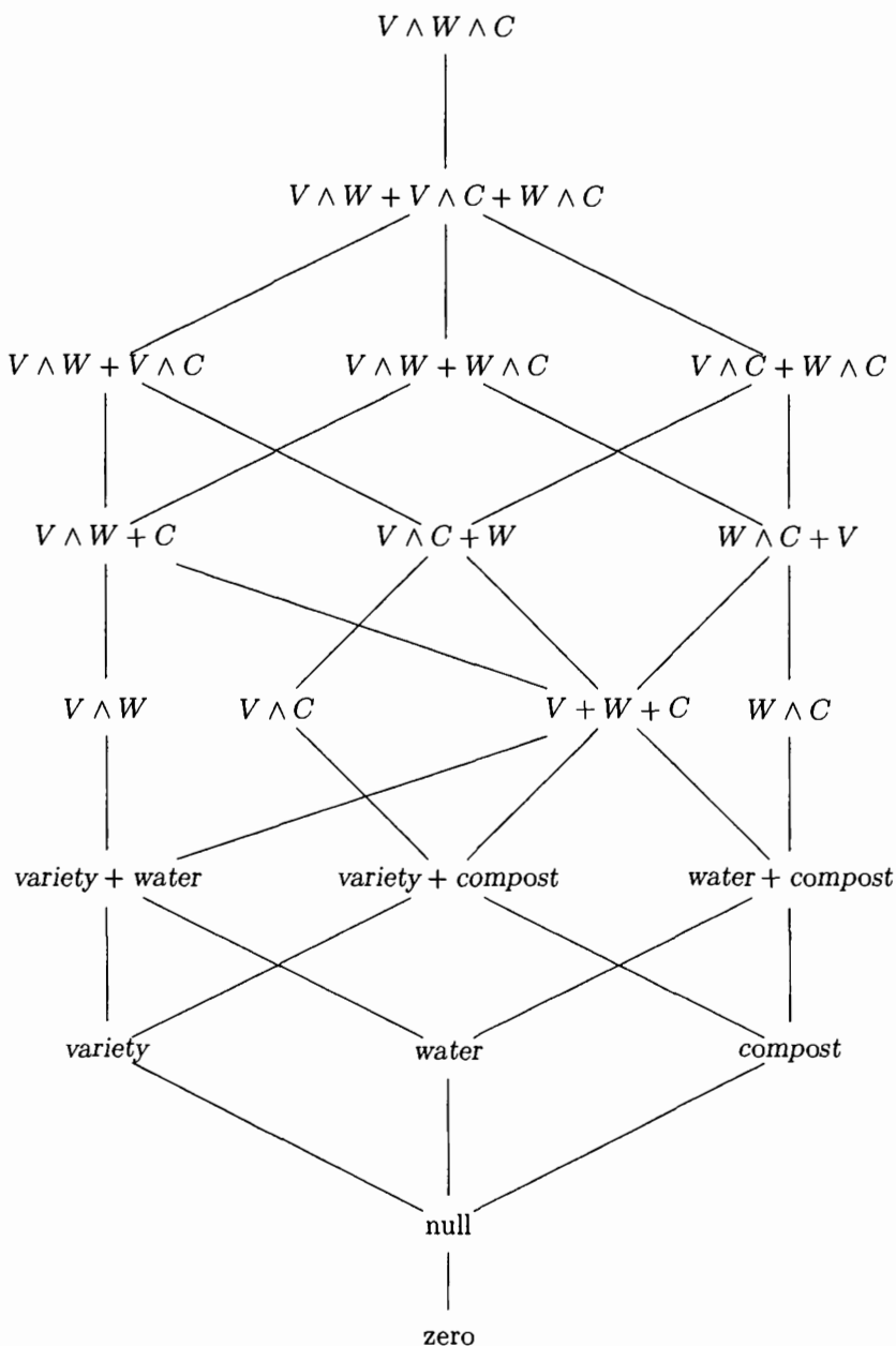
Fig. 14. Family of models for three treatment factors in Figure 9
