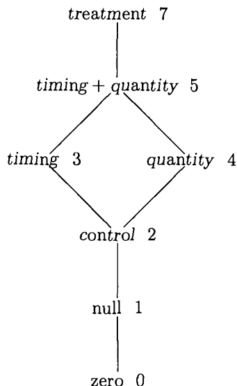
Fig. 13. Model diagram for the models listed in Figure 12
