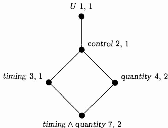
Fig. 11. The Tjur structure from Figure 1
