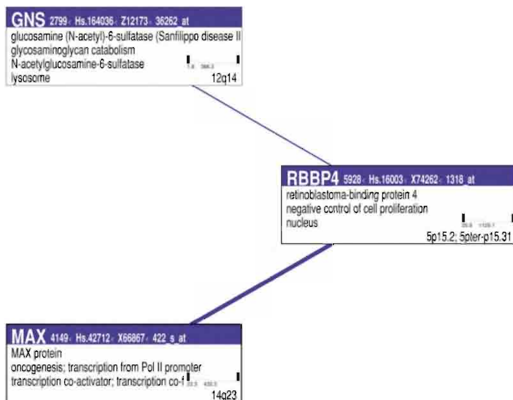
Figure 4.10: Sample relevance network. One of 78 networks formed by aggregating mouse samples from six different experiments. Threshold r^2 was set to .99, meaning that the "thinnest" line seen represented an r^2 of .99. The legend for this type of diagram is shown in figure 4.11. The hypothesis generated here is that RBBP4 expression correlates with GNS and MAX gene expression. The miniature histograms for each gene show no "spiking" in the expression measurements (see section 4.5.2). Each of these genes appears at a different chromosomal location. By including information from LocusLink (see section 5.5.1) and Gene Ontology (see section 5.1.1), we see that RBBP4 is known to control cell proliferation, and MAX is involved in oncogenesis.
