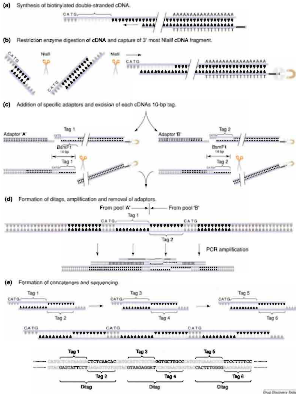
Figure 7.5: The Serial Analysis of Gene Expression. (Derived from Madden et al. [124].
