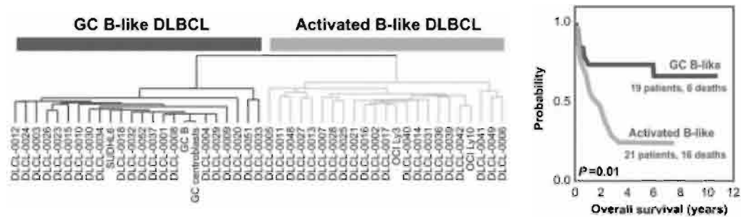
Figure 4.13: Subcategories of B-cell lymphoma determined by microarrays correspond clinically to duration of survival. On the left is a dendrogram constructed across the samples of B-cell lymphoma, using an unsupervised technique. The top branch essentially defines an even split between the categories GC B-like DLBCL and Activated B-like DLBCL, but this distinction was never before made clinically. On the right are Kaplan-Meier survival curves of the patients from whom the samples were obtained. Patients whose cancer matched the Activated B-like DLBCL gene expression profile had a significantly worse prognosis. (From Alizadeh et al. [3].)
