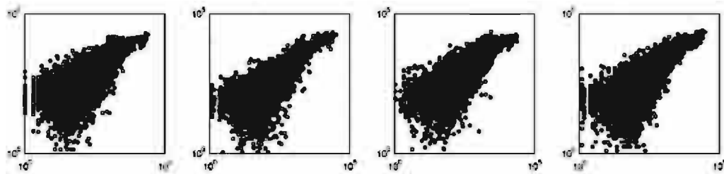
Figure 3.9: Expression measurements made in duplicate from the same RNA samples do not correlate well all the time. RNA samples from four human samples were placed on duplicate oligochips and the expression of 35,714 ESTs was measured. Each point represents an EST. The duplicate expression measurements are plotted here on a log-log scale (base 10). r = .69, .73, .73, .69 . (From Butte et al. [40].)
