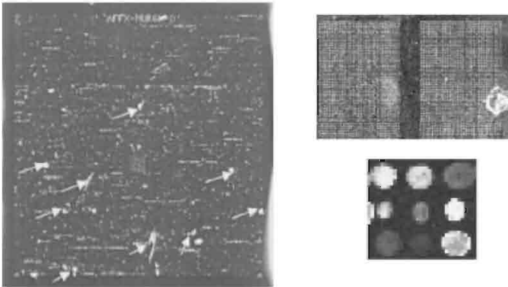
Figure 3.20: Problems in images acquired from microarrays. On the left: a contaminated D array from the Murine 6500 Affymetrix GeneChip set. Several particles are highlighted by arrows and are thought to be torn pieces of the chip cartridge septum, potentially resulting from repeatedly pipetting the target into the array [156]. On the right top: local changes in intensity due to contaminants and scratches. (Derived from http://www.mediacy.com/arraypro.htm .) Right bottom: high magnification of a scanned image of a spotted microarray. Note the different sizes and shapes of the spots [199].
