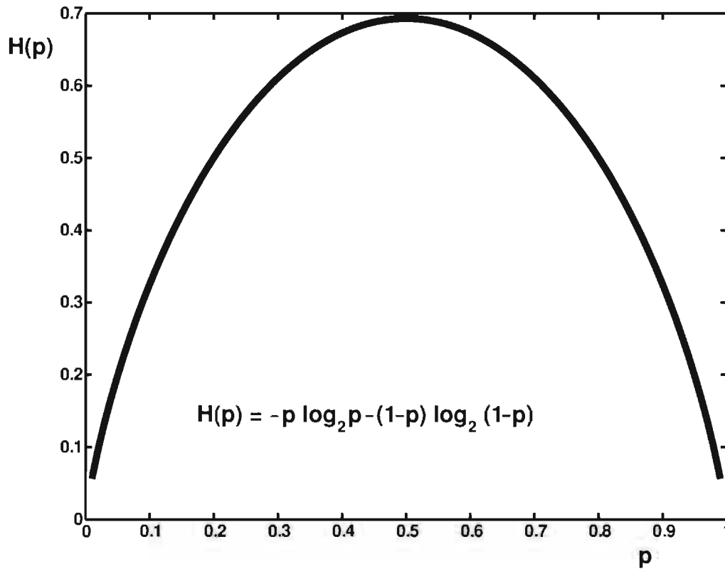
Figure 3.24: Entropy plot
