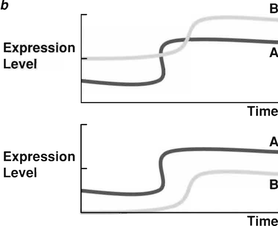
Figure 3.26: Dynamic relationships between genes. (a) The expressed product of Gene A binds an enhancer region that increases transcription of Gene B. (b) Gene B's initial expression level before being affected by Gene A can vary throughout the experiment. As a result, measuring the correlation between the absolute levels of Genes A and B will not reveal the underlying enhancement relationship between the two. Instead, this can only be done by analyzing the expression dynamics—the change in expression level of Gene B in relation to the expression level of Gene A. (Derived from Reis et al. [150].)
