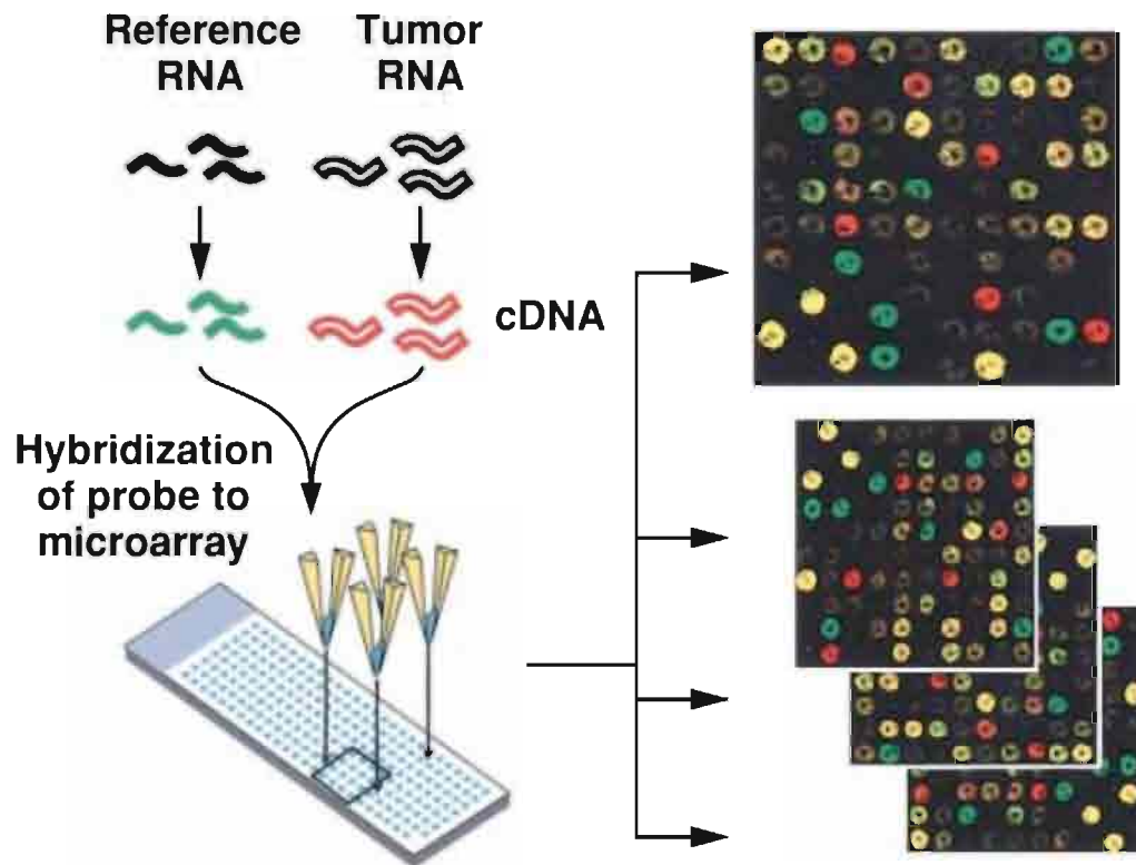
Figure 3.2: Robotically spotted microarray hybridized to two samples, each stained with two colored dyes. An overview of procedures for preparing and analyzing cDNA microarrays and tumor tissue. Reference RNA and tumor RNA are labeled by reverse transcription with different fluorescent dyes (green for the reference cells and red for the tumor cells) and hybridized to a cDNA microarray containing robotically printed cDNA clones. The slides are scanned with a confocal laser scanning microscope, and color images are generated for each hybridization with RNA from the tumor and reference cells. Genes upregulated in the tumors appear red, whereas those with decreased expression appear green. Genes with similar levels of expression in the two samples appear yellow. Genes of interest are selected on the basis of the differences in the level of expression by known tumor classes (e.g., BRCA1 mutation-positive and BRCA2 mutation-positive). Bioinformatics analysis determines whether these differences in gene expression profiles are greater than would be expected by chance. (Derived from Hedenfalk et al. [90].)
