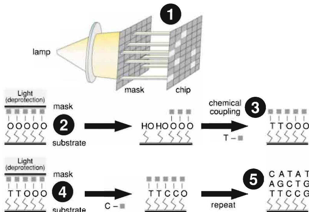
Figure 3.3: The photolithographic construction of microarrays. Synthesized high-density oligonucleotide microarray manufacturing with photolithography. Using selective masks, photolabile protecting groups are light-activated for DNA synthesis (1, 2); photoprotected DNA bases are added and coupled to the intended coordinates (3). This cycle is repeated (4) with the appropriate masks to allow for controlled parallel synthesis of oligonucleotide chains in all coordinates on the array (5). (Derived from Lipshutz et al. [121].)
