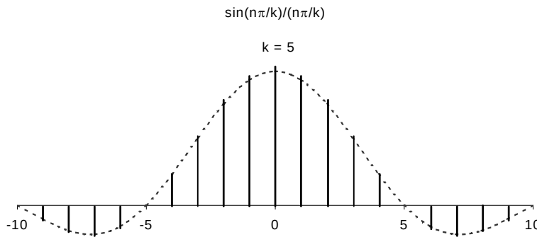
Figure 6.27. Line spectrum of (6.109) for k = 5
