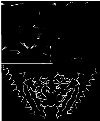
5.2 Al-atom contact examples from the structure of the protein. (a) shows a protein structure with a highlighted region. (b) shows a close-up of the highlighted region. (c) shows a network diagram of the protein structure, with nodes representing atoms and edges representing contacts. The network is highly interconnected, with a central cluster of nodes and many peripheral nodes connected to it.
