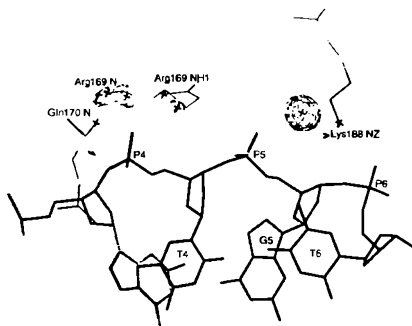
Figure 10.6. A view of the three residues in the consensus region for the high resolution CAP-DNA CC complex (Parkinson et al., 1996b). The predicted phosphate hydration is drawn as pseudoelectron density in cyan, the interacting protein residues are shown in dark brown, and the phosphate groups are red. The protein atoms that contact the DNA shown as blue crosses. The predicted sites are the red crosses. Reprinted from (Woda et al., 1998) with permission from the Biophysical Society. Figure also appears in Color Figure section.
