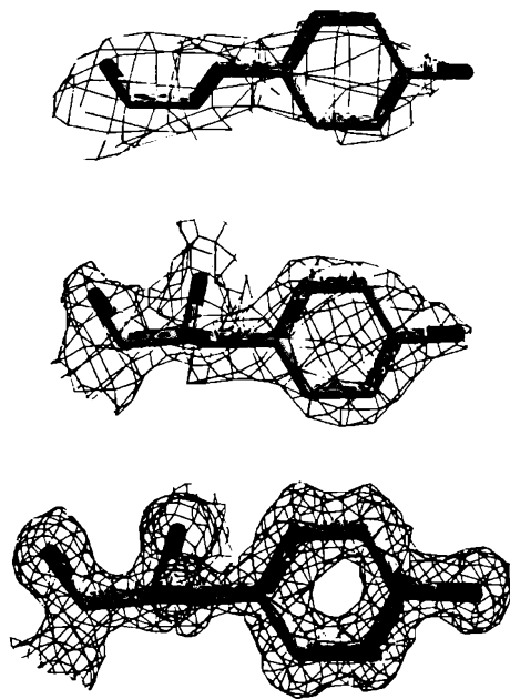
Figure 14.5. The effect of resolution on the quality of the electron density. The three plots show the electron density, as the wire-frame cage, surrounding a single tyrosine residue. The residue is Tyr100 from concanavalin A as found in three PDB structures solved at (a) 3.0 Å resolution (PDB code 1val), (b) 2.0 Å (1con), and (c) 1.2 Å (1jbc). At the lowest resolution the electron density is merely a shapeless blob, but as the resolution improves the individual atoms come into clear focus. The electron density maps were taken from the Uppsala Electron Density Server ( http://portray.bmc.uu.se/eds ) and rendered using BobScript (Lunouf, 1997) and Raster3D (McCrirt and Bacon, 1997).
