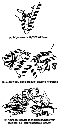
Figure 19.7. Prediction of function in earnest. Three structures solved in the absence of functional information. (a) Putative archaeal ATPase molecular switch; (b) putative bacterial hydrolase; (c) bifunctional archaeal inositol monophosphatase/fructose-1,6-bisphosphatase
