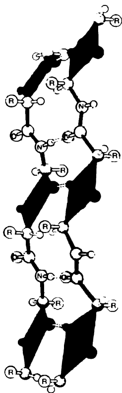
Figure 2.9. Diagram of an antiparallel \beta sheet using a ball-and-stick model. The bonds forming the backbone of the polypeptide are darkly shaded. The \beta sheet is stabilized by hydrogen bonds (shown here as dashed lines) formed between the carbonyl oxygen of a residue on one strand and the amide proton of a residue on the adjacent strand. Note that this arrangement produces a sheet that is pleated, with the residue side chains alternating positions on opposite sides of the sheet. From R. E. Dickerson and I. Geis. Hemoglobin: Structure, Function, Evolution, and Pathology . Menlo Park, CA: The Benjamin/Cummings Publishing Company, 1983. Used with permission from Geis Archives.
