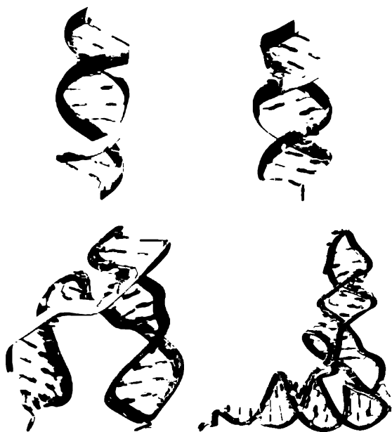
Figure 3.13. Examples of RNA. (a) RNA duplex with mismatches (GGACUUCGGUCC) (Holbrook et al., 1991). (b) A RNA duplex (Dock-Bregeon et al., 1989). (c) Hammerhead ribozyme (Fley, Faherty, and McKay, 1994). (d) tRNA (Sussman et al., 1978). Backbone is colored blue (for structures with one strand) and blue and gold (for structures with two strands). Bases are colored green for guanine, yellow for cytosine, red for adenine, and cyan for uracil. Modified bases follow the same color scheme.
