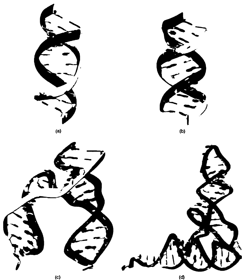
Figure 3.13. Examples of RNA. (a) RNA duplex with mismatches r(\text{GGACUUCGGUCC}) (Holbrook et al., 1991); (b) A-RNA duplex (Dock-Bregeon et al., 1989); (c) Hammerhead ribozyme (Pley, Flaherty, and McKay, 1994); (d) tRNA (Sussman et al., 1978). Figure also appears in Color Figure section.
