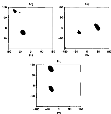
Figure 14.8. Differences in Ramachandran plots for (a) arginine, representing a fairly standard amino acid residue, (b) glycine which, due to its lack of a side chain, is able to reach the parts of the plot that other residue cannot reach, and (c) proline which, due to its restraints on the movement of the main chain, has a restricted range of \phi values. The darker regions correspond to the more densely populated regions as observed in a representative sample of protein structures.
