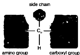
Figure 2.1. The structure of a prototypical amino acid. The chemical groups bound to the central alpha ( \alpha ) carbon are highlighted in gray. The R-group represents any of the possible 20 amino acid side chains.
