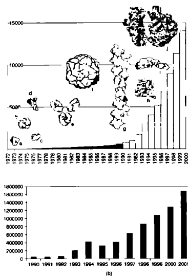
Figure 9.2 (A) Growth chart of the PDB showing the total number of structures available in the PDB archive per year and highlighting example structures from different time periods. a) myoglobin, b) hemoglobin, c) lysozyme, d) transfer RNA, e) antibodies, f) entire viruses, g) actin, h) the nucleosome, i) myosin, and j) 30S ribosomal subunits. Images were created by Dr. David Goodsell, who authors the PDB's Molecule of the Month series. Figure originally appeared in the International Union of Crystallography Newsletter (2001). Images, descriptions and the molecules, and links to related information can be found at http://www.rcsb.org/pdb/molecules/molecule.list.html . (B) Number of residues released in the PDB per year. Figure also appears in Color Figure section
