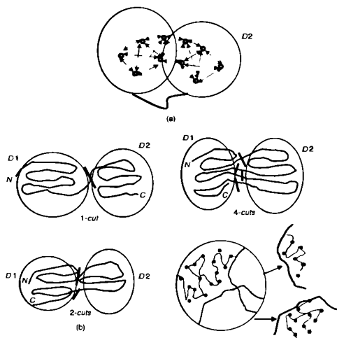
Figure 18.2. Illustration of the problem of parsing the protein 3D structure into structural domains. (a) The most common definition of structural domains, as groups of residues with a maximum number of contacts within each group and a minimum number of contacts between the groups. (b) Domains may be composed of one or more chain segments. Any domain-assignment procedure must therefore be able to cut the polypeptide chains as many times as necessary. When both domains are composed of contiguous chain segments (continuous domains), only one chain cut (1-cut) is required. When one domain is continuous and the other discontinuous, a situation that may arise as a result of gene insertion, then the chain has to be cut in two places (2-cuts). When both domains are discontinuous, additional chain cuts may be required. In the example shown, the chain is cut in four places (4-cuts), and thus the domain on the left-hand side contains three chain segments, whereas that on the right contains two chain segments. (c) This drawing shows two solutions to the problem of partitioning the protein 3D structure into substructures. To partition the 3D structure into domains, many such solutions need to be examined in order to single out the one that satisfies the criterion given in (a). Figure also appears in Color Figure section.
