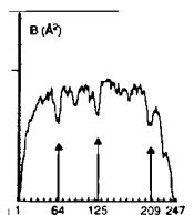
Figure 18.4. The interface area scan for Triose Phosphate Isomerase (TIM) computed as in Wodak and Janin (1981b). The area B in \text{\AA}^2 of the interface between residues 1 to i and i to N , with N being the last residue in the chain, is plotted against the position i of the cleavage point. Residue numbering is as in the original file for the atomic coordinates. The scan has been produced using a model of the protein, where each residue is represented by a single interaction center. The arrows shown in the plot indicate the minima of B in the scan. These occur at residue 64, 125, and 209. The minimum at residue 125 splits the TIM barrel into two halves, which correspond well with the proposals for the common half barrel ancestor (see text).
