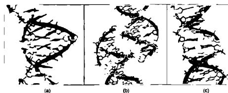
Figure 10.9. Examples of packing motifs in DNA duplexes in a B- and A-DNA. From left to right: (a) minor groove-minor groove interactions in BDJ042 (Leonard & Hunter, 1993); (b) major groove-backbone interactions in BDJ060 (Goodsell et al., 1995); (c) stacking interactions in BDJ025 (Grzeskowiak et al., 1991). The bases are colored green for guanine, yellow for cytosine, red for adenine, and blue for thymine. Reprinted from (Berman et al., 1996) with permission from Elsevier Science. Figure also appears in Color Figure section.
