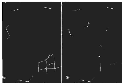
Figure 15.8 A test of alternative sequence possibilities: substituting Trp for Tyr at a buried position in the N-terminal domain of a repressor, using the 'remote update' function of the interactive MageProbe system. (a) One of the listed rotamer trials, with impossibly bad clashes both sides of the Trp ring. (b) The best of the exact rotamers, with only two minor overlap clashes, indicating that the Trp side chain can indeed fit without perturbing the structure significantly. Starting coordinates from MB Boerner and Paller, 1992. Figure as it appears for Prokin sector.
