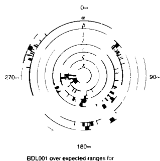
Figure 3.10 Conformational wheel (Schneider, Neidle, and Berman, 1997) showing the torsion angles for BDL001 (Drew et al. 1981). Black lines show actual values of torsion angles, cyan background their allowed range in the B-type DNA conformation (Schneider, Neidle, and Berman, 1997). The grey shades in the outer rings show the average value(s) of the torsions in dark grey flanked by values of one and two estimated standard deviations in lighter grey.
