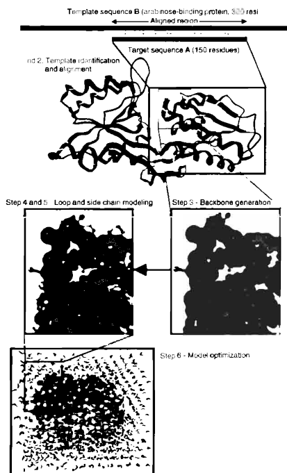
Figure 25.2 The steps to homology modeling. The fragment of the template (arabinose-binding protein) corresponding to the region aligned with the target sequence forms the basis of the model (including conserved side chains). Loops and missing side chains are predicted, then the model is optimized (in this case together with surrounding water molecules). Images created with Yasara ( www.yasara.com ). Figure also appears in Color Figure section.
