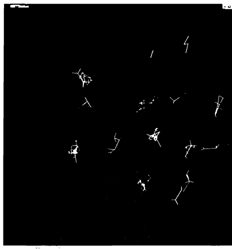
Figure 7.2 A typical fragment of electron density and a section of atomic model from the CUA domain of cytochrome BC3 (Williams et al., 1999) (PDB ID code 2CUA), displayed using XFIT from the XtalView package. Bonds are colored according to the atoms that they join. Putative hydrogen bonds are drawn as dashed white lines. Figure 7.3 also appears in this section.
