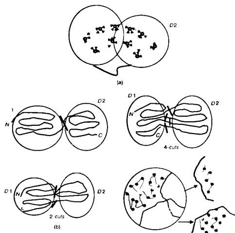
Figure 1B.2. Illustration of the problem of parsing the protein 3D structure into structural domains. (a) The most common definition of structural domains, as groups of residues with a maximum number of contacts within each group and a minimum number of contacts between the groups. (b) Domains may be composed of one or more chain segments. Any domain-assignment procedure must therefore be able to cut the polypeptide chains as many times as necessary. When both domains are composed of contiguous chain segments (continuous domains), only one chain cut (1-cut) is required. When one domain is continuous and the other discontinuous, a situation that may arise as a result of gene insertion, then the chain has to be cut in two places (2-cuts). When both domains are discontinuous, additional chain cuts may be required. In the example shown, the chain is cut in four places (4-cuts), and thus the domain on the left-hand side contains three chain segments, whereas that on the right contains two chain segments. (c) This drawing shows two solutions to the problem of partitioning the protein 3D structure into substructures. To partition the 3D structure into domains, many such solutions need to be examined in order to single out the one that satisfies the criterion given in (a).
