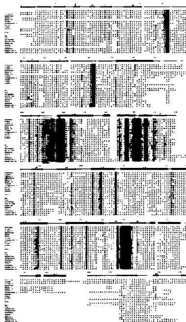
2. MDD sequence alignments. Proteins similar to S. cerevisiae MDD (E-value = 10^{-6} ) were identified using PSI-BLAST (Altschul et al., 1997), and aligned with CLUSTAL (Higgins, and Fuchs, 1992). Secondary structural elements of S. cerevisiae MDD are shown with helices and arrows ( \beta -strands). Grey dots denote poorly resolved residues in the final density map. Color coding denotes sequence conservation among MDDs (white = green = 100% identity). Red box denotes the ATP-binding P-loop. Adapted from (Bonanno
