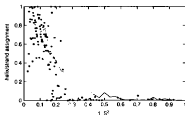
Figure 17.10. Protein motion and secondary structure. Using one set of coordinates from an ensemble of NMR models, the continuous DSSP assignment reproduces the segments in proteins that experimentally had a high degree of motion due to thermal fluctuations in water. Figure reproduced from (Andersen et al., 2001). Protein motion has been independently measured by the order parameter 1 S^2 , by the tumbling of the N-H backbone bond-vector. The order parameter is low when the amino acid is fixed as in the protein core and it is high when the residue fluctuates. The figure shows 1 S^2 versus the continuous DSSP assignment grouping helices (GH) and strands (EB). The points are averages over a window segment of three consecutive residues, the line gives an average of helix/strand assignments.
