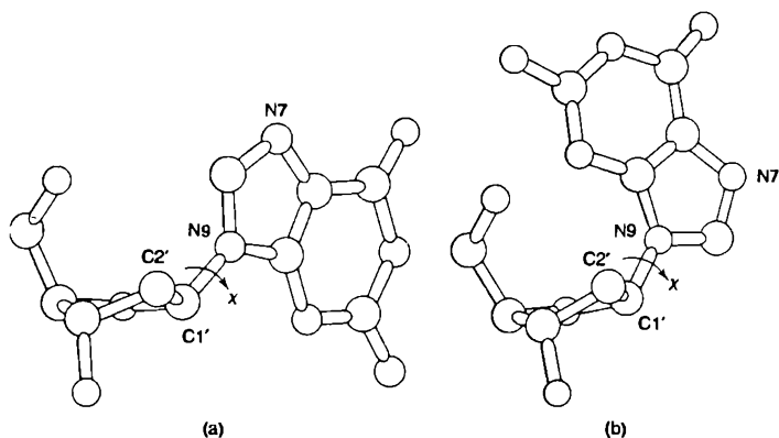
Figure 3.9. (a) A guanosine nucleoside with the glycosidic angle \chi set in an anti conformation. (b) Guanosine now in the syn conformation. From (Neidle, 2002). Reprinted by permission of Oxford University Press.
