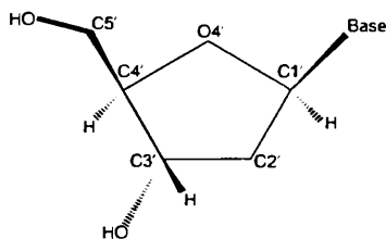
Figure 3.3. The stereochemistry of a natural \beta -nucleoside. Solid bonds are coming out of the plane of the page, toward the reader. Dashed bonds are going away from the reader. Reprinted from (Neidle, 2002). Reprinted by permission of Oxford University Press.
