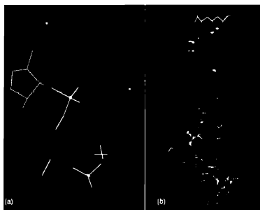
Fig. 15.6. Base and backbone all-atom contacts in the 5S RNA from the 2.4Å 1THK (Ban et al., 2000). (a) A section of the backbone. Backbone contacts are packed but with one impossible overlap of C3 and C4 hydrogens (red sticks). (b) Contacts, showing the long-range well-fit base stacking. Figure also shows a section.
