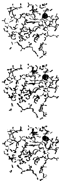
Figure 14.7 Examples of typical uncertainties in atomic positions for (a) an s.u. of 0.2Å, (b) 0.3Å, and (c) 0.39Å. The protein is the same rubredoxin from Figure 14.1a. Of course, as shown in Figure 14.1a, the distribution of uncertainties would not normally be so uniform, with higher variability in the surface side-chain atoms than, say, the buried main-chain atoms.
