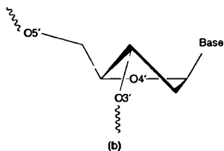
Figure 3.8. (a) C2'-endo sugar pucker for a guanosine nucleoside, viewed along the plane of the sugar ring. (b) C3'-endo sugar pucker for a guanosine nucleoside, with the sugar viewed in the same direction as in panel (a). From (Neidle, 2002). Reprinted by permission of Oxford University Press.
