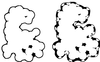
Figure 21.1. Popular definitions of the PBE coefficients. (a) The molecular surface (solid black line) often used to define the dielectric coefficient \epsilon(\mathbf{x}) . This surface can be constructed by rolling solvent probes (small hatched circles) over the macromolecule (large white spheres). Gray regions show areas outside the atomic volume that are treated as inside the molecular surface. (b) The ion-accessible volume is the region outside the solid black line. This volume is defined as the region of space accessible to ion probe spheres (hatched circles).
