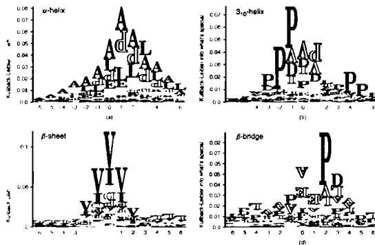
Figure 17.B. Sequence distributions for secondary structure. The four graphs show alignment statistics for (a) \alpha -helices, (b) 3_{10} -helices, (c) \beta -sheets, and (d) \beta -bridges by the Kullback-Leibler information at positions surrounding the one assigned (position 0). The number of aligned segments are: (a) 41,803, (b) 4952, (c) 27,320, (d) 1851. These segments were retrieved from a data set of 707 nonhomologous protein chains using the DSSP assignment. At a given position, we therefore observed the 20 amino acids with a certain frequency; the Kullback-Leibler information calculates the information content of the observed frequencies with respect to the background frequencies (irrespective of the structure). The more an observed set of frequencies differs from the background, the higher the respective letter. If an amino acid at a given position is observed less frequently than in the background, it is drawn upside-down and hollow.
