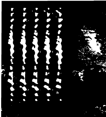
Example for a hybrid study that combines elements of electron crystallography with homology modeling and molecular docking approaches to solve the structure of an actin-fimbrin crosslink (Volkmann et al., 2001b). Fimbrin is a member of the actin-binding protein family and is responsible for cross-linking of actin filaments. It is found in tightly packed networks such as actin bundles in microvilli or stereocilia of the inner ear. The image shows the paracrystalline array of actin-fimbrin crosslinks (background) and the spatial relationship between the actin filaments and the various crosslinks. Combination of this data with homology modeling and data from the structure of fimbrin's N-terminal actin-binding domain into helical reconstruction allowed us to build a complete atomic model of the cross-linking molecule (see Color Figure section).
