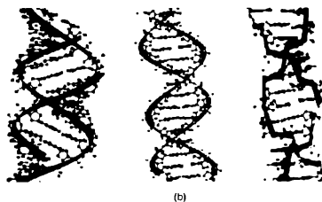
Figure 3.11 Canonical helical types of A-, B-, and Z-DNA from (1996) with permission from Elsevier Science
