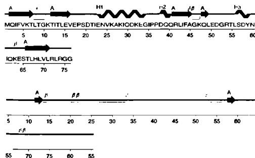
Figure 14.11. Schematic diagrams of two protein models in the PDB. (a) A typical protein showing an expected 50–60% of its residues in \alpha -helices (shown schematically by the sawtooth regions) and \beta -strands (shown by arrows). (b) A poorly defined model that has hardly any regions of secondary structure at all. The labels and symbols correspond to various secondary structure motifs. The \beta and \gamma symbols identify \beta - and \gamma -turns, while the hairpinlike symbols correspond to \beta -hairpins. The helices are labeled H1–H3 in a, and strands are labeled A for \beta -sheet A. The Ramachandran plots for both models are shown in Figure 14.7. The sequence of the protein in b has been removed to hinder identification. The above plots were obtained from the PDBsum database.
