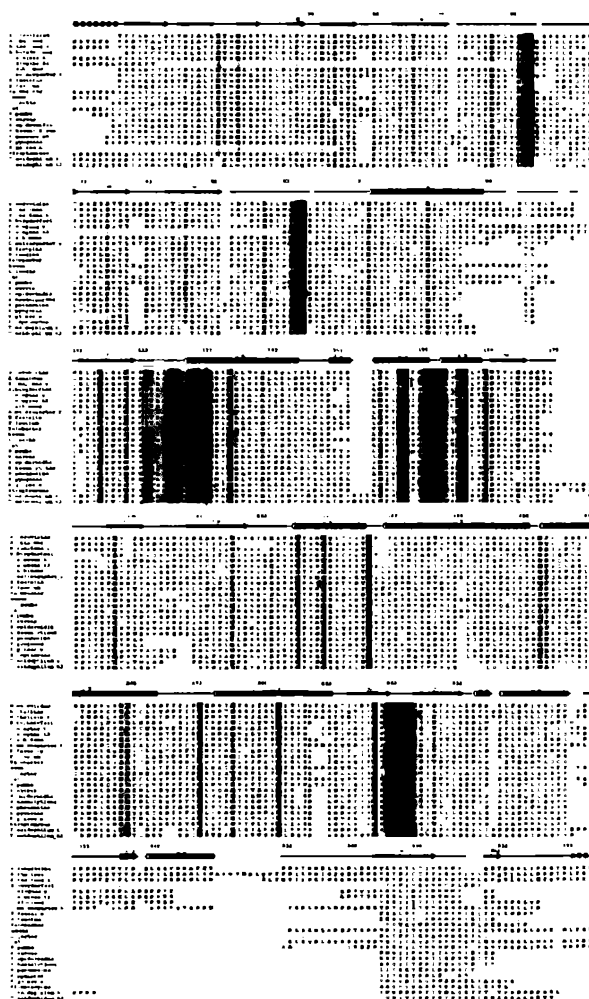
Figure 29.2. MDD sequence alignments. Proteins similar to S. cerevisiae MDD (E-value \sim 10^{-4} ) were identified using PSI-BLAST (Altschul et al., 1997), and aligned with CLUSTAL (Higgins, Bleasby, and Fuchs, 1992). Secondary structural elements of S. cerevisiae MDD are shown with cylinders ( \alpha -helices) and arrows ( \beta -strands). Grey dots denote poorly resolved residues in the final electron density map. Color coding denotes sequence conservation among MDDs (white \rightarrow green ramp, 30 \rightarrow 100% identity). Red box denotes the ATP-binding P-loop. Adapted from (Bonanno et al., 2001). Figure also appears in Color Figure section.
