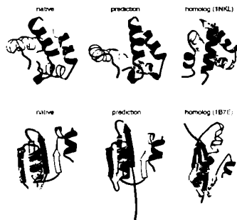
Figure 27.2. Potential of ab initio predictions to detect distant protein homologies. (a) The native structure of bacterial lysis protein Bacteriocin AS-48 (left, PDB id 1E68) is compared to the best ROSETTA prediction for the structure (center), and the native structure of NK Lysin (right, PDB id 1NKL), a functionally similar protein. (b) The native structure of domain 2 of the DNA mismatch repair protein MutS (left, PDB id 1EWQ), is compared to the best ROSETTA prediction for the domain (center), and a domain from the native structure of the Trs transposase inhibitor (right, PDB id 1B7E). In both (a) and (b) the ab initio models of the proteins were of sufficient quality to detect these functional homologs by the similarity of the folds in the absence of significant sequence similarity.
