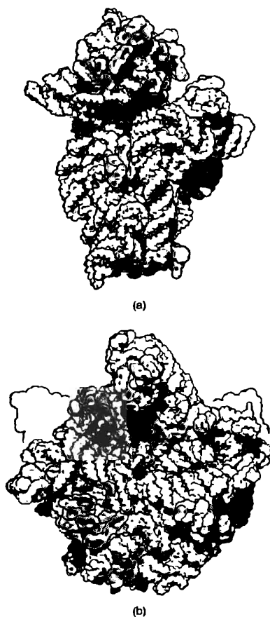
Figure 3.15. The (a) 30S and (b) 50S ribosome structure (Ban et al., 2000; Schlutzen et al., 2000; Wimberly et al., 2000). Image created by David Goodsell for the Protein Data Bank's Molecule of the Month series at http://www.pdb.org/ . Figure also appears in Color Figure section.
