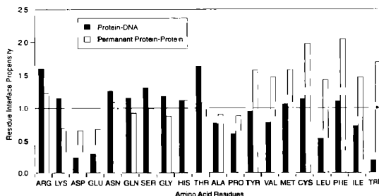
Figure 10.7. Histogram of the interface residue propensities calculated for 26 protein-DNA complexes and compared to those for permanent protein-protein complex (Jones & Thornton, 1995). 'Permanent' complexes are those in which the components only exist as part of a complex, they do not exist in isolation. Generally, they have larger interfaces that are more hydrophobic and more complementary. A propensity of >1 indicates that a residue occurs more frequently in the interface than on the protein surface. The amino acid residues have been ordered using the Faucher & Pliska (Faucher & Pliska, 1983) hydrophobicity scale, with the most hydrophilic residues on the left-hand side and the most hydrophobic on the right-hand side of the graph. Reprinted with permission from (Jones et al., 1999).
