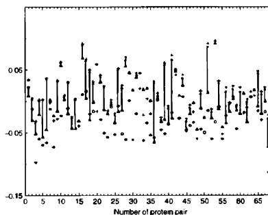
Figure 26.5. Differences between various approximations for energy calculations. Open circles correspond to the real energy, triangles to approximation 4, and crosses to approximation 5 (see text for details).
