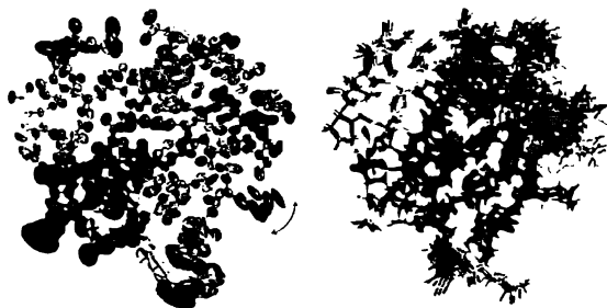
Figure 14.1 The different types of model generated by X-ray crystallography and NMR spectroscopy. Both are representations of the same protein: rubredoxin. (a) In X-ray crystallography the model of a protein structure is given in terms of atomic coordinates, occupancies, and B -factors. The side chain of Glu50 has two alternative conformations, shown in the paler colors, with the change from one conformation to the other identified by the double-headed arrow. The B -factors on all the atoms are illustrated by "thermal ellipsoids," which give an idea of each atom's anisotropic displacement about its mean position. The larger the ellipsoid, the more disordered the atom. Note that the main chain atoms tend to be better defined than the side chain atoms, some of which exhibit particularly large uncertainty of position. Carbons are shown in green, oxygens in red, nitrogens blue, sulfur yellow, and the bound zinc ion in deep pink. The region around the bound zinc ion appears well ordered. This is in stark contrast with the NMR case in (b). The coordinates and B -factors come from PDB entry 1rrn, which was solved at 1.2 Å and refined with anisotropic B -factors. (b) The result of an NMR structure determination is a whole ensemble of model structures, each of which is consistent with the experimental data. The ensemble shown here corresponds to 10 of the 20 structures deposited for as PDB code 1bfy. In this case the metal ion, shown in pink, is iron. Hydrogens are colored white. The more disordered regions represent either regions that are more mobile, or regions with a paucity of experimental data, or a combination of both. The region around the iron-binding site appears particularly disordered. Both diagrams were generated with the help of the Raster3D program (Merritt and Bacon 1997).
