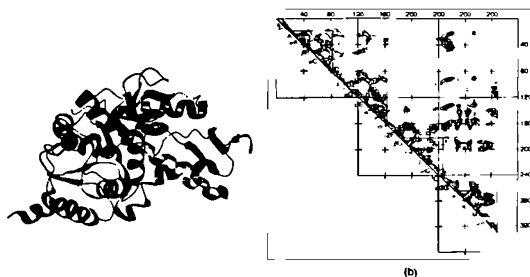
Figure 18.1. Domain structure of dogfish lactate dehydrogenase, determined using the Ca-Ca distance map. (a) Ribbon diagram of lactate dehydrogenase, showing the NAD binding (green) and catalytic domains (red). In gray is part of the helix, spanning residues 164–180, linking the two domains. (b) Distance map and structural domains in lactate dehydrogenase. Contours represent Ca-Ca distances of 4Å, 8Å, and 16Å within the subunit of dogfish lactate dehydrogenase. Elements of secondary structure are identified along the diagonal. Triangles enclose regions where short Ca-Ca distances are abundant. The NAD-binding domain comprises the first two triangles (counting from the N-terminus), which are subdomains. The catalytic domain comprises the last two triangles (the C-terminal domain). From Rossmann and Liljas (1974) and reproduced by permission of Academic Press (London) Ltd. Figure also appears in Color Figure section.
