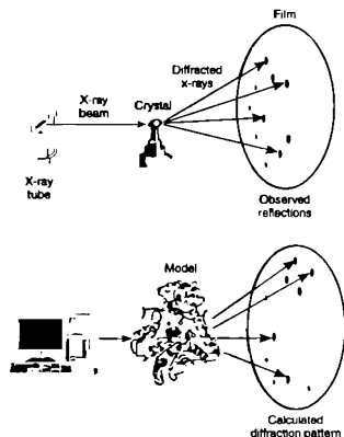
Figure 14.3. A schematic diagram illustrating the principle of structure refinement in X-ray crystallography. (a) X-rays are passed through a crystal of the molecule(s) of interest, generating a diffraction pattern from which, by one method or another (see Chapter 5), an initial model of the molecular structure is calculated. (b) Using the model, it is possible to apply scattering theory to calculate the diffraction pattern we would expect to observe. Usually this will differ from the experimental pattern. The process of structure refinement involves iteratively modifying the model of the structure until a better and better fit between the observed and calculated patterns is obtained. The goodness of fit of the two sets of data is measured by the reliability index, or R -factor.
