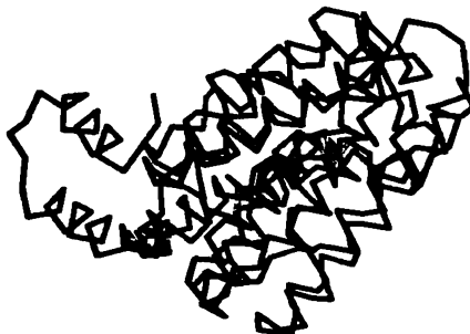
Figure 16.2. Structure alignment as computed by CE for colicin A (1COL: ) (grey) and c-phycocyanin (1CPC.A) (black). The alignment extends over 115 residues with 16 single residue gaps. The rmsd is 3.2Å with a z-score of 5.5. The sequence identity is 13.5%.
