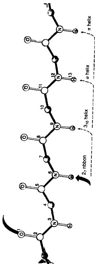
Figure 2.8. The hydrogen bonding patterns of different helical secondary structures. The peptide backbone is shown in an extended conformation, with an arrow denoting the hydrogen bonding pairings that would occur in each type of helix. The common \alpha helix, depicted in Figure 2.7, forms hydrogen bonds between the carbonyl oxygen of each residue and the amide proton of the residue 4 residues ahead in the helix. The 3_{10} helix forms hydrogen bonds between the carbonyl oxygen of each residue and the amide proton of the residue 3 residues ahead, forming a more narrow and elongated helix. The \pi helix forms hydrogen bonds between the carbonyl oxygen of each residue and the amide proton of the residue five residues ahead, forming a wider helix. The 2_7 ribbon is not a regular secondary structure, but is shown here to demonstrate all possible hydrogen bond pairings. From R. E. Dickerson and I. Geis. The Structure and Action of Proteins . New York: Harper & Row, 1969. Used with permission from Geis Archives.
