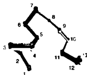
Figure 25.7. Correcting an alignment based on the structure of the modeling template (Ca-trace shown in black). While the alignment with the highest score (dark gray, also in Figure 25.6) leads to a gap of 7.5 Å between residues 7 and 11, the second option (white) creates only a tiny hole of 1.3 Å between residues 5 and 9. This can easily be accommodated by small backbone shifts (The normal Ca–Ca distance of 3.8 Å has been subtracted).
