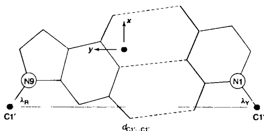
Figure 3.6. Illustration of idealized base-pair parameters, d_{C1'..C1'} and \lambda , used, respectively, to displace and pivot complementary bases in the optimization of the standard reference frame for right-handed A- and B-DNA, with the origin at • and the x- and y-axes pointing in the designated directions. Reprinted with permission from (Olson et al., 2001).
