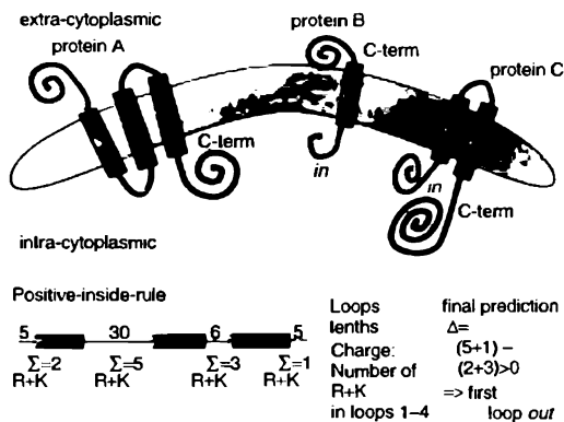
Figure 28.3. Topology of helical membrane proteins. In one class of membrane proteins, typically apolar helical segments are embedded in the lipid bilayer oriented perpendicular to the surface of the membrane. The helices can be regarded as more or less rigid cylinders. The orientation of the helical axes, that is, the topology of the transmembrane protein, can be defined by the orientation of the first N-terminal residues with respect to the cell. Topology is defined as out when the protein N-term (first residue) starts on the extracytoplasmic side (protein A), and as in if the N-term starts on the intracytoplasmic side (proteins B and C). The lower part explains the inside-out rule. The differences between the positive charges are compiled for all even and odd nonmembrane regions. If the even loops have more positive charges, the N-term of the protein is predicted outside. This rule holds for most proteins of known topology.
