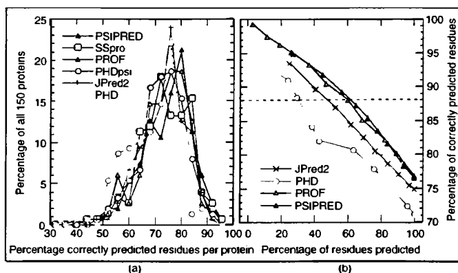
Figure 28.4. Prediction accuracy varies but stronger predictions are better 1 All results are based on 150 novel protein structures not used to develop any of the method shown (Eyrich et al., 2001b; Rost, 2001b). For all methods shown, the three-state per-residue accuracy varies significantly between these proteins, with one standard deviation on the order of 10% (A). This implies that it is difficult for users to estimate the actual accuracy for their protein. However, most methods now provide an index measuring the reliability of the prediction for each residue. Shown is the accuracy versus the cumulative percentages of residues predicted at a given level of reliability (coverage versus accuracy). For example, PSIPRED and PROFphd reach a level above 88% for about 60% of all residues (dashed line). This particular line is chosen since secondary structure assignments by DSSP agree to about 88% for proteins of similar structure. Although JPred2 is only marginally less accurate than PSIPRED and PROFphd, it reaches this level of accuracy for less than half of all residues.
