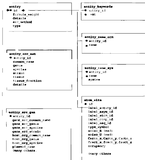
Figure 8.9. A schematic diagram illustrating the content and relationships among a portion of the mmCIF categories describing chemical entities, entity names, entity source organism, and the relationship between the entity and atomic level of description. In this figure, boxes enclose the data items within each mmCIF category, and arrows indicate the correspondence between data items that are common to multiple categories, with the arrowheads pointing in the direction of the parent data item. The category key data items are indicated with black dots.
