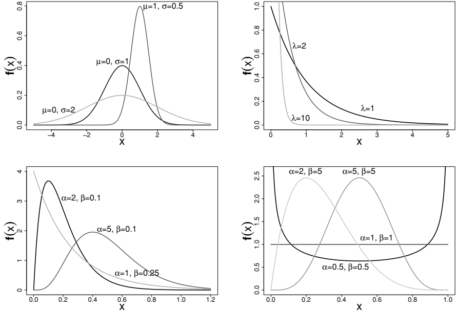
Figure A.3 The densities \mathbf{f}_{\mathbf{X}} for the measures in Table A.1. (Left) Densities of the Gaussian/normal and the Gamma measure. (Right) Densities of the exponential and Beta measure.
