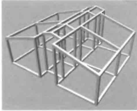
Figure 1.8 Solid frame generated by the expression (Offset:<0.2,0.2,0.2> ~ @1):House . The Offset function is discussed in Section 14.6.3
