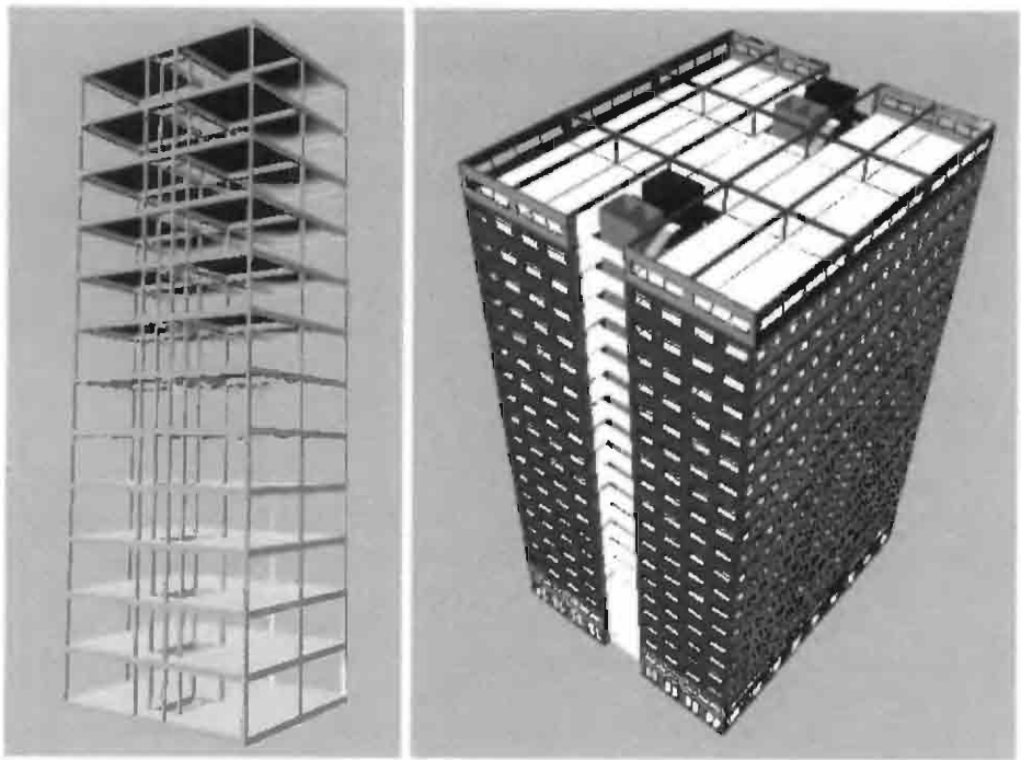
Figure 14.29 (a) Concrete frame of a variational building; (b) schematic design of a short skyscraper. Views generated by a VRML viewer
