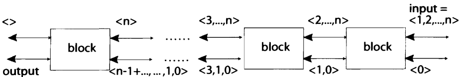
Figure 2.2 Computational pipeline of ProgressiveSum function
