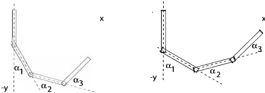
Figure 15.3 Two plane robot configurations generated by arm:<30,45,60> and arm:<60,45,30>
