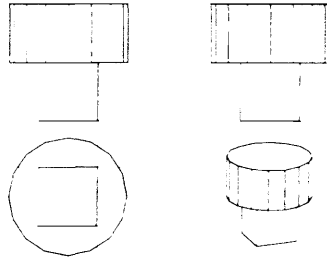
Figure 2.17 Monge's projections and dimetric projection of the result of the expression Cube TOP Cyl
