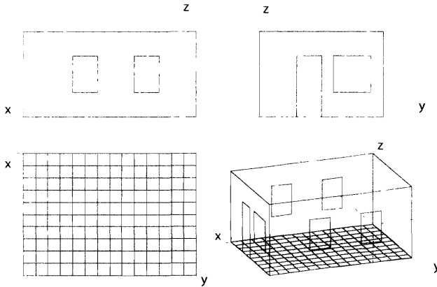
Figure 10.11 Monge's orthographic projections, and axonometric projection
