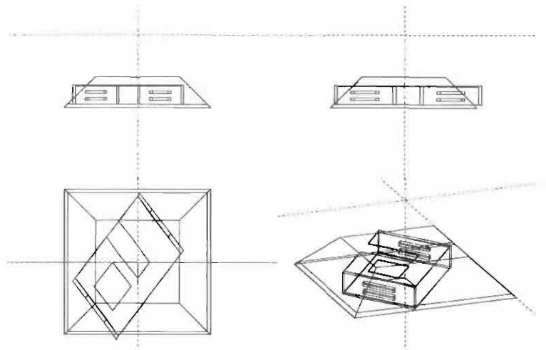
Figure 9.9 House model (in NPC) after the orientation and the view mapping transformation
