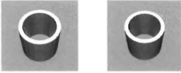
Figure 2.12 Geometric object generated by expression Tube:<0.8,1,2>:24 (a) standard rendering (b) smooth rendering via color shading
