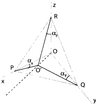
Figure 10.12 Geometric model of the orthogonal axonometric projection
