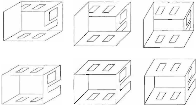
Figure 10.19 Standard military projections with VUV = e_2 and DOP in third and first octant, respectively
