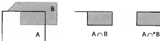
Figure 13.28 Standard set intersection and regularized set intersection
