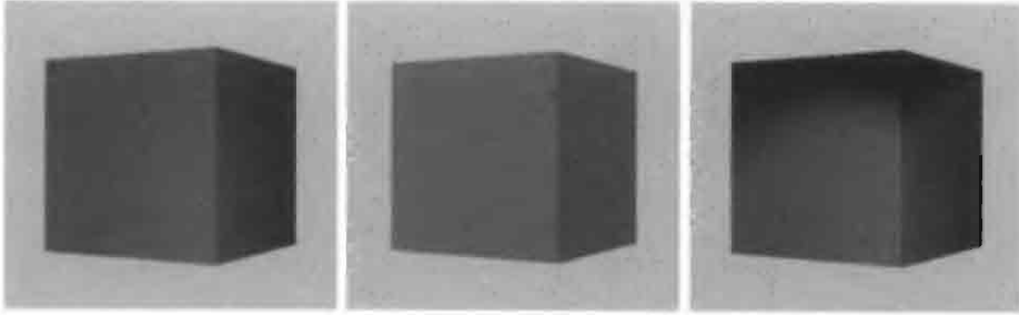
Figure 10.42 Light sources: (a) point (b) directional (c) spot
