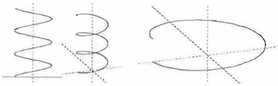
Figure 5.12 Two helices of the same length and different radius
