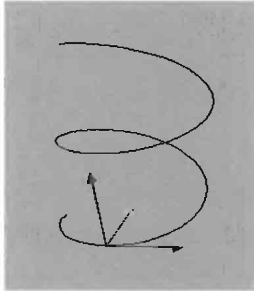
Figure 5.11 Intrinsic triplet at a helix point
