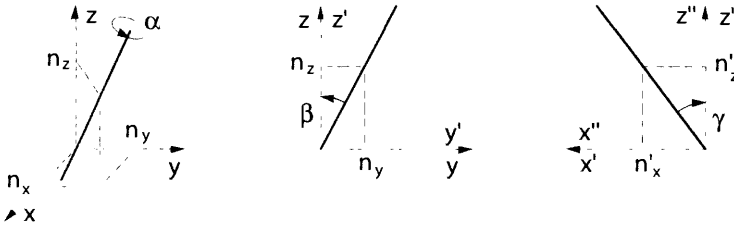
Figure 6.22 Decomposition of a general rotation into elementary rotations: (a) the \mathbf{n} -axis (b) the x -rotation (c) the y -rotation
