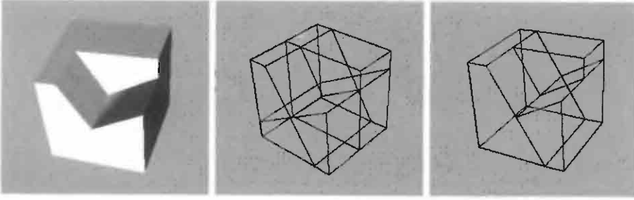
Figure 14.2 Difference between 3D cubes: (a) resulting object (b) set of solid cells of the space partition induced by the cube boundary planes (c) set of solid cells of the pruned BSP tree
