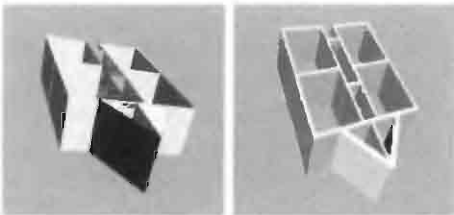
Figure 14.23 (a) 2-complex A in \mathbb{E}^3 (b) 3-complex A + [(0.2, 0), (0, 0.2)]
