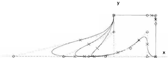
Figure 11.17 Three NURB splines that differ for the weights of a control point
