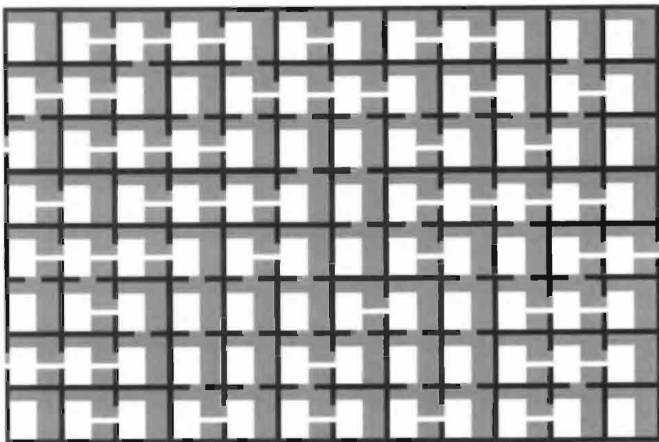
Figure 15.28 A 2D labyrinth (black) and the free configuration space (white) for a moving rectangle CUBOID:<4,2> with 2 translational DOFs only . The gray areas are the grown obstacles. The labyrinth's entrances are unconnected in FP, hence an admissible motion between them does not exist
