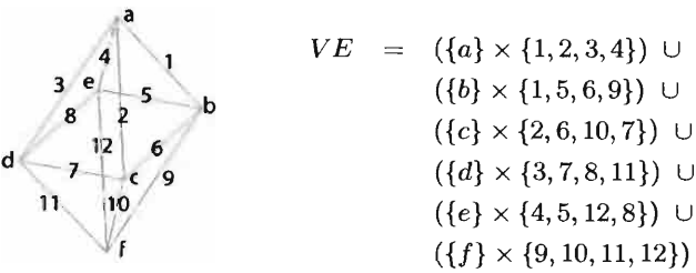
Figure 13.14 Incidence relation VE between vertices and edges
