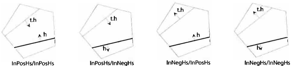
Figure 14.5 The hyperplanes t.h and h do not intersect inside the convex region
