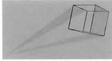
Figure 4.1 Finite cone
