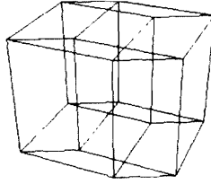
Figure 14.17 1-skeleton of rotated 4D hypercube, projected in \mathbb{E}^3
