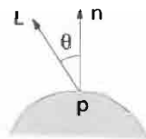
Figure 10.26 Lambert's cosine model of diffused reflection
