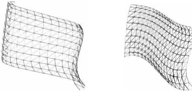
Figure 12.12 (a) Hermite's patch with reversed S^u directions (b) Display of the differences between Hermite's and Ferguson's patches
