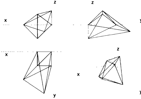
Figure 3.2 Monge projections of the convex hull of the set of points of \mathbb{E}^3 given in Script 3.2.1
