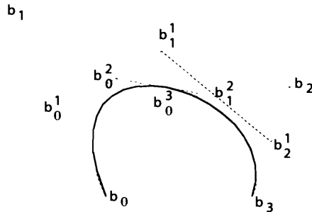
Figure 11.12 The de Casteljau algorithm for a Bézier cubic
