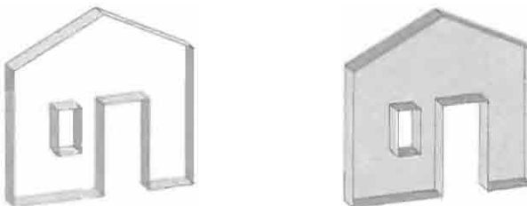
Figure 7.15 (a) object1 value: extruded boundary of a multiply connected triangleStrip (b) object2 value
