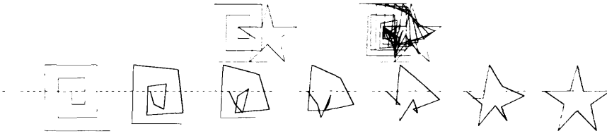
Figure 7.24 A sampling of the straight line in S^{10} between the spiral and star shapes
