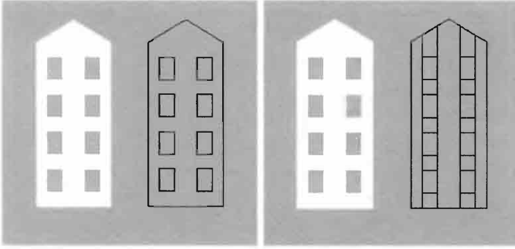
Figure 14.7 2D object and 1-skeleton: (a) BSP unprune (b) BSP prune (standard default)
