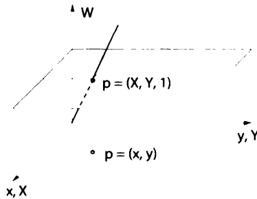
Figure 6.2 Homogeneous coordinates of 2D plane
