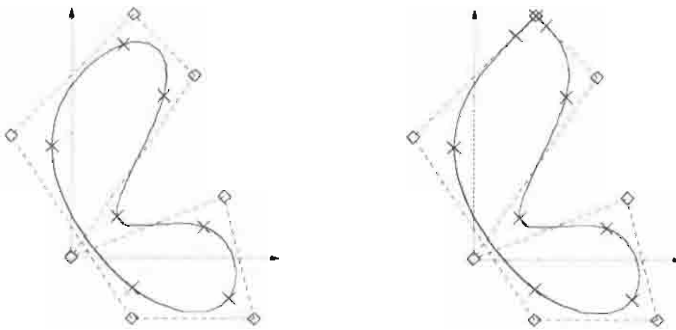
Figure 11.21 (a) Closed cubic uniform B-spline (b) Interpolation of a control point
