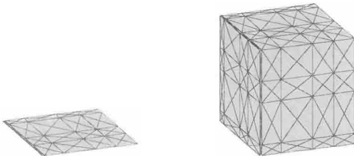
Figure 7.4 Triangulations of non-uniform grids: (a) 2D grid (b) boundary of a 3D grid
