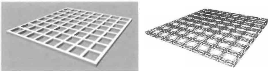
Figure 7.29 Single polyhedron of topologic genus 64 generated by XQUADARRAY:< <1,-4,1,-4,1,-4,1,-4,1,-4,1,-4,1,-4,1>, <1,-4,1,-4,1,-4,1,-4,1,-4,1,-4,1,-4,1> > * Q:1
