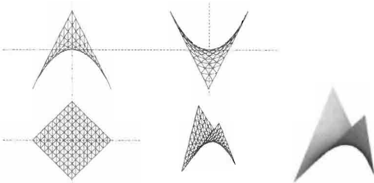
Figure 12.4 The patch S[-1, 1]^2 of hyperbolic paraboloid
