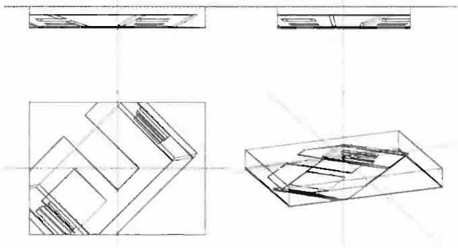
Figure 9.12 Canonical volume after perspective transformation, clipping and scaling to the window 2D
