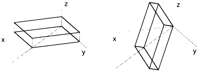
Figure 6.23 Action of a rotation tensor \text{Rot\_xyz}:\langle \pi/2, \langle 1, 1, 0 \rangle \rangle of angle \pi/2 about axis n = [1 \ 1 \ 0]^T
