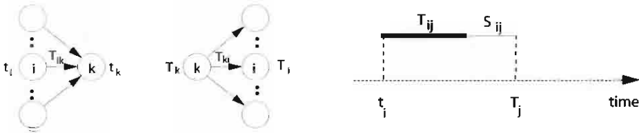
Figure 15.11 (a) Predecessors and successors of the k event (b) Duration T_{i,j} and slack S_{i,j} of the (i, j) segment
