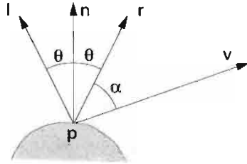
Figure 10.27 Specular reflection from a point source
