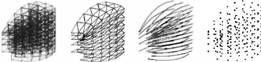
Figure 12.15 (a) Three-quadratic Bézier solid (b), (c) and (d) Submanifolds of dimensions 2, 1 and 0, respectively
