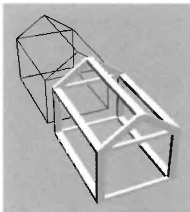
Figure 14.27 Solid model generated by offset operator from a wire model
