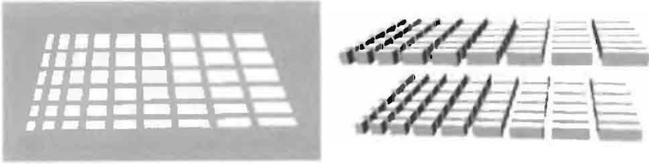
Figure 1.16 (a) Cartesian product of two 1D polyhedral complexes (b) Cartesian product of three 1D polyhedral complexes
