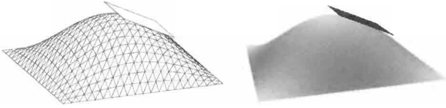
Figure 5.7 Graphs of map \phi on [0, \pi]^2 and of map (\phi + D\phi)(\frac{\pi}{3}, \frac{\pi}{2}) on [-1, 1]^2 , with \phi = \sin u \sin v : (a) polyhedral approximation (b) smooth rendering
