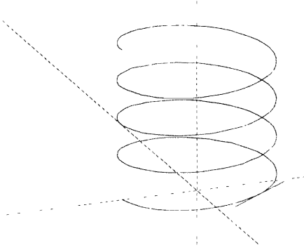
Figure 5.6 Image of the tangent map to the helix curve at the point \frac{2}{3}\pi
