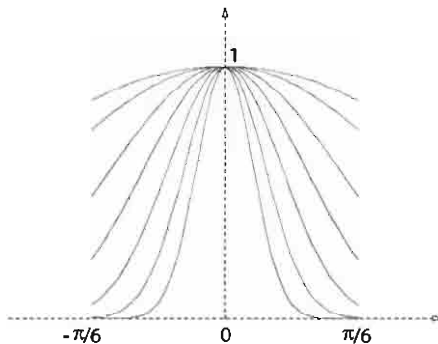
Figure 10.28 Graph of function \cos^n \alpha , for -\frac{\pi}{6} \leq \alpha \leq \frac{\pi}{6} , and with samples of n between 1 and 80
