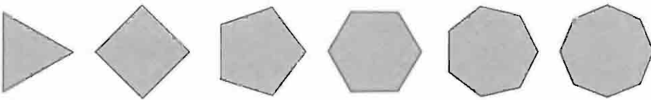
Figure 4.3 Regular polygons with a number of sides from 3 (triangle) to 8 (octagon)
