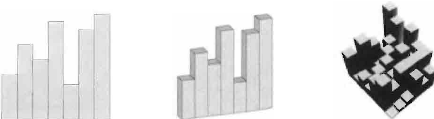
Figure 2.16 (a) 2D histogram (b) 3D histogram (c) 3D histogram of a double sequence of values
