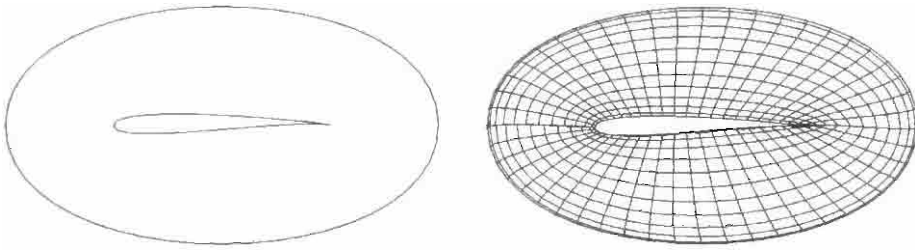
Figure 12.20 (a) The plane domain bounded by the four curve maps c_1 , c_2 and b_1 , b_2 (b) Wire-frame picture of domain \text{grid1}(\Sigma[0, 1]^2) \cup \text{grid2}(\Sigma[0, 1]^2) .
