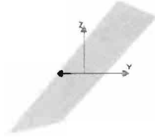
Figure 3.3 Plane passing for (0, 0, 0) , (1, 0, 0) and (1, 1, 1)
