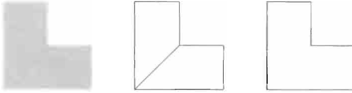
Figure 1.2 (a) L-shaped polyhedral complex produced by the MKPOL primitive (b) 1-skeleton of the definition with 2 polyhedral cells (c) 1-skeleton of the definition with 1 polyhedral cell
