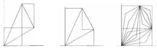
Figure 7.22 The triangle t displayed with: (a) the associated t^{sup} (b) the associated t^{inf} (c) a family of convex combinations of such shapes
