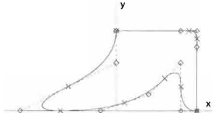
Figure 11.16 Quadratic NURB spline generated by 12 control points and by a suitable knot sequence
