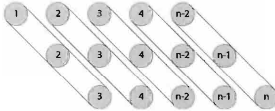
Figure 7.12 Generation of a set of triangles from the point sequence of triangleStrip
