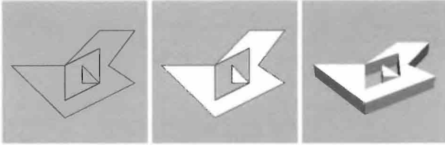
Figure 14.9 (a) Set of 2D polylines (b) 2D polygon generated by Solidify operator (c) Non-manifold solid generated by extrusion
