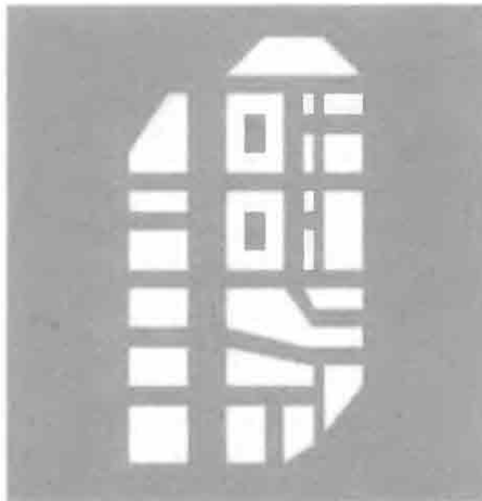
Figure 1.18 Polyhedral complex generated by evaluating the object Manhattan2D
