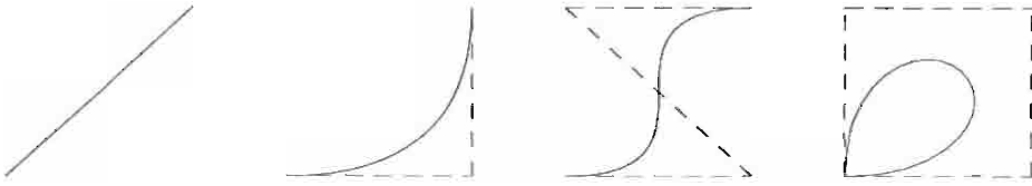
Figure 11.4 Bézier curves of degrees 1, 2, 3 and 4 with their control polygons
