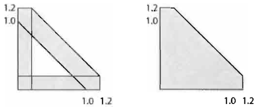
Figure 14.22 Offset objects: (a) \partial\sigma^2 + [V] (b) \sigma^2 + [V] , with V = \{(0.2, 0), (0, 0.2)\}
