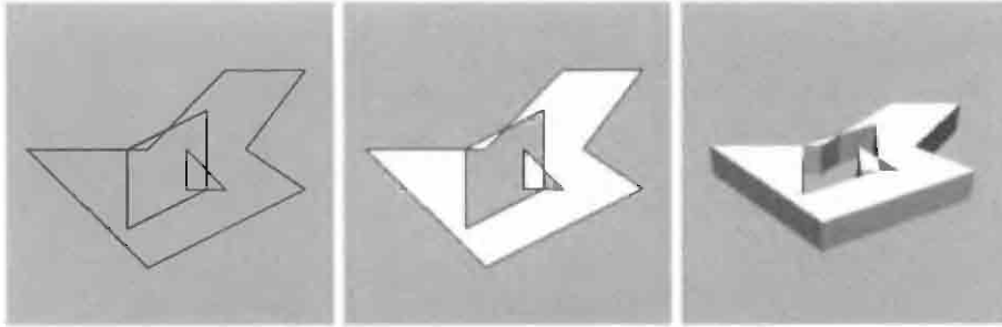
Figure 14.10 (a) 2D Self-intersecting polylines (b) Generated 2D polygon (3) Extruded solid. The results are always valid !
