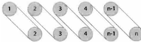
Figure 7.2 Generation of a set of segments from the point sequence of a polyline
