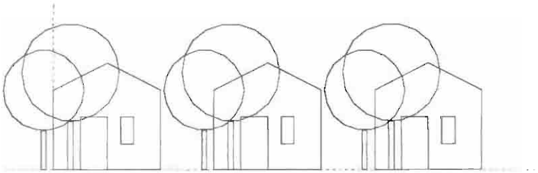
Figure 6.8 Geometric value generated by the evaluation of the PLaSM expression triplet:HouseTrees
