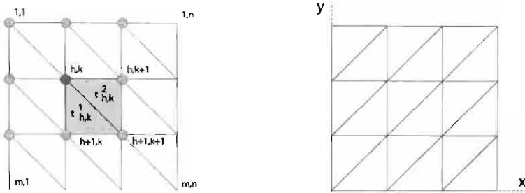
Figure 7.17 (a) Algorithmic scheme of QUADMESH (b) 2D grid generated by QUADMESH on a 4 \times 4 grid of integer 2D points
