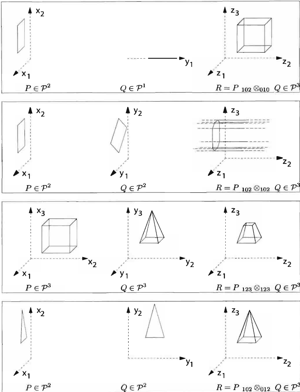
Figure 14.14 Some applications of the product operator: (a) Cartesian product (b) intersection (c) and (d) intersection of extrusions
