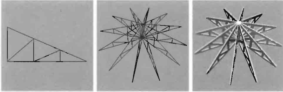
Figure 1.22 (a) 2D model generated by Trellis2D:<12,23> (b) 3D model generated by Radial:12:Trellis3D (c) Solid model generated by Radial:12:SolidTrellis
