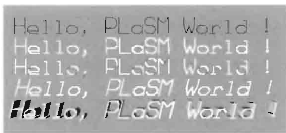
Figure 7.10 (a) Vector text (b) Offset text (c) Swept text (d) Slanted offset text (e) Extruded slanted offset text
