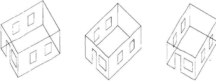
Figure 10.17 Left, centered and right standard military projections
