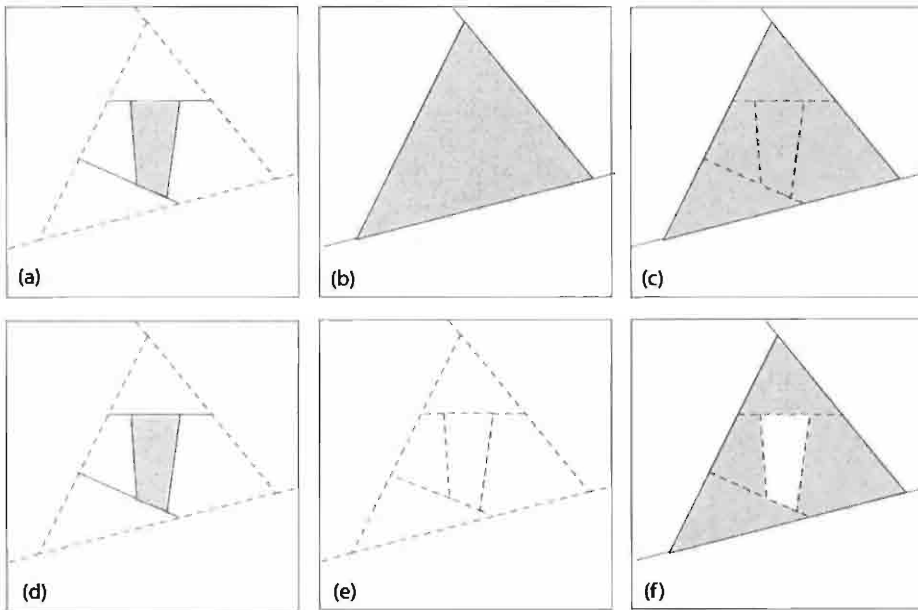
Figure 14.6 Combinations of a t_1 subtree within a t_2 leaf: (a) t_1 subtree (b) t_2 leaf (c) t_1 \cup t_2 (d) t_1 \cap t_2 (e) t_1 - t_2 (f) t_1 \wedge t_2
