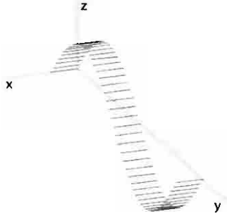
Figure 7.1 Polyhedral complex of dimension (1,3) generated by sampling the sin function with the points operator
