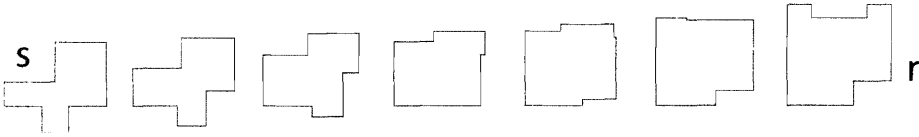
Figure 7.23 The convex interpolation of two orthogonal shapes s and r
