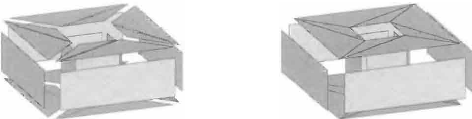
Figure 10.54 xyz -exploded view of boundary: (a) convex cells (b) polyhedral cells
