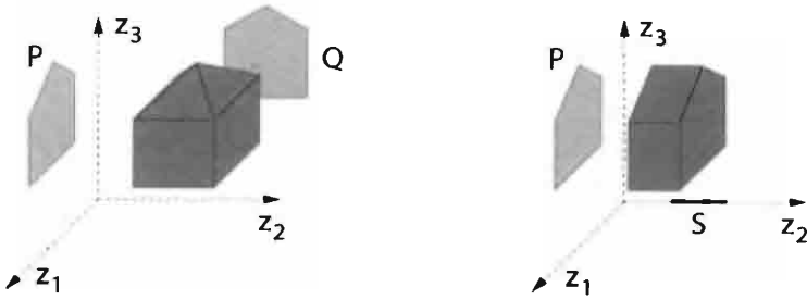
Figure 14.13 Intersection of two extruded polyhedra: (a) P_{102} \otimes_{012} Q (b) P_{102} \otimes_{010} S
