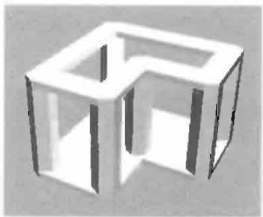
Figure 14.28 Minkowski sums with an hexagonal cell
