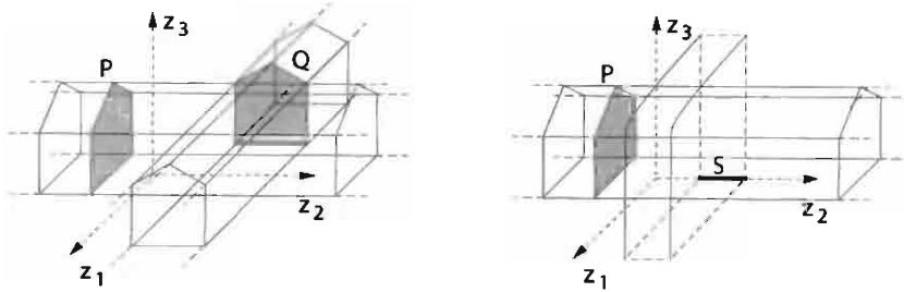
Figure 14.12 Extrusion of two polyhedra in \mathbb{R}^3
