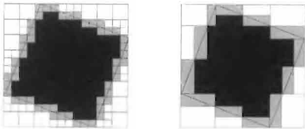
Figure 13.7 Quadtree vs bintree
