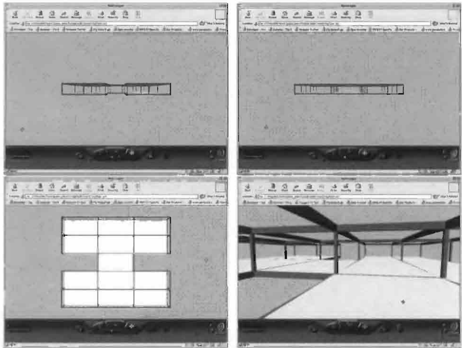
Figure 9.18 Different viewpoints in PLASM-generated VRML model of beams and pillars in a building fabric
