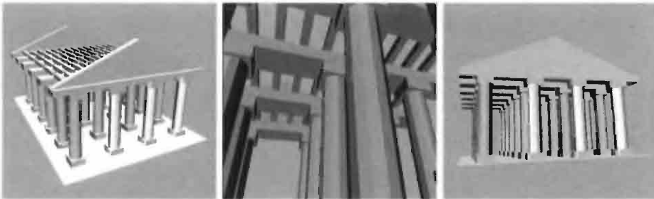
Figure 2.22 Three views from the VRML file of the temple generated by PLaSM
