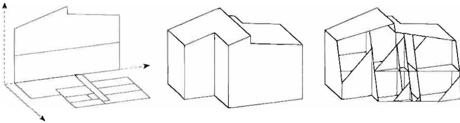
Figure 14.15 The product operator used as an intersection of extrusions. The generating expression is @2(A_{120} \otimes_{102} B) , where A and B are shown on the left and @2() is the extraction operator for the 2-skeleton.
