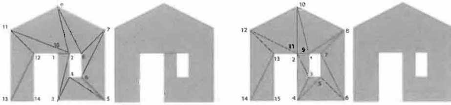
Figure 7.14 (a) Sequence of triangleStrip vertices not corresponding to a simplicial complex (b) Generated polygon (c) Sequence of triangleStrip vertices which correspond to a simplicial complex (d) Generated polygon
