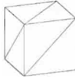
Figure 13.26 Winged-triangle representation of cube boundary
