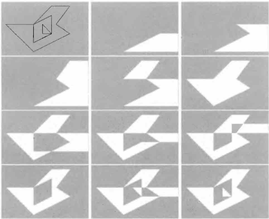
Figure 14.8 The boundary-to-interior algorithm, based on the xor of stripes generated by boundary cells
