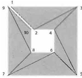
Figure 7.13 The ordering of triangleStrip vertices which produces a 2D solid polygon with a hole
