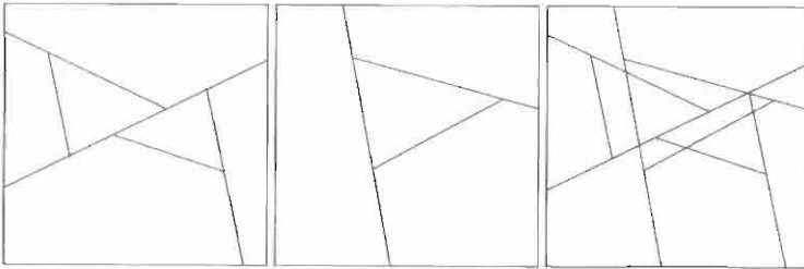
Figure 14.3 Two binary space partitions. To execute a set operation the two partitions must be merged
