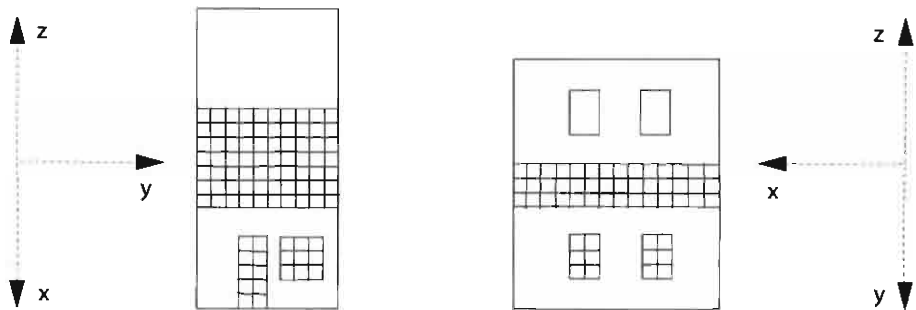
Figure 10.20 (a) Front and side military projections, with DOP in the xz and yz plane, respectively (b) Projected images of basis vectors
