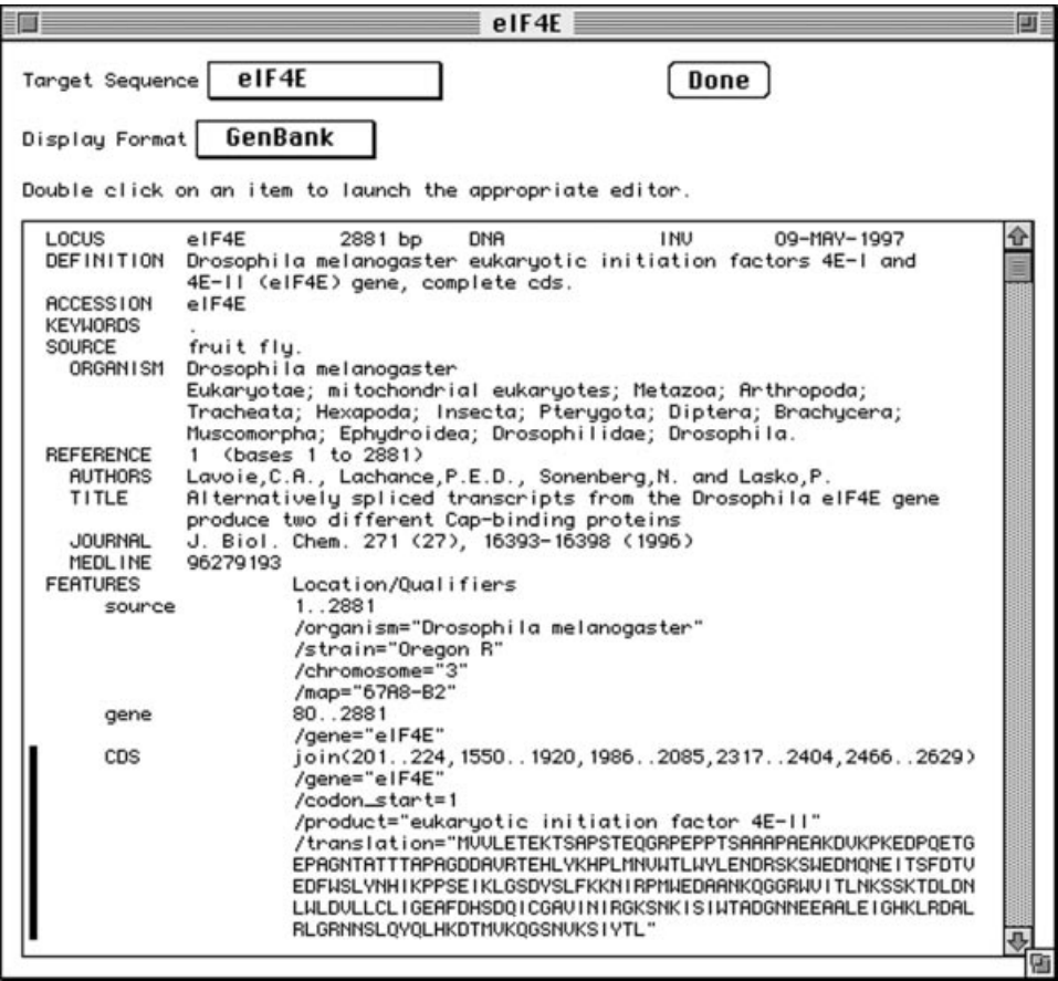
Figure 4.1. Viewing a sequence record with Sequin. The sequence record viewer uses GenBank format, by default. In this example, a CDS feature has been clicked, as indicated by the bar next to its paragraph. Double-clicking on a paragraph will launch an editor for the feature, descriptor, or sequence that was selected. The viewer can be duplicated, and multiple viewers can show the same record in different formats.
