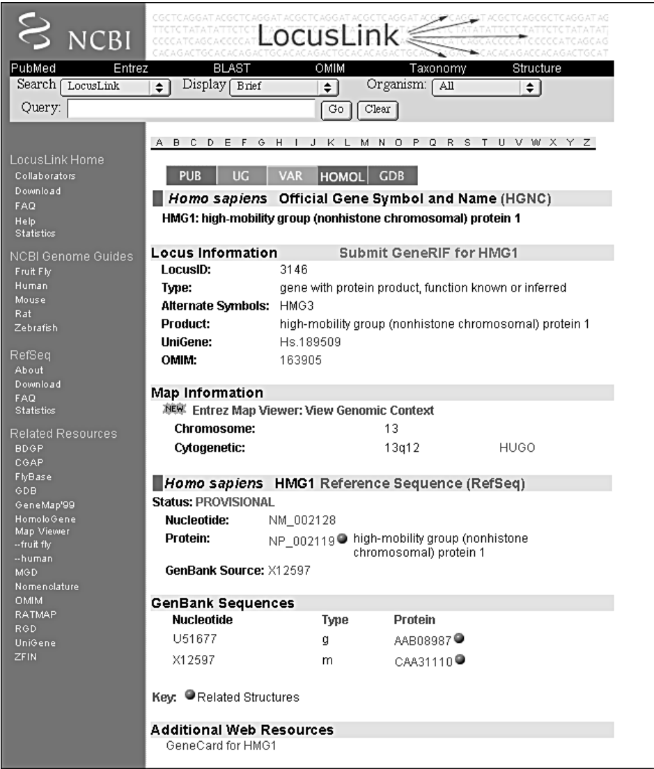
Figure 7.14. The LocusLink report view for human HMG1. The report is divided into six sections, providing gene symbol, locus, map, RefSeq, and GenBank information, as well as links to external data sources. See text for details.
