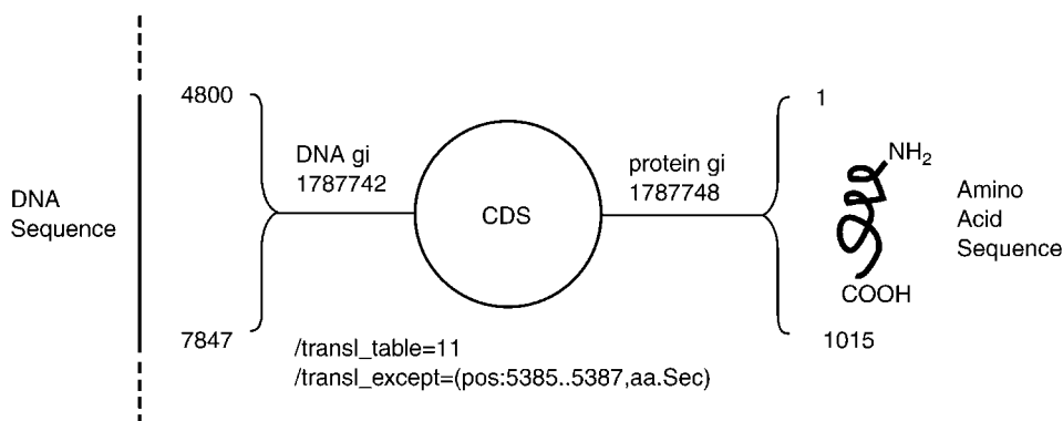
Figure 2.3. The Coding Region (CDS) feature links specific regions on a nucleotide sequence with its encoded protein product. All features in the NCBI data model have a “location” field, which is usually one or more intervals on a sequence. (Multiple intervals on a CDS feature would correspond to individual exons.) Features may optionally have a “product” field, which for a CDS feature is the entirety of the resulting protein sequence. The CDS feature also contains a field for the genetic code. This appears in the GenBank flat file as a /transl_table qualifier. In this example, the Bacterial genetic code (code 11) is indicated. A CDS may also have translation exceptions indicating that a particular residue is not what is expected, given the codon and the genetic code. In this example, residue 196 in the protein is selenocysteine, indicated by the /transl_except qualifier. NCBI software includes functions for converting between codon locations and residue locations, using the CDS as its guide. This capability is used to support the historical conventions of GenBank format, allowing a signal peptide, annotated on the protein sequence, to appear in the GenBank flat file with a location on the nucleotide sequence.
