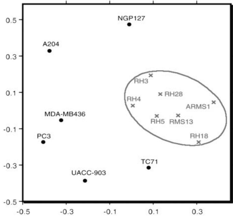
Figure 16.13. Multidimensional scaling plot of the same data represented in Figure 16.12. Note that the samples that fall closely together in the dendrogram also plot near to one another in the MDS plot. Ideally, this plot should be viewed in three dimensions on a computer screen so that it can be rotated to allow better inspection of the distances between the data points.
