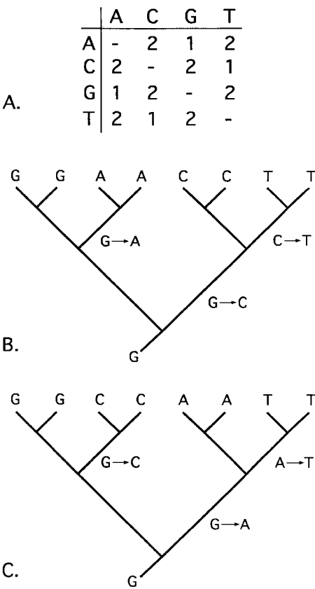
Figure 14.5. Character weight matrix and application in MP phylogenetic analysis. (A) Matrix indicating that a transversion substitution costs twice that of a transition. Because, according to MP bases shared between two sequences cannot ever have changed, diagonal elements of the matrix are ignored. (B, C) Two phylogenetic resolutions and reconstructions of the evolution of a hypothetical pattern of aligned bases at a particular site in eight sequences. With unweighted MP, both reconstructions (among several others) have the same cost (three steps); hence, they are equally acceptable. With the weight matrix in (A), the reconstruction of (B) requires four steps, and the reconstruction of (C) requires five. Thus, the first reconstruction (B) and others requiring four steps are preferred.
