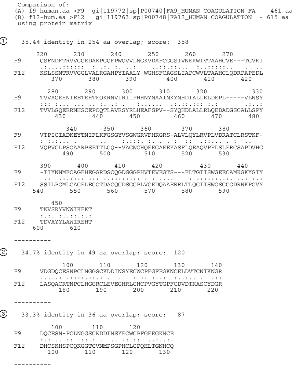
Figure 8.6. Optimal and suboptimal local alignments. The three best alignments found when using lalign to align the sequences of human coagulation factor IX (F9; SWISS-PROT 900740) and coagulation factor XII (F12; SWISS-PROT P00748).
