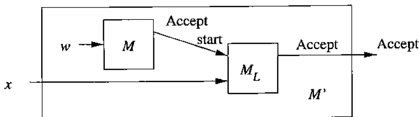
Figure 9.10: Construction of M' for the proof of Rice's Theorem
