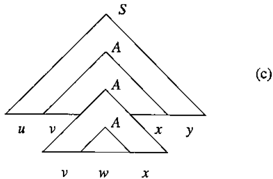
Figure 7.7: Pumping strings v and x zero times and pumping them twice
