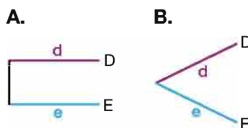
Figure 6.16. Branch lengths of most closely related sequences by UPGMA method.
