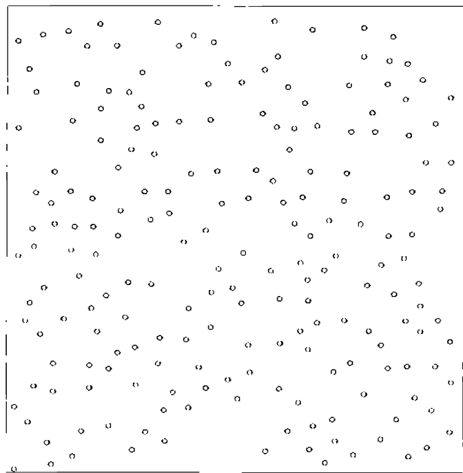
Figure 4.25 Realization of a simple sequential inhibition process with periodic boundaries.
