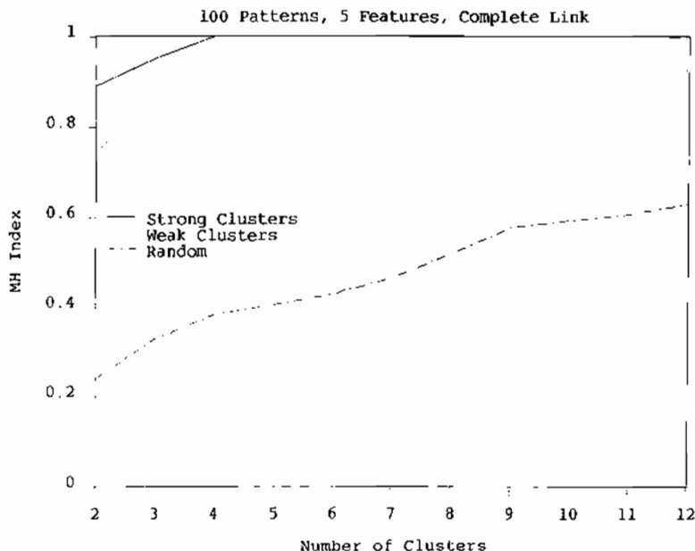
Figure 4.14 MH relative index for strongly and weakly clustered data containing four clusters and for random data.
