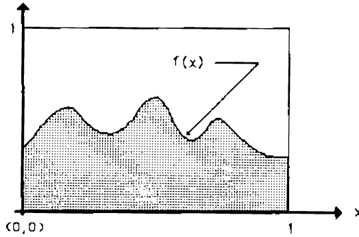
Figure 4.4 Evaluating an integral with Monte Carlo analysis.
