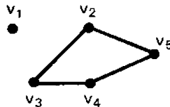
Cycles in the Reference Graph
