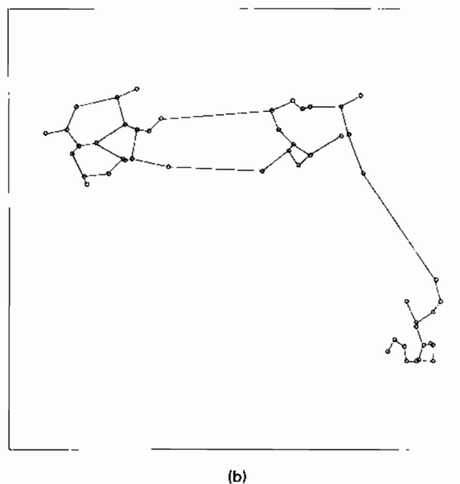
Figure 3.33 MST, RNG, GG, and Delaunay triangulation for the data in Figure 3.30(a): (a) MST; (b) RNG; (c) GG; (d) Delaunay triangulation.
