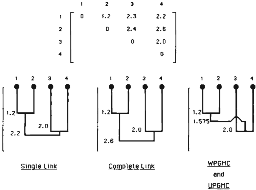
Figure 3.14 Examples of crossover or reversal in dendrogram.
