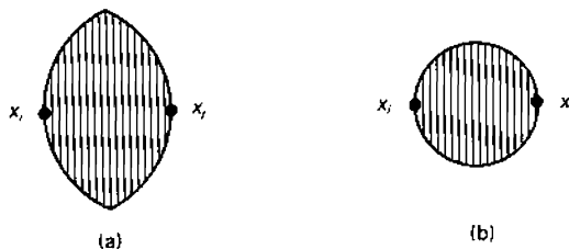
Figure 3.32 Regions of influence for RNG and GG.
