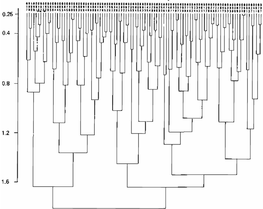
Figure 3.11 Complete-link hierarchy for 100 random patterns in six dimensions.
