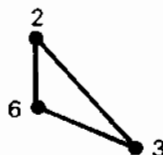
Maximal Complete Subgraphs
