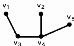
Not a Subgraph
