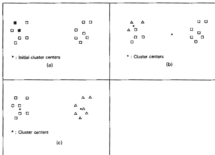
Figure 3.19 Convergence of K -means clustering: (a) initial data; (b) cluster membership after first loop; (c) cluster membership after second loop.
