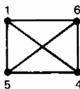
Maximal Complete Subgraphs
