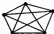
Complete Graph on 5 Vertices
