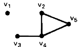
Not a Cycle
