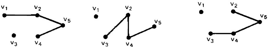
Some Subgraphs That Are Paths
