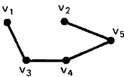
Not a Path in the Reference Graph
