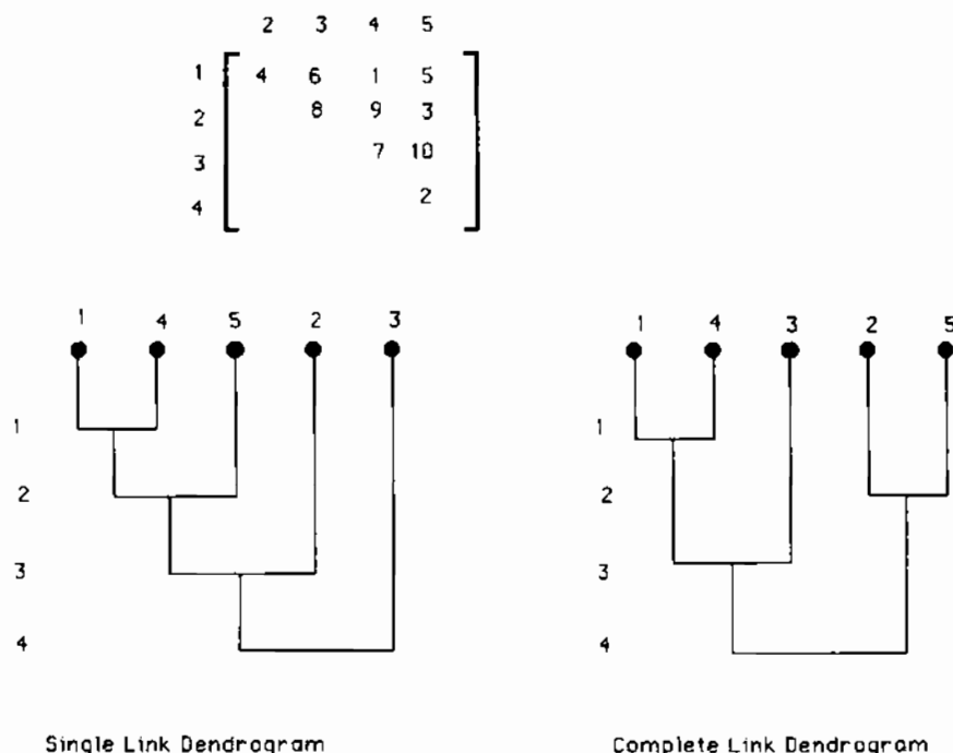
Figure 4.8 Single-link and complete-link dendrograms for the ordinal proximity matrix in Example 4.5.
