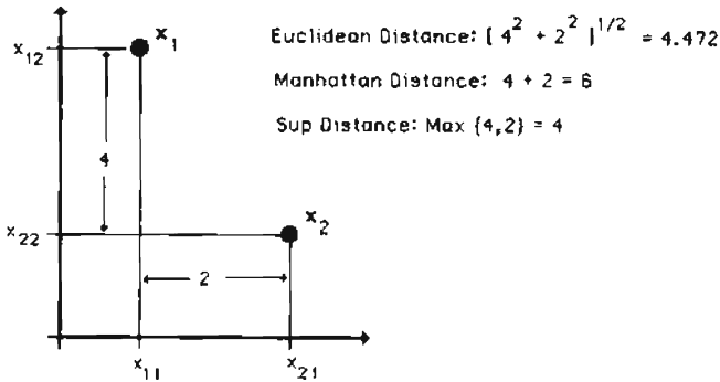
Figure 2.3 Minkowski metrics.
