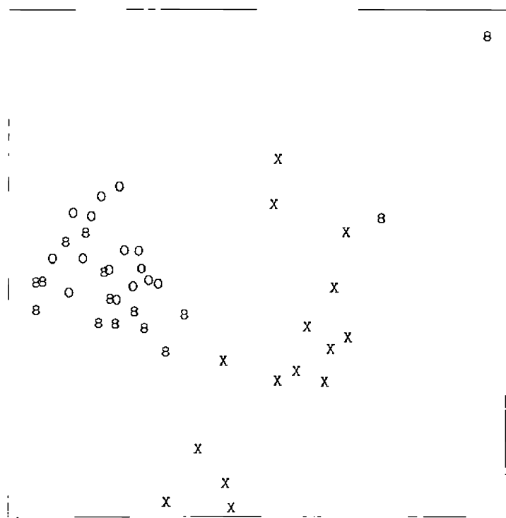
Figure 2.6 Two-dimensional representation of 8OX data on the first two principal components.
