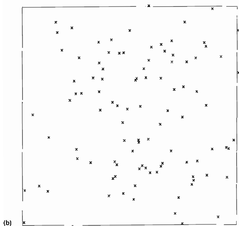
Figure 4.10 Eigenvector projections of six-dimensional data sets.
