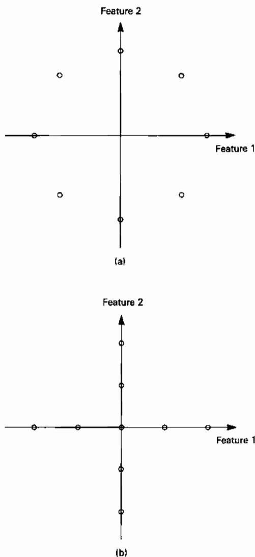
Figure C.1 Two sets of two-dimensional patterns.
