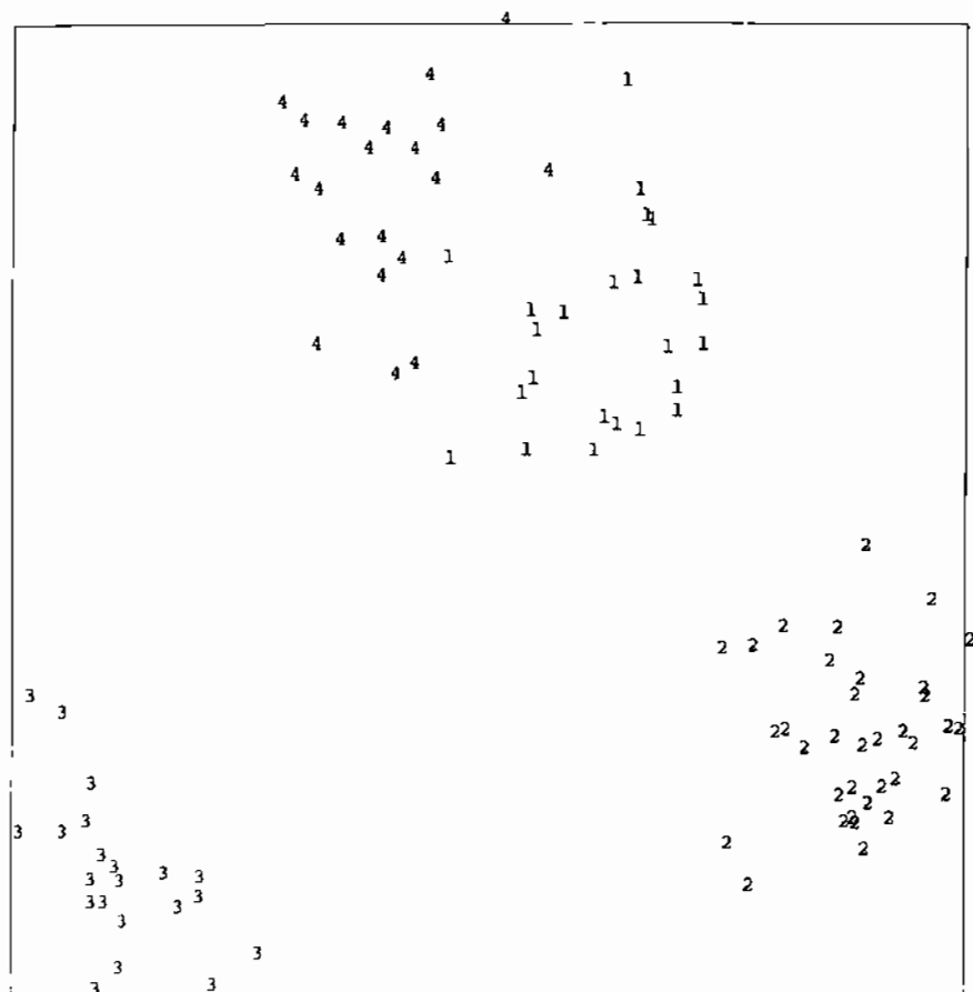
Figure 2.10 Two-dimensional projection of DAT1 showing category labels.
