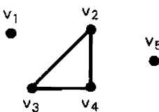
Cycles in the Reference Graph
