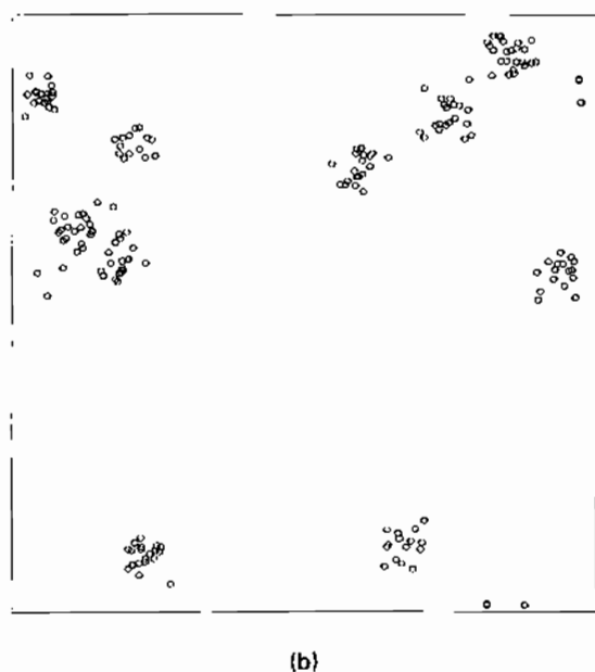
Figure 4.24 Realizations of Neyman-Scott cluster processes with periodic boundaries: (a) cluster process (200 patterns, \mu = 20 , \sigma = 0.75 ); (b) cluster process (200 patterns, \mu = 20 , \sigma = 0.025 ).
