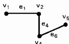
A Connected Subgraph
