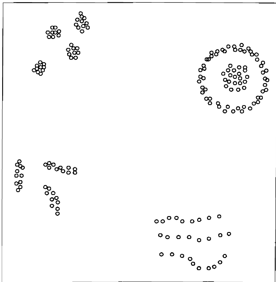
Figure 1.1 Clusters of point patterns in two dimensions.
