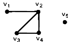
Not a Path (Repeated Vertex)
