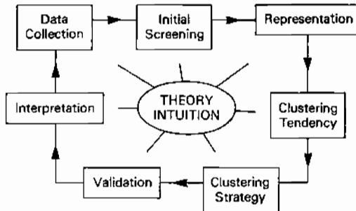
Figure 3.35 Clustering methodology.
