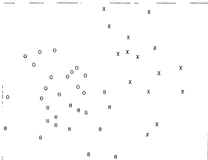
Figure 2.13 Projection of 80X data by Sammon's method.
