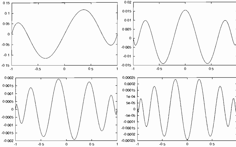
Figure 2.33 Error factor \beta_p(x) for Chebyshev nodal points, p = 4, 7, 10 and 13 .
