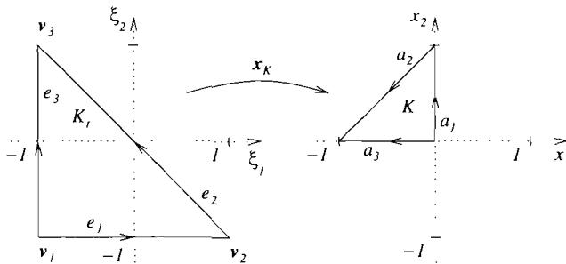
Figure 7.8 Affine transformation x_K : K_t \rightarrow K .
