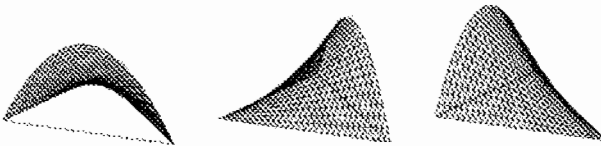
Figure 4.17 Nodal basis of the P^2 -element; the edge functions \varphi_{1,t}^{e_1} , \varphi_{1,t}^{e_2} , and \varphi_{1,t}^{e_3} .
