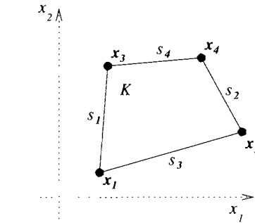
Figure 3.3 Q^1 -element on a quadrilateral domain K \subset \mathbb{R}^2 .
