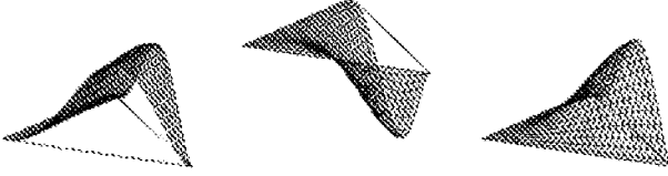
Figure 6.34 Nodal basis of the quintic Argyris element; shape functions \varphi_t^{v_2,1,1} , \varphi_t^{v_2,1,2} , and \varphi_t^{v_2,2,2} , representing \partial^2/\partial x_1^2 , \partial^2/\partial x_1\partial x_2 , and \partial^2/\partial x_2^2 at the vertex v_2 .
