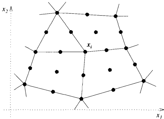
Figure 4.23 Element patch S(i) corresponding to an unconstrained vertex x_i in a hybrid Q^2/P^2 mesh.
