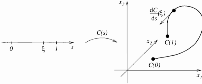
Figure 7.1 Parameterization of a smooth curve and its derivative.
