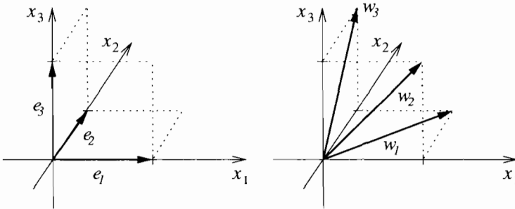
Figure A.8 Canonical basis of \mathbb{R}^3 .
