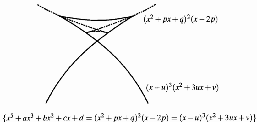
Fig. 1: The section by the plane a = -1 of the caustic (continuous line) and the Maxwell strata (dotted line) of the family x^5 + ax^3 + bx^2 + cx (the constant term d is discarded)
