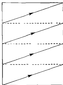
\frac{a}{b} rational
