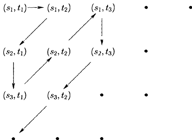
Figure 1.1 Product of two countable sets is countable
