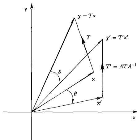
Figure 3.2 Active view of a similarity transformation
