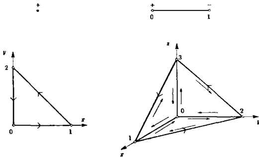
Figure 17.5 Standard low dimensional p -simplices
