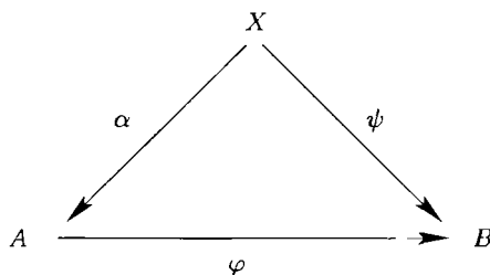
Figure 1.3 Monomorphism \varphi
