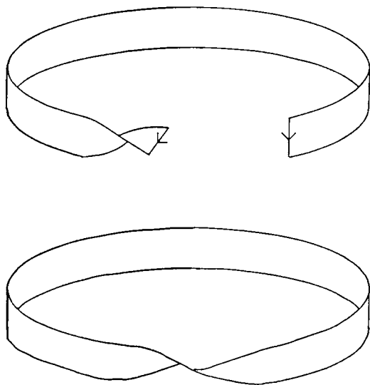
Figure 17.1 Möbius band
