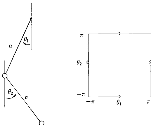
Figure 16.3 Double pendulum
