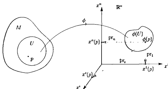
Figure 15.1 Chart at a point p
