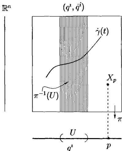
Figure 16.1 Tangent bundle
