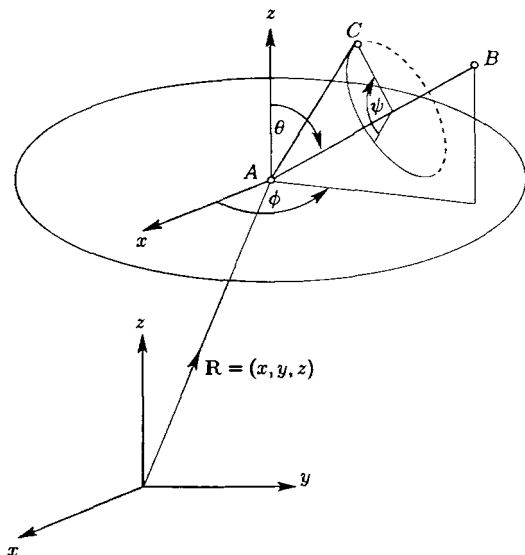
Figure 16.4 Degrees of freedom of a rigid body
