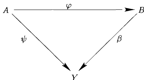
Figure 1.4 Epimorphism \varphi
