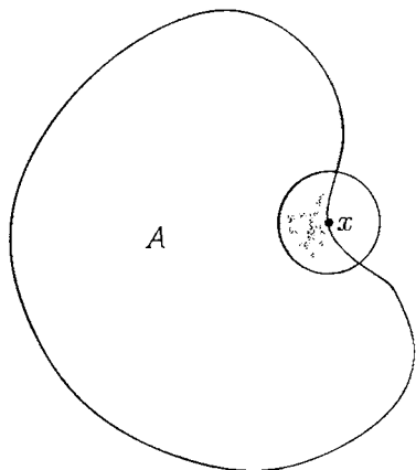
Figure 10.3 Accumulation point of a set
