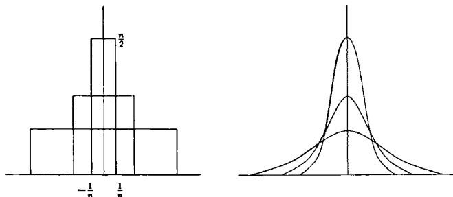
Figure 12.1 Dirac delta function as a limit of functions
