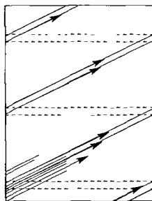
\frac{a}{b} irrational
