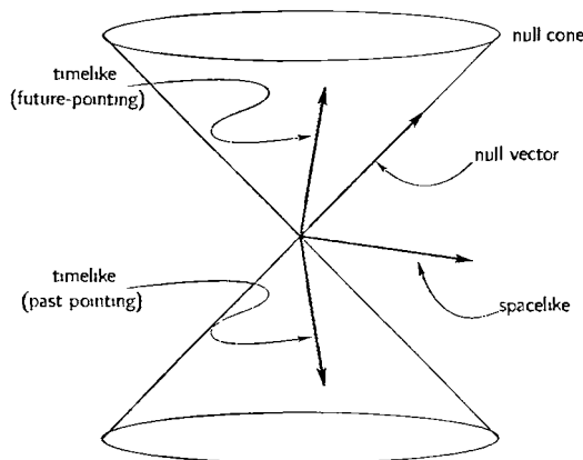
Figure 9.1 The null cone in Minkowski space
