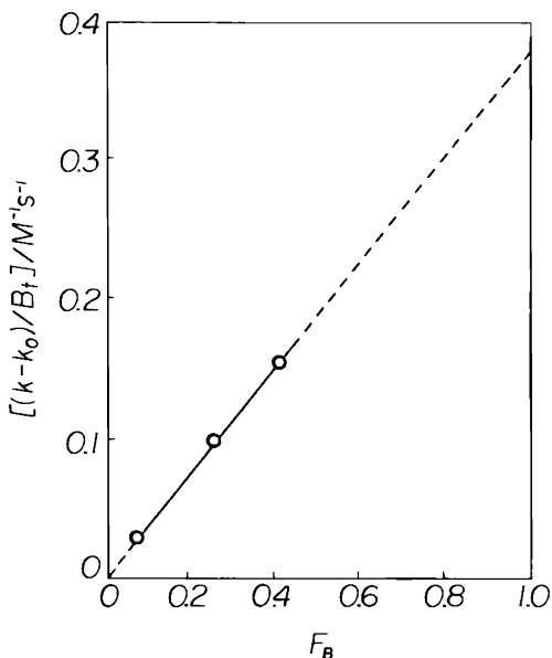
Figure 6-5. Plot according to Eq. (6-47) of the results in Fig. 6-4. The points, from top to bottom, correspond to pH 10.06, 9.76, and 9.14.
