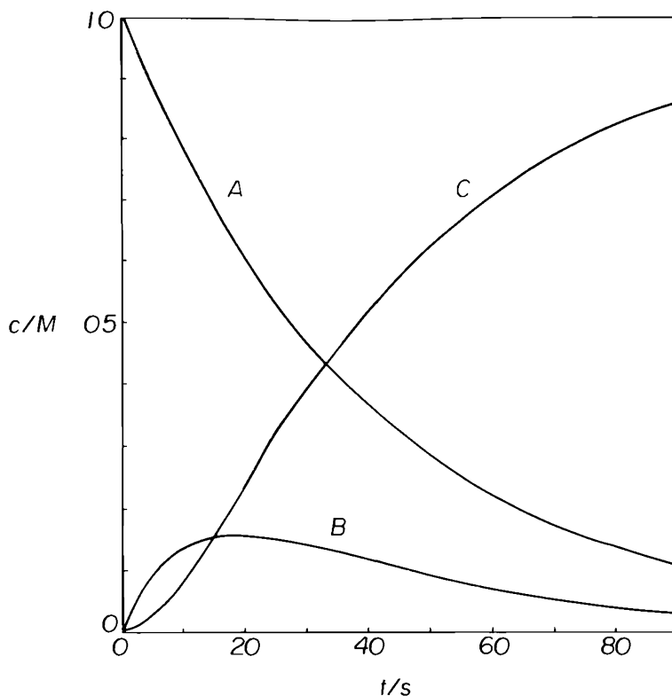
Figure 3-3. Plots of Eqs. (3-24), (3-27), and (3-29) for a system having parameters c_A^0 = 1 , k_1 = 0.025 \text{ s}^{-1} , k_2 = 0.10 \text{ s}^{-1} . Compare with Fig. 3-2.
