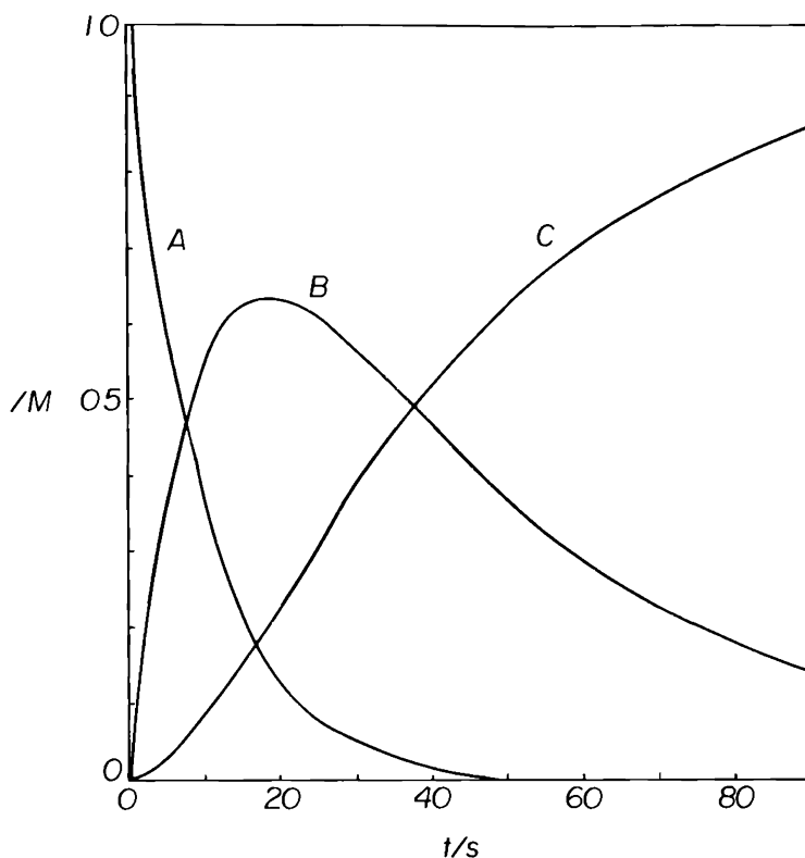
Figure 3-2. Plots of Eqs. (3-24), (3-27), and (3-29) for a hypothetical system having parameters c_A^0 = 1 , k_1 = 0.10 \text{ s}^{-1} , k_2 = 0.025 \text{ s}^{-1} . Compare with Fig. 3-3.
