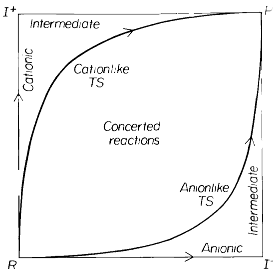
Figure 5-22. Generalized RIP diagram.
