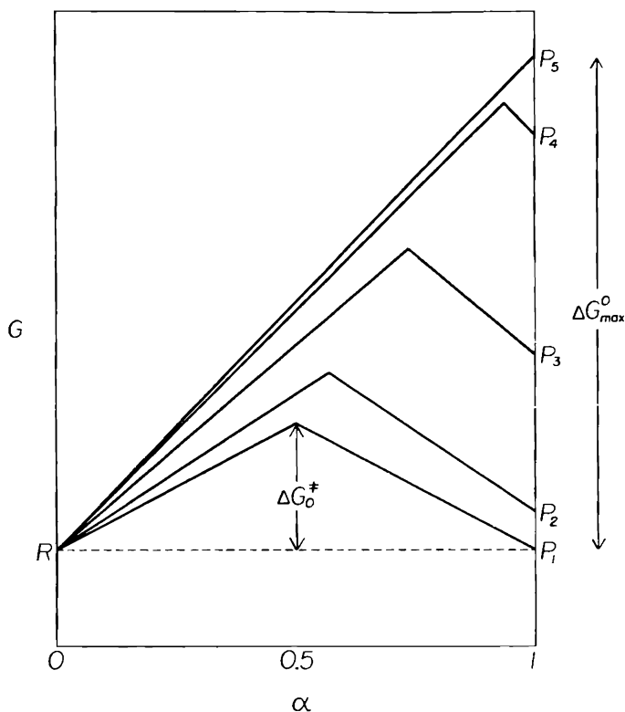
Figure 5-16. Schematic reaction coordinate diagrams of a reaction series, showing \Delta G_0^\ddagger , the intrinsic barrier, and \Delta G_{\max}^0 , the maximum standard free energy difference.
