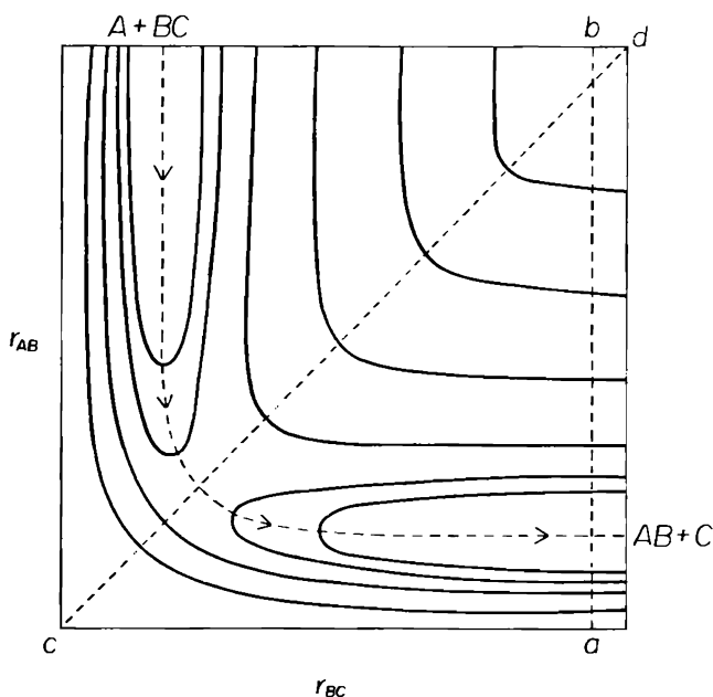
Figure 5-2. A hypothetical potential energy surface for the reaction A + BC \rightarrow AB + C .
