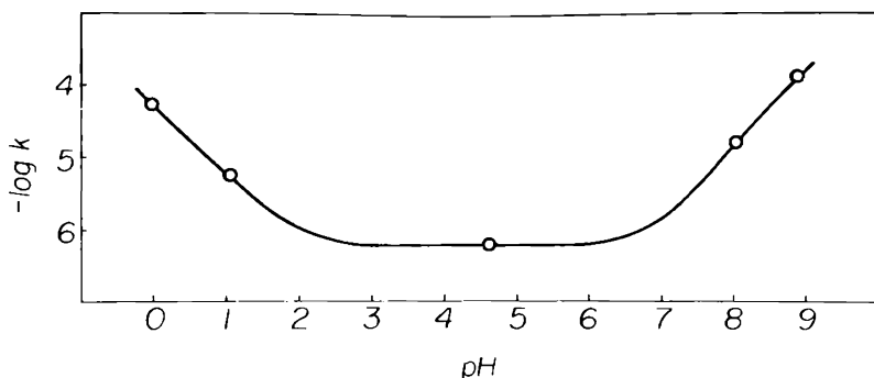
Figure 6-8. pH-rate profile for the hydrolysis of p -nitrophenyl acetate at 25°C in aqueous solution containing 1% acetonitrile. Ionic strength = 0.1 M except at pH 0.
