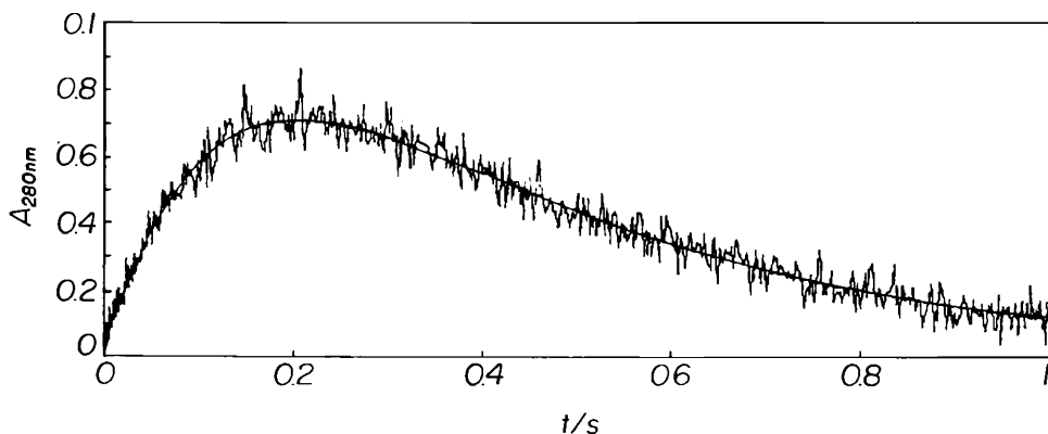
Figure 4-12. Stopped-flow study of the pyridine-catalyzed hydrolysis of acetic anhydride, showing the formation and decay of the acetylpyridinium ion intermediate. Initial concentrations were: 0.087 M pyridine, 2.1 \times 10^{-4} M acetic anhydride; the pH was 5.5; ionic strength, 1.0 M; temperature, 25°C. Five hundred data points (absorbance at 280 nm) were measured in 1 s. The smooth curve is a fit to Eq. (3-27). Source: Data of D. Khosravi and S.-F. Hsu, University of Wisconsin.
