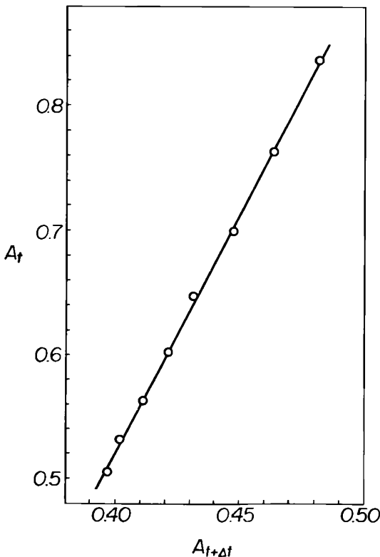
Figure 2-10. Plot of Eq. (2-56) for the hydrolysis of phenyl cinnamate. Data are from Table 2-4.
