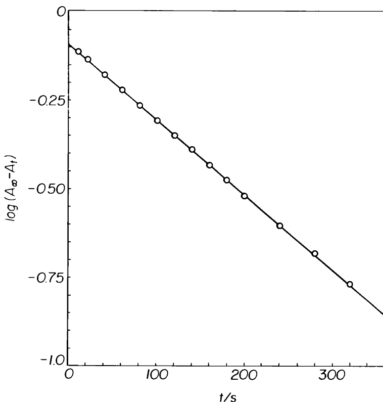
Figure 2-8. First-order plot of the hydrolysis of p -nitrophenyl glutarate at 25°C. Reaction followed spectrophotometrically at 400 nm; b = 1 cm, A_\infty = 0.900 , pH 7.14.
