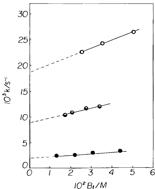
Figure 6-4. Plot of Eq. (6-46) for the hydrolysis of cinnamic anhydride at 25°C and ionic strength 0.1 M in carbonate buffers. B_1 represents the total buffer concentration. From top to bottom, pH = 10.06, 9.76, and 9.14.
