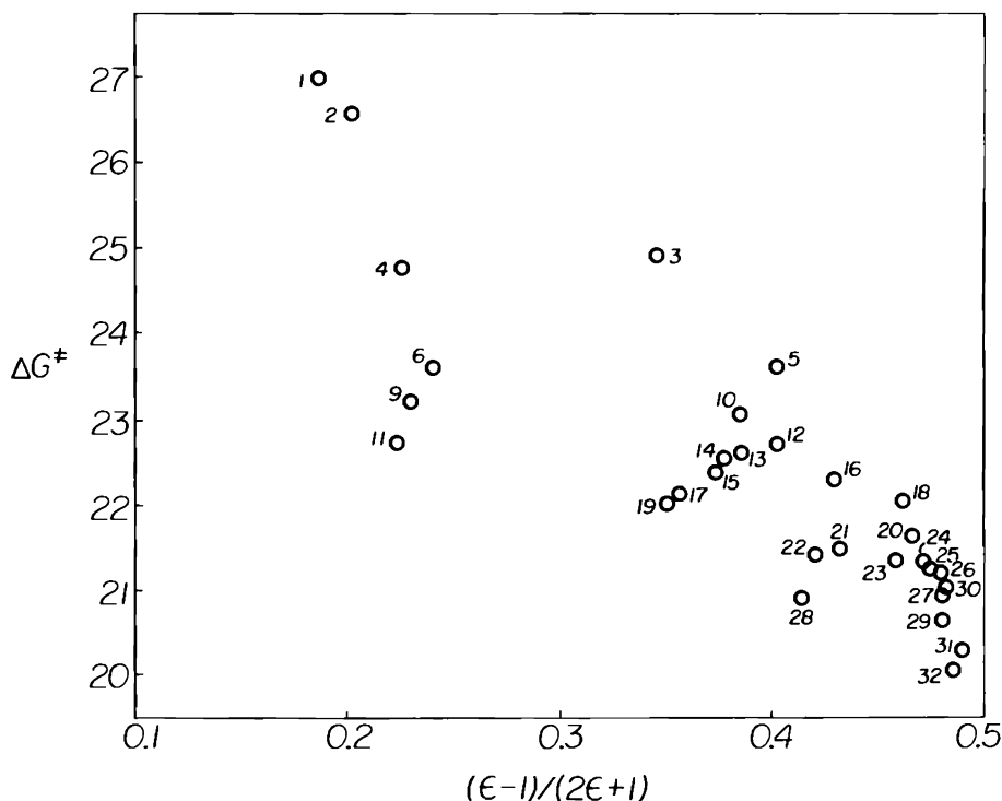
Figure 8-3. Plot of free energy of activation for the Menschutkin reaction \text{Et}_3\text{N} + \text{EtI} \rightarrow \text{Et}_4\text{N}^+ + \text{I}^- against the Kirkwood dielectric constant function. Data are from Table 8-5, where the solvents are identified.
