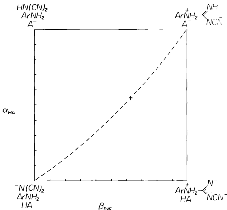
Figure 5-23. RIP diagram for the general acid-catalyzed addition of anilines to dicyanamide.
