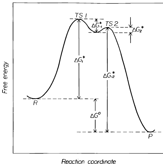
Figure 5-10. Hypothetical free energy reaction coordinate diagram for Scheme II (TS \equiv transition state).
