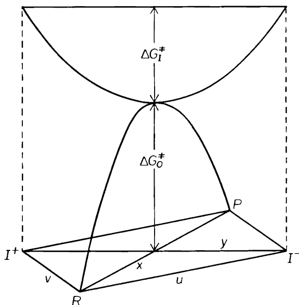
Figure 5-25. Sections through a hyperbolic paraboloid energy surface constructed over an RIP diagram. The intrinsic barrier \Delta G_0^\ddagger of the main reaction and the intrinsic well \Delta G_I^\ddagger of the disparity reaction are shown.
