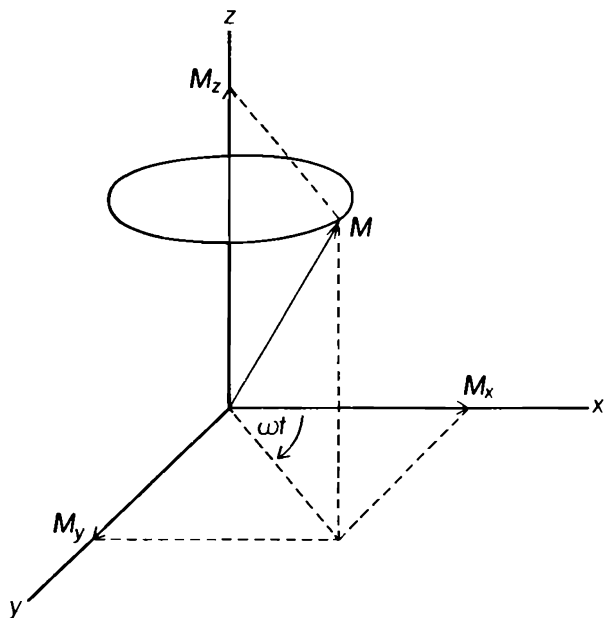
Figure 4-5. Coordinate system for the NMR equation of motion.
