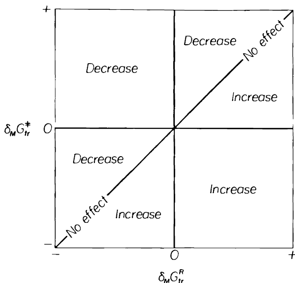
Figure 8-5. Two-dimensional representation of the possible combinations of transfer free energies of reactants (R) and transition state (‡). The words refer to rate increases or decreases relative to the reference solvent, which lies at the origin.
