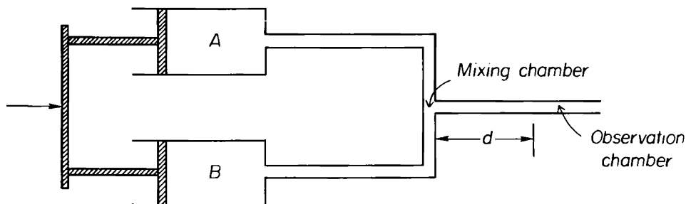
Figure 4-10. Schematic diagram of continuous flow kinetic system. The quantity d is the distance from the mixer to the point of observation.
