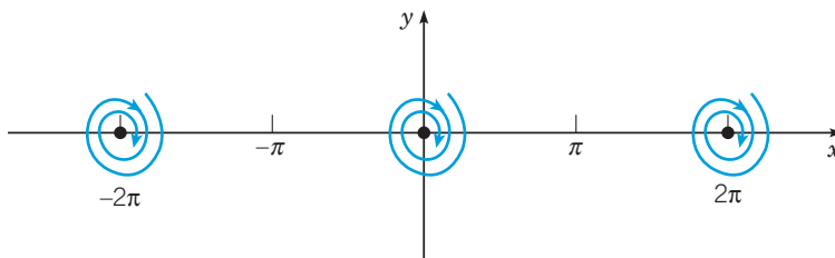
FIGURE 9.3.3 Asymptotically stable spiral points at (\pm 2n\pi, 0) for the damped pendulum with small damping, \gamma^2 - 4\omega^2 < 0 .
