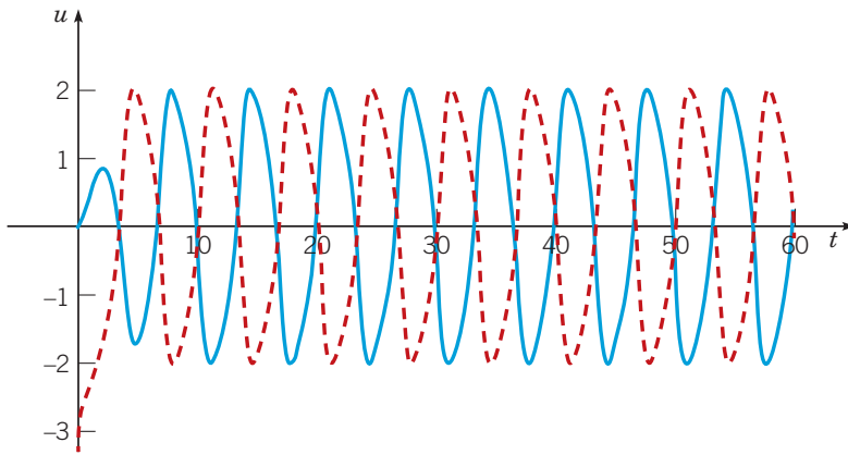
FIGURE 9.7.5 Plots of u versus t for the trajectories in Figure 9.7.4. Note that the waveforms are periodic and completely out of phase.
