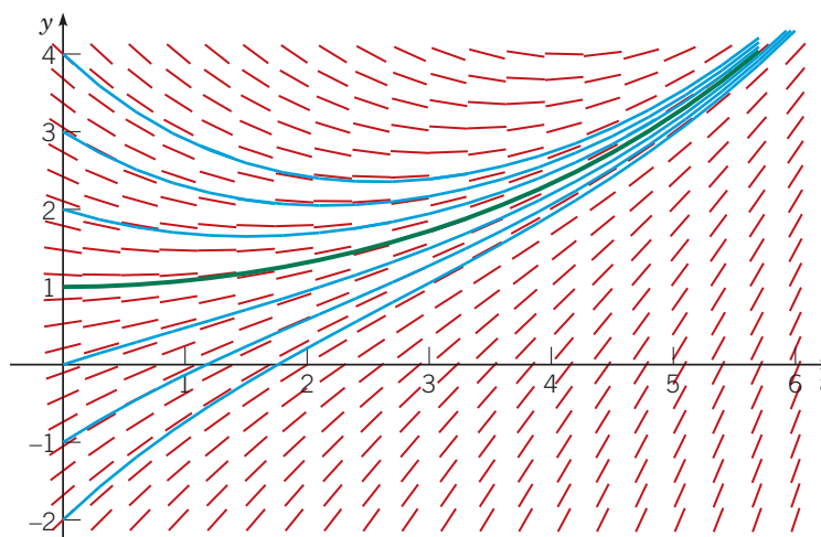
FIGURE 2.1.1 Direction field and integral curves of y' + \frac{1}{2}y = \frac{1}{2}e^{t/3} ; the green curve passes through the point (0, 1) .
