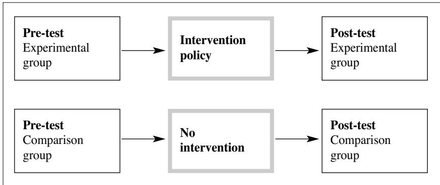
Figure 8.1 Non-equivalent comparison group design
