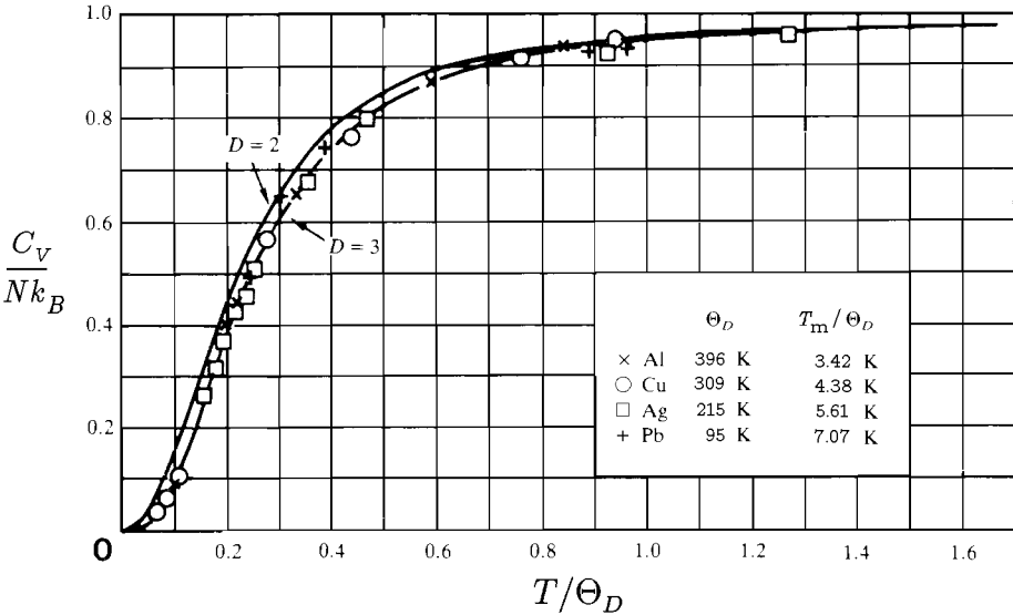
FIGURE 19.2 Specific heat of various solids. By plotting the data against the ratio T/\Theta_D , where \Theta_D is the Debye temperature, the data fall on a universal curve. The insert lists \Theta_D -values and melting temperature T_m .
