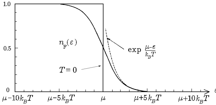
FIGURE 2.2 Average Fermi occupation number n_F(\varepsilon) . Fermions have a positive chemical potential \mu .
