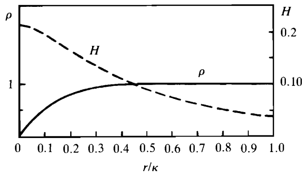
FIGURE 16.2 Order parameter \rho , and the magnetic field h for an n = 1 vortex line in a deep type-II superconductor with K = 10 .
