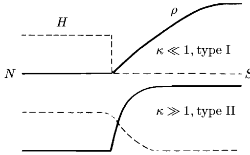
FIGURE 16.1 Dependence of order parameter \rho and magnetic field H on the reduced distance z for a planar domain wall between the normal and superconductive phases. The magnetic field points parallel to the wall.
