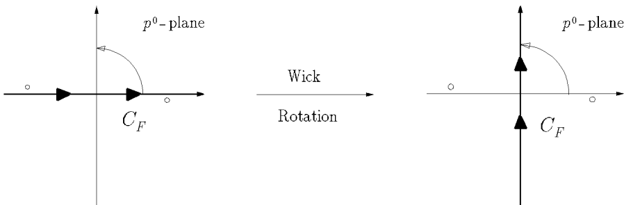
FIGURE 5.2 Wick rotation of the contour of integration in the complex p^0 -plane
