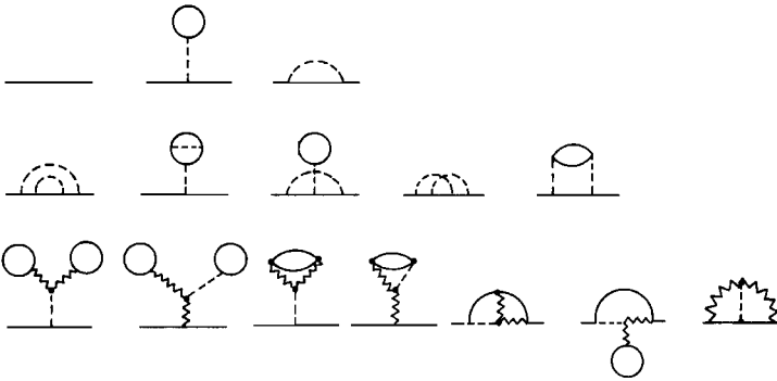
FIGURE 25.1 Two-loop diagrams
