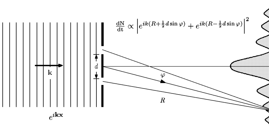
FIGURE 1.1 Probability distribution of particle behind a double slit, being proportional to the absolute square of the sum of the two complex field strengths.
