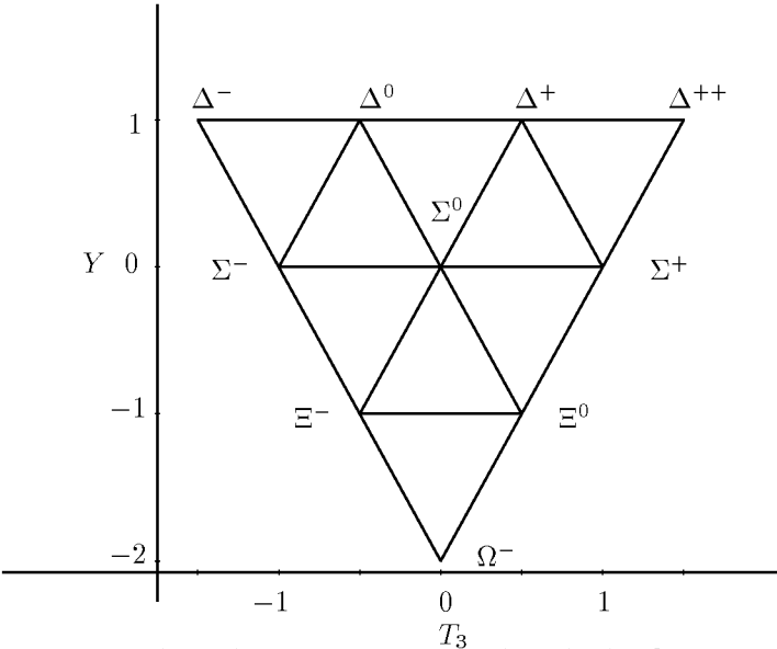
FIGURE 22.8 Baryon decuplet states associated with the first resonance of the nucleons.
