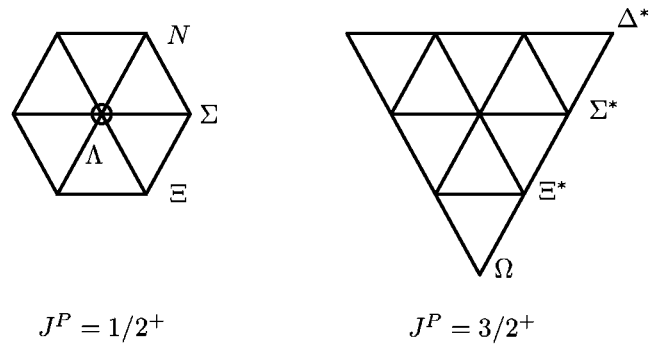
FIGURE 23.3 The SU(3) content of the particles in the 56 representation of SU(6) containing the J^P = 1/2^+ nucleons and the J^P = 3/2^+ resonances.
