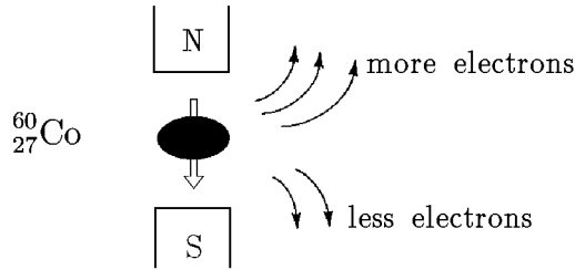
FIGURE 3.2 Asymmetry observed in the distribution of electrons from the \beta -decay of polarized {}^{60}_{27}\text{Co} .
