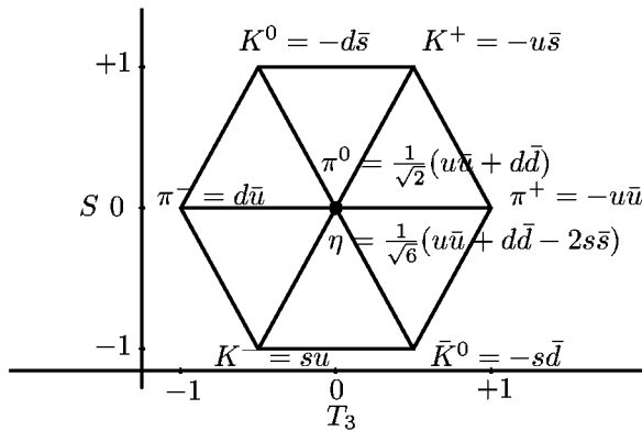
FIGURE 22.13 The quark-antiquark content of the meson octet meson states with de Swart phase convention.
