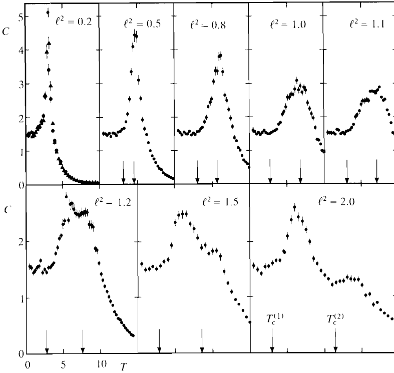
FIGURE 19.6 Separation of first-order melting transition into two successive Kosterlitz-Thouless transitions when increasing the length scale \ell of rotational stiffness of the defect model.
