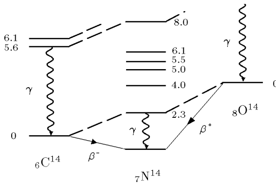
FIGURE 22.5 Singlets and triplets of isospin in the nuclei {}_6\text{C}^{14} , {}_7\text{N}^{14} , {}_8\text{O}^{14} (with the excitation energies in MeV). The dotted lines connect levels are roughly degenerate after subtracting the Coulomb energy according to the estimate (22.9).
