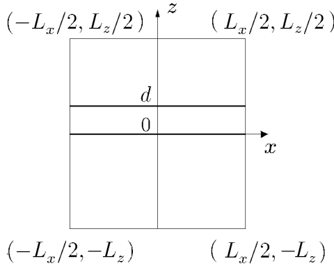
FIGURE 5.5 Geometry of the plates for the calculation of the Casimir effect.
