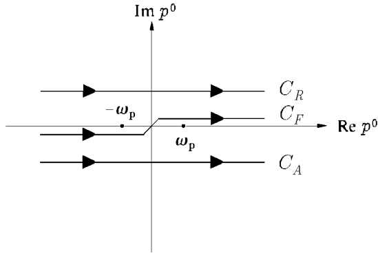
FIGURE 5.3 Integration contours in the complex p^0 -plane of the Fourier integral for the various propagators: C_F for the Feynman propagator, C_R for the retarded and C_A for the advanced propagators.
