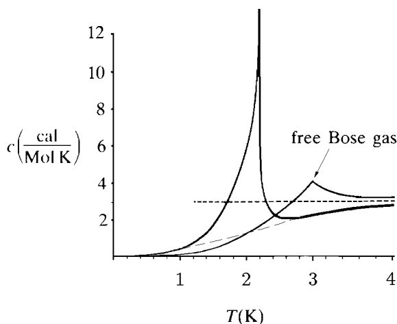
FIGURE 19.1 Specific heat of superfluid ^4\text{He} . The peak is caused by the superfluid-normal transition. A T^3 -behavior is indicated as a dashed curve under the peak.
