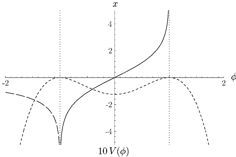
FIGURE 15.5 Classical kink solution (solid curve) in double-well potential (short-dashed curve with units marked on the lower half of the vertical axis). The solution connects the two degenerate maxima in the reversed potential. The long-dashed curve shows a solution which starts out at a maximum and slides down into the adjacent abyss.
