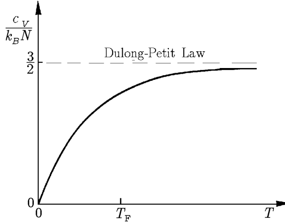
FIGURE 2.3 Temperature behavior of specific heat of a free Fermi gas.
