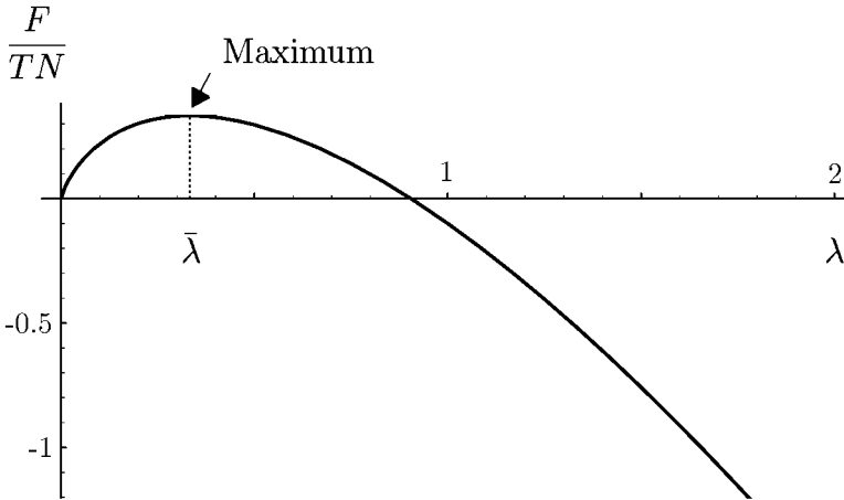
FIGURE 18.1 Free energy as a function of \lambda for D = 2 (schematically). The gap equation determines the position \bar{\lambda} of the maximum.
