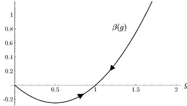
FIGURE 21.2 Flow of the coupling constant g(\sigma) as the scale parameter \sigma approaches zero (infrared limit). For the opposite direction (ultraviolet limit), the arrows are reversed.
