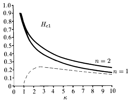
FIGURE 16.3 Critical field h_{c1} at which a vortex line of strength n forms when it first invades a type-II superconductor, as a function of the parameter \kappa . The dotted line indicates the asymptotic result (1/2\kappa) \log \kappa of Eq. (16.168). The magnetic field h_c is measured in units of \sqrt{2}H_c where H_c is the magnetic field at which the magnetic energy equals the condensation energy.
