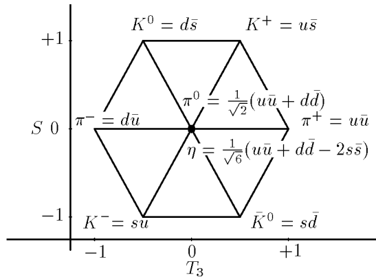
FIGURE 22.9 Quark content of the pseudoscalar meson octet fields. The particle and quark symbols denote the annihilation parts of the corresponding fields.
