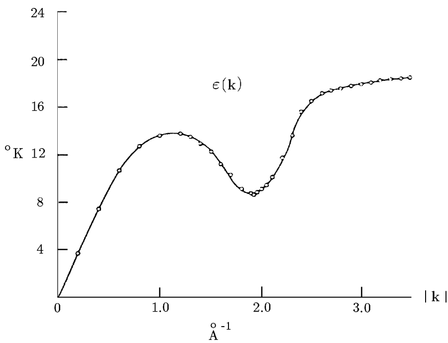
FIGURE 19.3 Energies of the elementary excitations of superfluid ^4\text{He} measured by neutron scattering, showing the excitation energy of the Nambu-Goldstone bosons [after R.A. Cowley and A.D. Woods, Can. J. Phys 49 , 177 (1971)].
