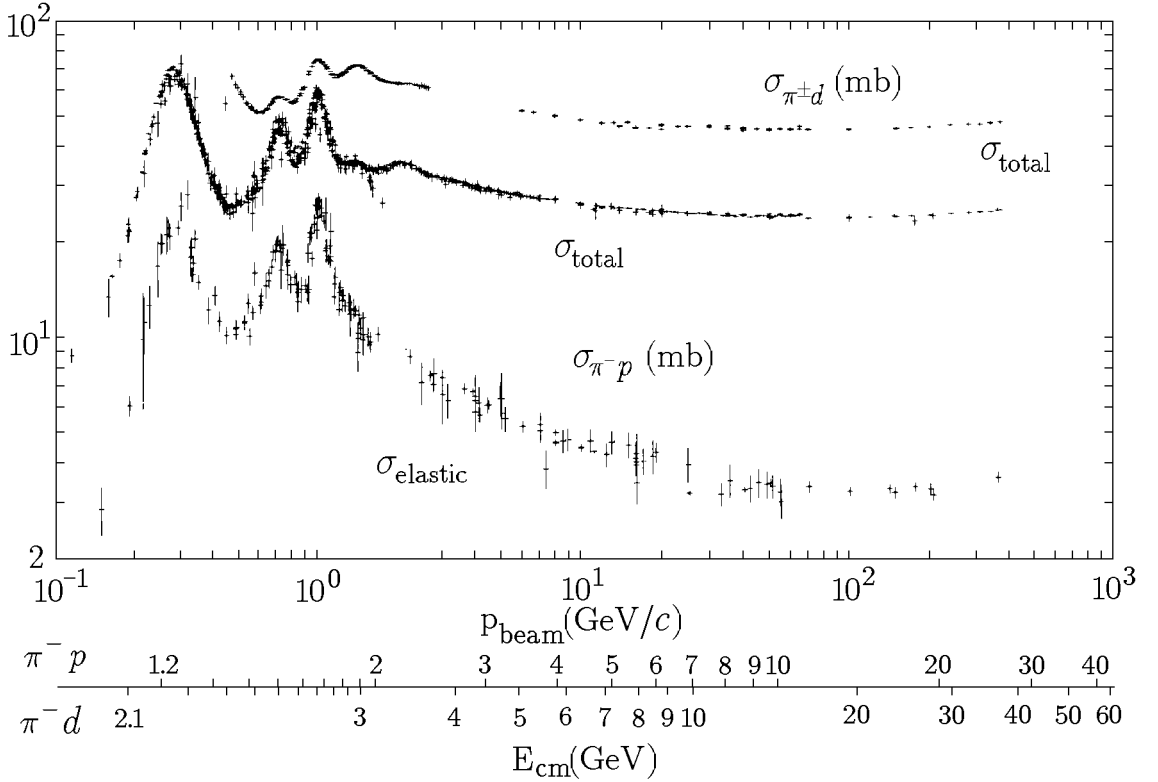
FIGURE 22.2 The total and elastic \pi^- -proton cross section showing again clearly the first nucleon resonance called \Delta(1232) , but with only a third of the height. This is in agreement with the isospin 3/2 assignment and the amplitude relations (22.39) if one invokes the optical theorem, according to which the total cross section is proportional to the imaginary part of the forward scattering amplitude.
