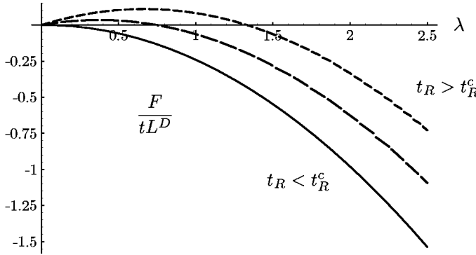
FIGURE 18.2 Free energy as a function of \lambda for D = 2 (schematically). The gap equation determines the position \bar{\lambda} of the maximum.
