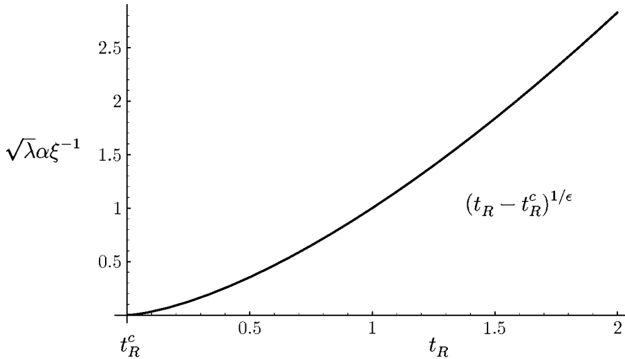
FIGURE 18.4 Temperature behavior of the correlation length.
