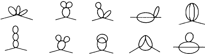
FIGURE 25.2 Three-loop diagrams
