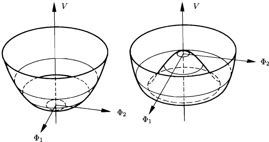
FIGURE 15.1 Effective potential of the \phi^4 -theory for N = 2 in mean-field approximation. for m^2 > 0 and m^2 < 0 , corresponding to temperatures above and below the critical temperature respectively.
