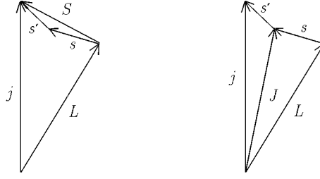
FIGURE 5.4 Different coupling schemes for two-particle states of total angular momentum j and helicity m . The first is the LS , the second the JL scheme.
