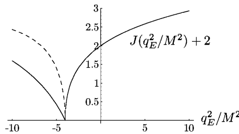
FIGURE 20.2 The function J(z) + 2 in the denominator of the \sigma' -propagator (20.60). For z < -4 , the curve shows the real, the dashed curve the imaginary part.
