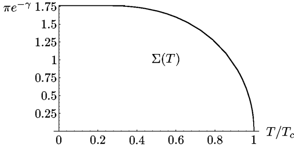
FIGURE 20.4 Solution of the temperature dependent gap equation, showing the decrease of the fermion mass M(T) = \Sigma(T) with increasing temperature T/T_c .
