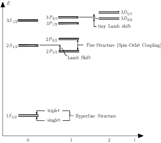
FIGURE 4.1 Hydrogen spectrum according to Dirac's theory. The splittings are shown only schematically. The fine-structure splitting of the 2P -levels is about 10 times as big as the hyperfine splitting and Lamb shift.
