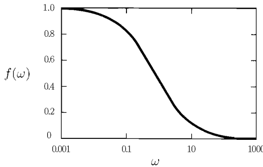
FIGURE 10.8 Ratio between total relativistic Compton cross section and nonrelativistic Thomson cross section.
