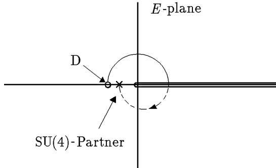
FIGURE 23.1 Pole position of the would-be SU(4) partner of the deuteron with spin-1 and isospin-0. It is close to the D-pole but not a particle since it hides in the complex energy plane just below the two-particle cut.
