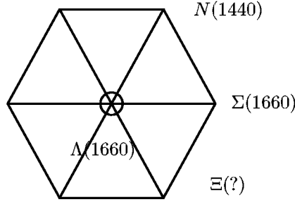
FIGURE 23.5 Octet of spin-parity \frac{1}{2}^+ baryons.
