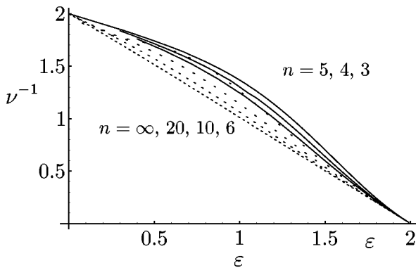
FIGURE 25.12 The highest approximations ( M = 4 ) for n = 3, 4, 5 (counting from the top), and the 1/n -expansions to order 1/n^2 for n = \infty, 20, 10, 6 (counting from the bottom). The sixth-order result is obviously still far from the exact one.
