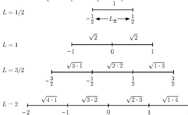
FIGURE 3.3 Effect of raising and lowering operators \hat{L}_+ and \hat{L}_- upon the states |s, m\rangle .
