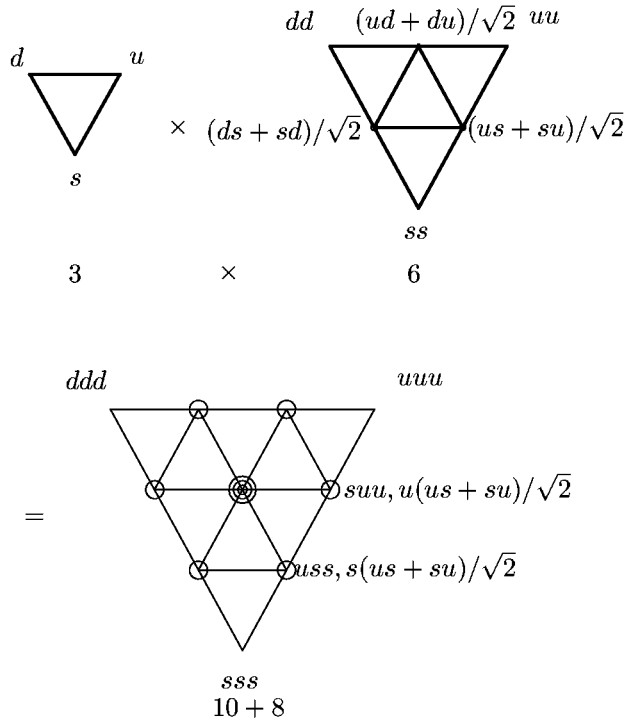
FIGURE 22.17 The irreducible three-quark states 10 and 8 in the product 3 \times 6 (the symbol (\dots)_s denotes complete symmetrization).
