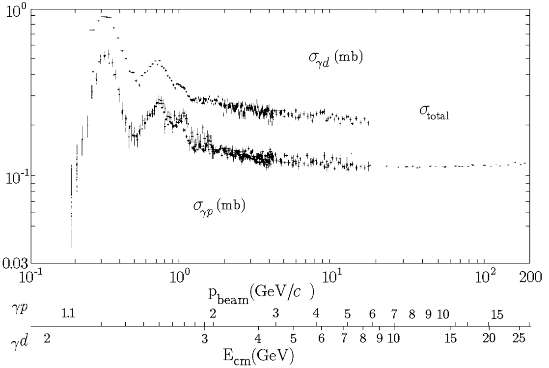
FIGURE 22.3 The photon-proton and photon-deuteron total cross sections showing clearly the first nucleon resonance \Delta(1232) as well as a second resonance called N(1520) .
