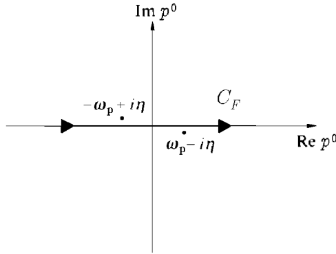
FIGURE 5.1 Pole positions in the complex p^0 -plane in the integral representations (5.63) and (5.83) Feynman propagators.
