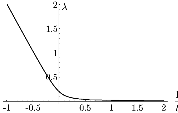
FIGURE 18.3 Solution of the gap equation (18.48) for \epsilon = 1 and large volume L^D . For L \rightarrow \infty , the right-hand part of the curve approaches more and more the abscissa.
