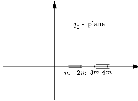
FIGURE 9.1 Singularities in complex q_0 -plane of Feynman propagator. There are poles and cuts due to three- and more-particle intermediate states in the diagram.
