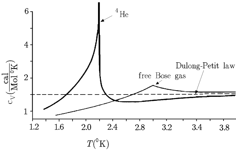
FIGURE 2.6 Temperature behavior of the specific heat of a free boson gas. For comparison we show the specific heat of the strongly interacting Bose liquid ^4\text{He} , scaled down by a factor 2 to match the Dulong-Petit limit of the free Bose gas.
