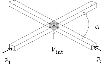
FIGURE 7.1 Geometry of particle beams in a collider. The angle of intersection \alpha is greatly exaggerated. The intersection defines the interaction volume \hat{V}_{\text{int}} .
