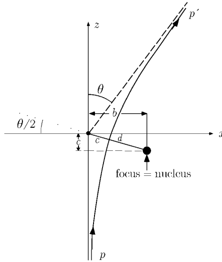
FIGURE 10.5 Kinematics of Rutherford cross section.
