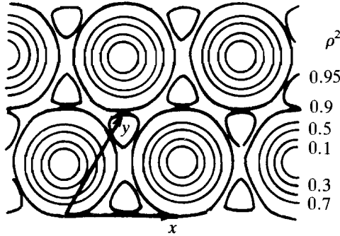
FIGURE 16.4 Spatial distribution magnetization of the order parameter \rho(\mathbf{x}) in a typical mixed state in which the vortex lines form a hexagonal lattice (from W.M. Kleiner et al., See References.)
