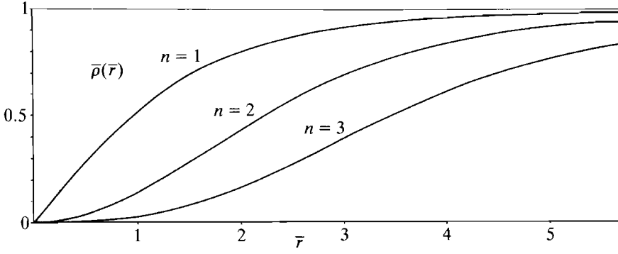
FIGURE 15.7 The order parameter \bar{\rho} = |\varphi|/|\varphi_0| around a vortex line of strength n = 1, 2, 3, \dots as a function of the reduced distance \bar{r} = r/\xi where r is the distance from the axis and \xi the healing length.
