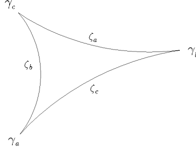
FIGURE 3.4 Triangle formed by rapidities in a hyperbolic space. The sum of angles is smaller than 180^\circ . The angular defect yields the angle of Thomas precession.
