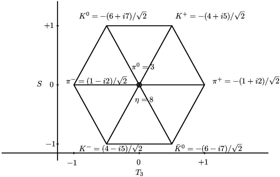
FIGURE 22.14 Combination of indices a in the pseudoscalar octet field M_a^\dagger of (22.99). Here -(1 \pm i2)/\sqrt{2} stands for -(M_1^\dagger \pm iM_2^\dagger)/\sqrt{2} .
