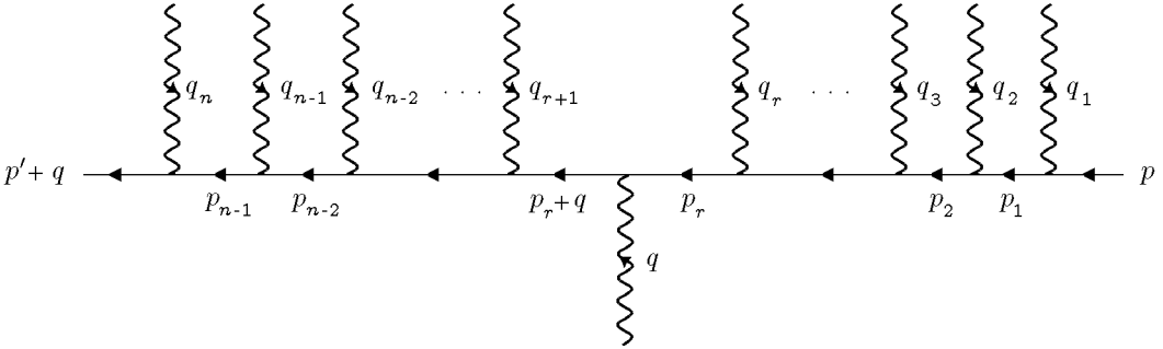
FIGURE 10.2 An electron on the mass shell absorbing several photons, plus an additional photon, and leaving again on the mass shell.
