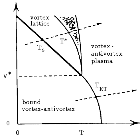
FIGURE 19.4 Phase diagram of a two-dimensional layer of superfluid ^4\text{He} . At a higher fugacity y > y^* , an increase in temperature causes the vortices to first condense to a lattice and to undergo a Kosterlitz-Thouless vortex unbinding transition only after a melting transition.
