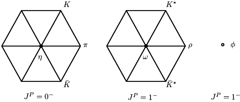
FIGURE 23.2 The pseudoscalar and vector mesons of the 35 representation of SU(6).
