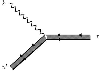
FIGURE 10.4 Transition of an atomic state from a state n with energy E_n to a lower state n' with energy E_{n'} , thereby emitting a photon with a frequency \omega = (E_{n'} - E_n)/\hbar
