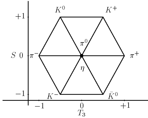
FIGURE 22.6 Pseudoscalar meson octet states associated with the pions. The same picture holds for the vector meson octet states with the replacement (22.58).
