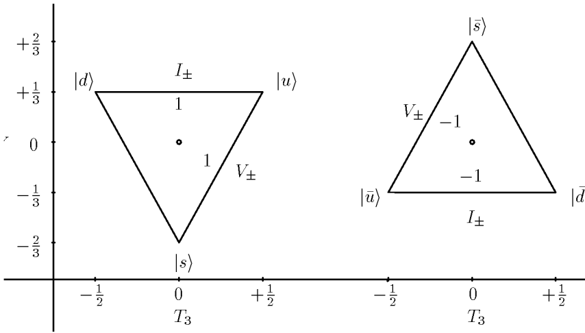
FIGURE 22.10 Effect of raising and lowering operators on quark and antiquark states. Here and in the subsequent weight diagrams the ket symbols of the states are omitted.
