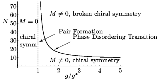
FIGURE 20.3 The two transition lines in the N - g -plane of the chiral Gross-Neveu model in 2 + \epsilon dimensions. For \epsilon = 0 , the vertical transition line coincides with the N -axis, and the solid hyperbola degenerates into a horizontal line at N_c = 8 . The quark masses and chiral properties are indicated.
