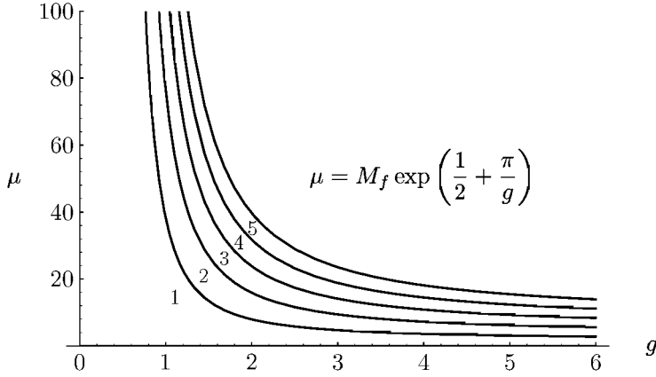
FIGURE 21.1 Curves in the (\mu, g) -plane corresponding to the same physical fermion mass M_f = 1, \dots, 5 , and thus to identical physical observables. These curves are the renormalization group trajectories of the O(N) -symmetric four-fermion model in the limit N \rightarrow \infty .
