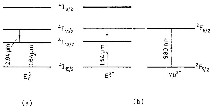
FIG. 9.4. Relevant energy level diagram of: (a) Er:YAG; (b) Yb:Er:phosphate-glass.
