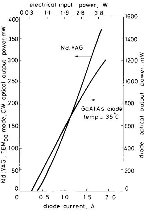
FIG. 7.13. Output power vs diode current for the Nd:YAG laser of Fig. 7.12. In the same figure the output power vs current of the laser diode array is also shown (after ref., (15) by permission).
