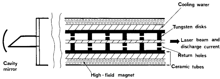
FIG. 10.7. Schematic diagram of a high-power water-cooled \text{Ar}^+ laser tube.
