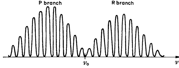
FIG. 3.7. Transitions between two vibrational levels, taking account of the rotational splitting. This transition, which, in the absence of rotational energy, would consist of a single line centered at \nu_0 , actually consists of two groups of lines: the so-called P – branch, which corresponds to a jump in rotational quantum number of \Delta J = +1 and the so-called R – branch, which corresponds to a jump in rotational quantum number of \Delta J = -1 .
