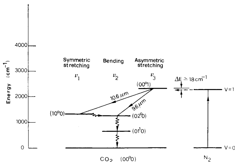
FIG. 10.9. The lowest vibrational levels of the ground electronic state of a CO 2 molecule and a N 2 molecule (for simplicity, the rotational levels are not shown).
