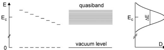
Fig. 18.6 Quasiband model of excited-impurity quasiparticles
