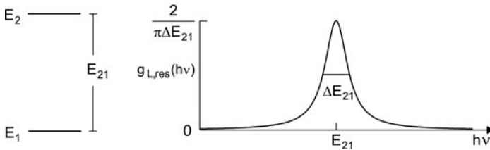
Fig. 4.10 Lorentz resonance function on the energy scale
