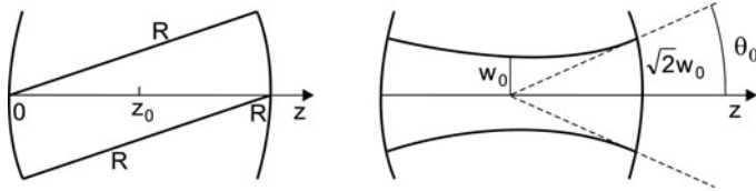
Fig. 11.4 Confocal resonator
