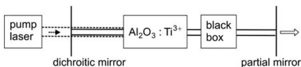
Fig. 5.2 Titanium–sapphire laser
