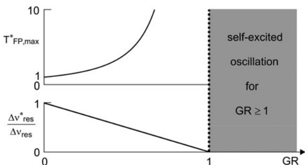
Fig. 3.5 Fabry–Perot resonator containing an active medium
