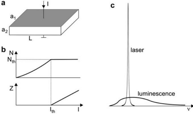
Fig. 21.6 Bipolar laser diode. (a) Device. (b) Dependence of the electron density and the photon density on the current. (c) Laser and luminescence radiation
