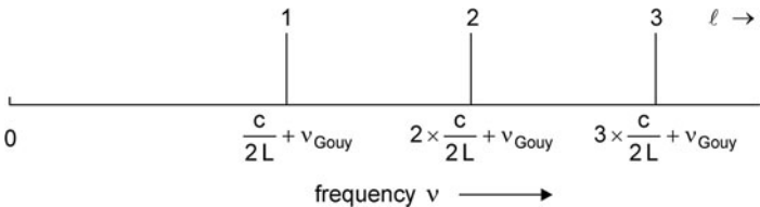
Fig. 11.13 Low-order resonance frequencies of an open resonator
