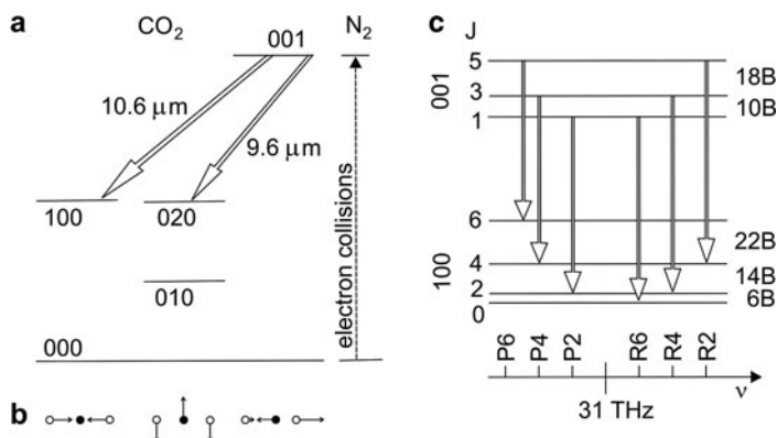
Fig. 14.9 CO 2 laser. (a) Vibrational levels of CO 2 and N 2 . (b) Vibrations of the CO 2 molecule. (c) Vibrational-rotational transitions in CO 2
