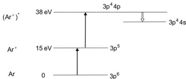
Fig. 14.6 Argon ion laser
