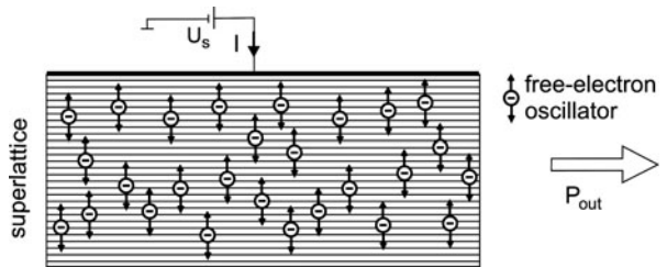
Fig. 32.1 Principle of a superlattice Bloch laser
