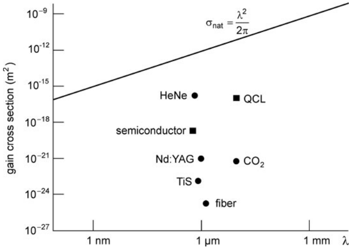
Fig. 7.3 Gain cross sections
