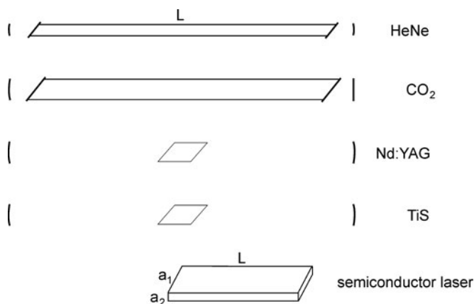
Fig. 2.15 Various lasers
