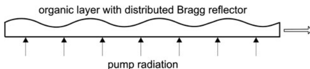
Fig. 34.5 Organic laser ( arrangement )
