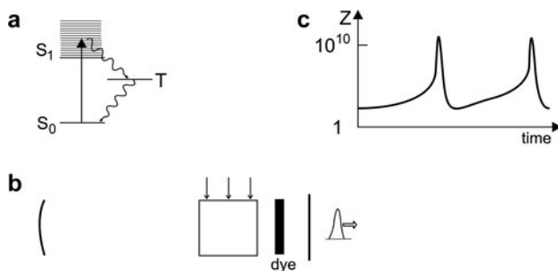
Fig. 12.5 Q-switching with a saturable absorber. (a) Saturation process for dye molecules. (b) Arrangement. (c) Photon density in the laser resonator
