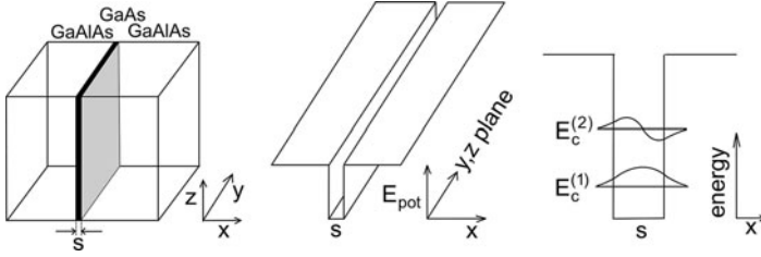
Fig. 26.1 Quantum well
