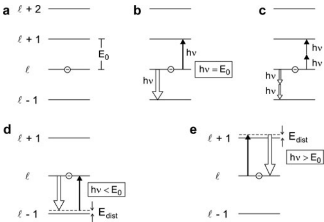
Fig. 32.12 Energy levels of an electron in a superlattice submitted to a static field and optical transitions. (a) Energy ladder. (b) Absorption and stimulated emission. (c) Two-photon transitions. (d) Stimulated emission. (e) Absorption
