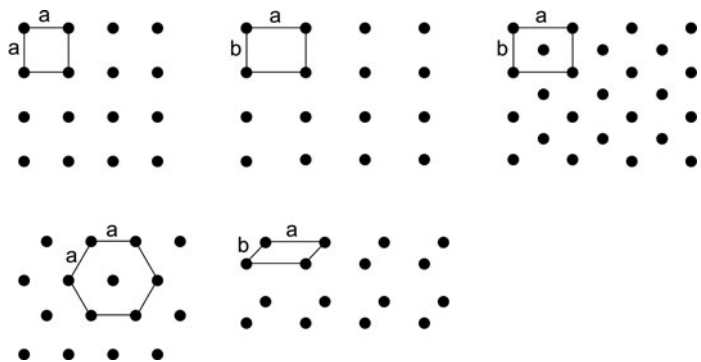
Fig. 25.5 Elementary cells of 2D photonic crystals
