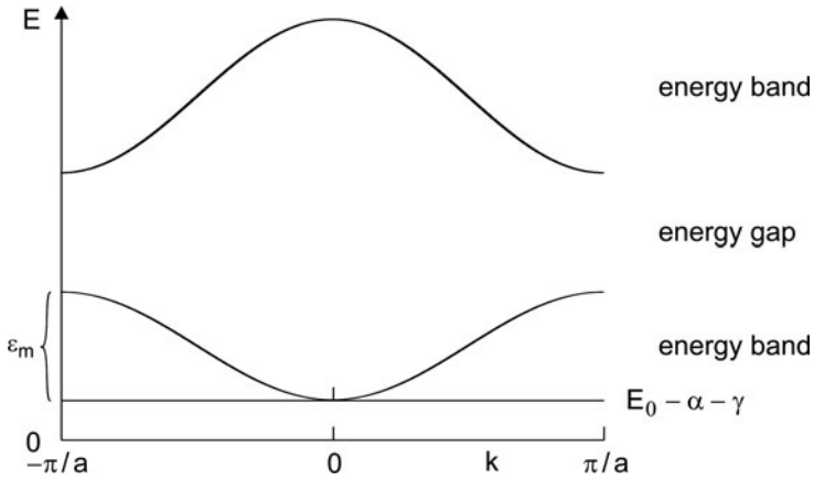
Fig. 30.3 Energy bands
