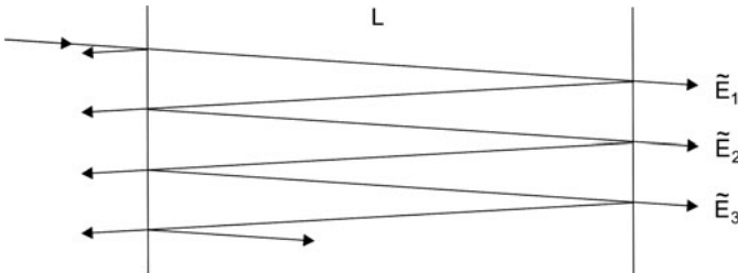
Fig. 3.3 Fabry–Perot interferometer
