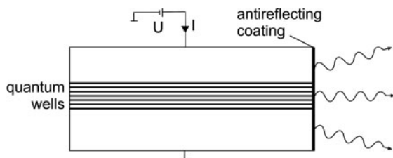
Fig. 34.1 Superluminescent LED
