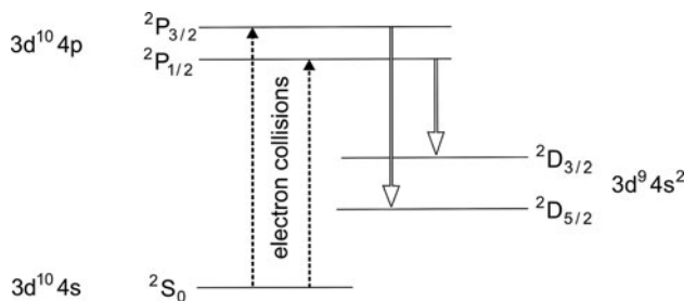
Fig. 14.5 Copper vapor laser
