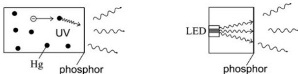
Fig. 34.2 Energy-saving lamp and LED based white light source
