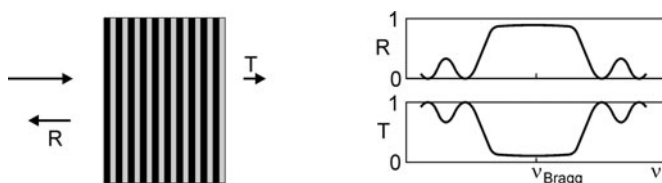
Fig. 25.3 Bragg reflector
