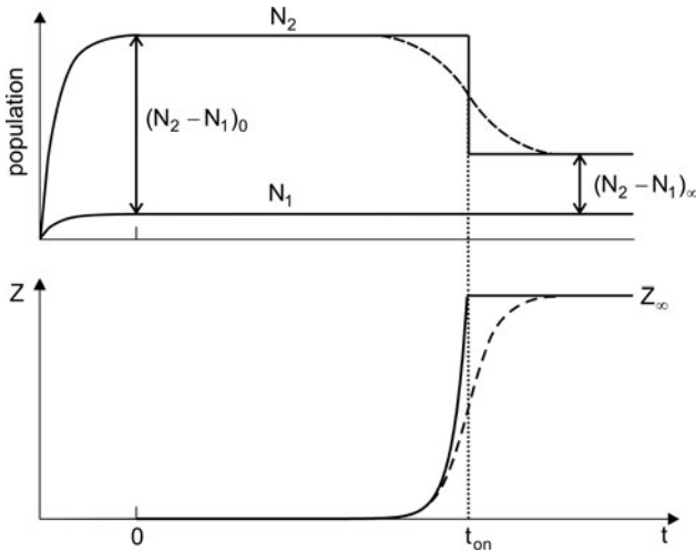
Fig. 8.3 Onset of laser oscillation
