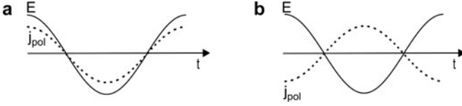
Fig. 9.5 Polarization current and field at resonance (a) in a nonactive medium and (b) for an active medium
