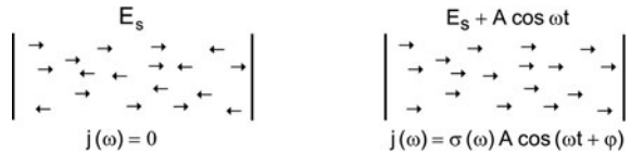
Fig. 32.10 Bloch oscillations of miniband electrons under the action of a static field (left), and of both a static and a high frequency field (right)
