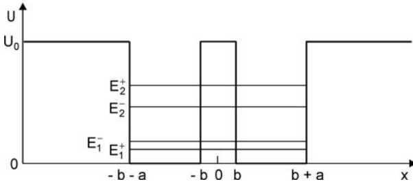
Fig. 30.6 Double-well potential
