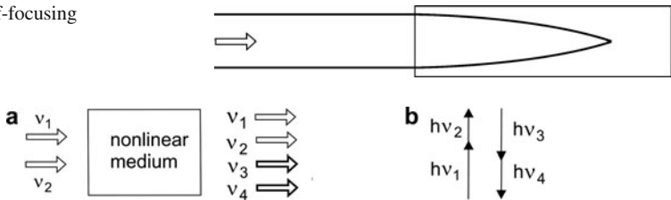
Fig. 35.7 Four-wave mixing. (a) Principle. (b) Elementary process
