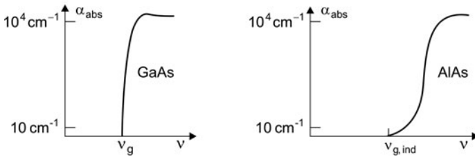
Fig. 23.6 Absorption coefficients of GaAs and AlAs
