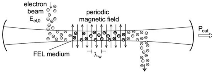
Fig. 19.1 Free-electron laser
