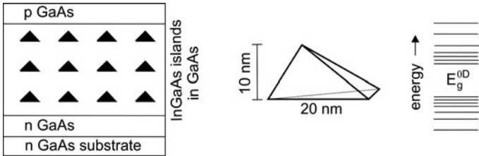
Fig. 27.4 Quantum dot
