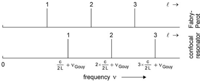
Fig. 11.5 Resonance frequencies
