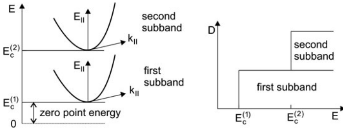
Fig. 26.3 Subbands of electrons in a quantum film
