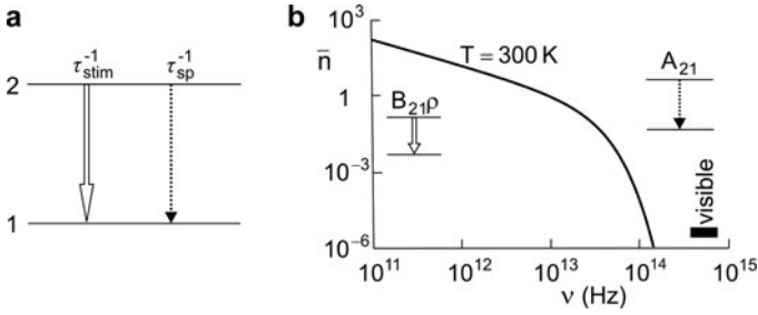
Fig. 6.7 Stimulated and spontaneous emission of radiation. (a) The two processes and (b) regions of their dominance
