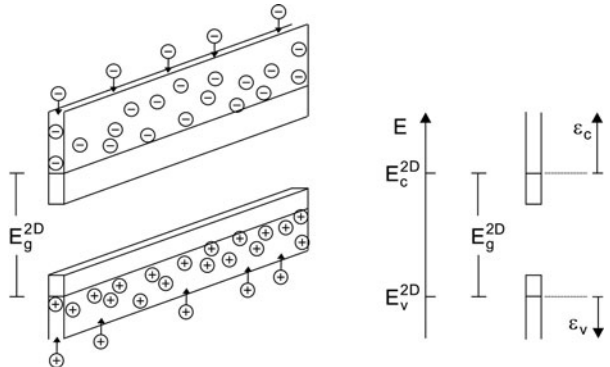
Fig. 22.2 An active quantum well and energy scales
