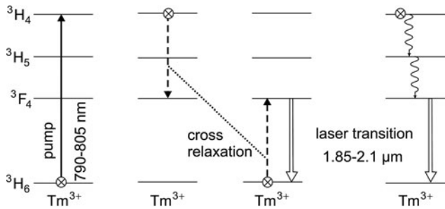
Fig. 15.11 2- \mu\text{m} thulium-doped fiber laser
