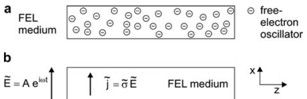
Fig. 19.8 Response of a free-electron laser medium to a high frequency field. (a) Free-electron laser medium: ensemble of free-electron oscillators. (b) Field and current density
