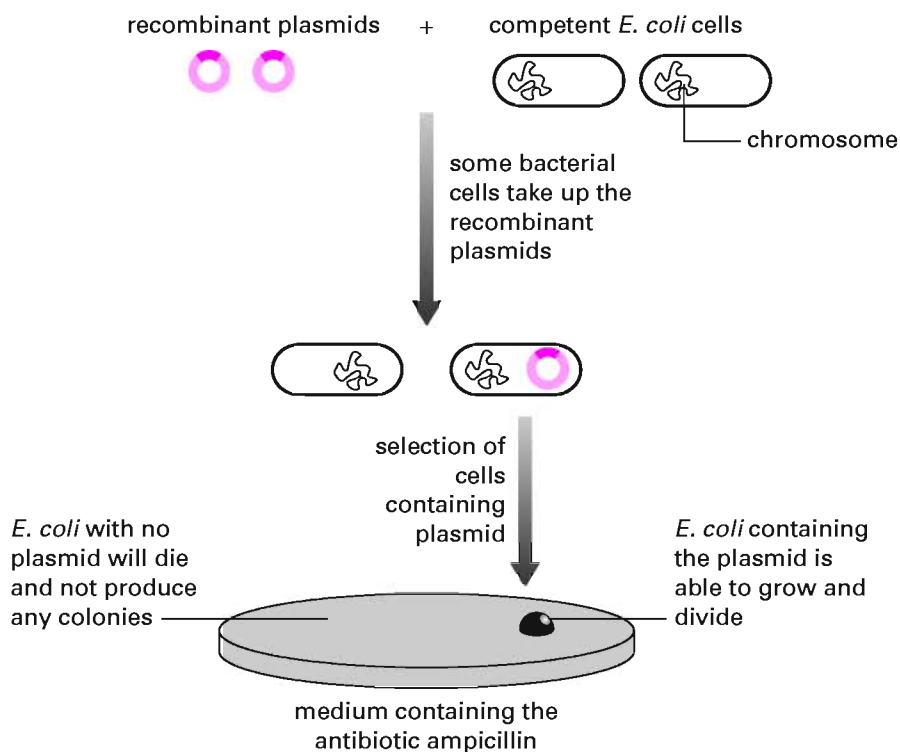
Figure 7.6. Introduction of recombinant plasmids into bacteria.
