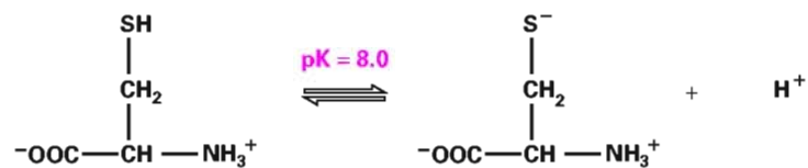
Figure 9.4. Histidine and cysteine.
