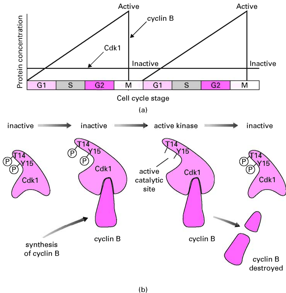
Figure 19.8. Control of Cdk1 by cyclin B and by phosphorylation.
