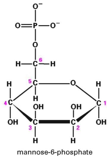
Figure 2.11. Deoxyribose, N -acetyl glucosamine and mannose-6-phosphate are modified sugars.
