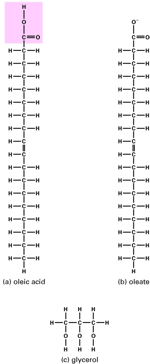
Figure 2.18. Oleic acid and glycerol.
