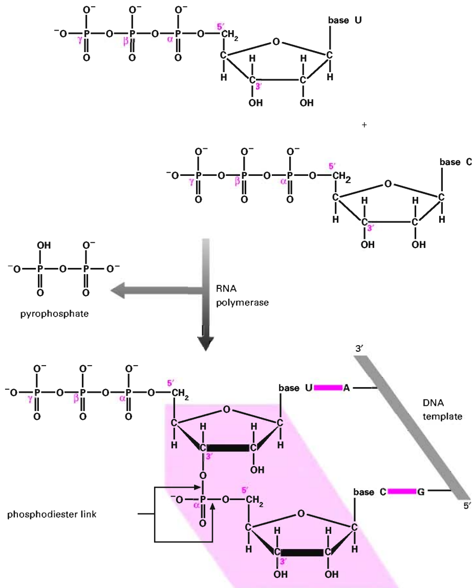
Figure 6.2. Synthesis of an RNA strand.
