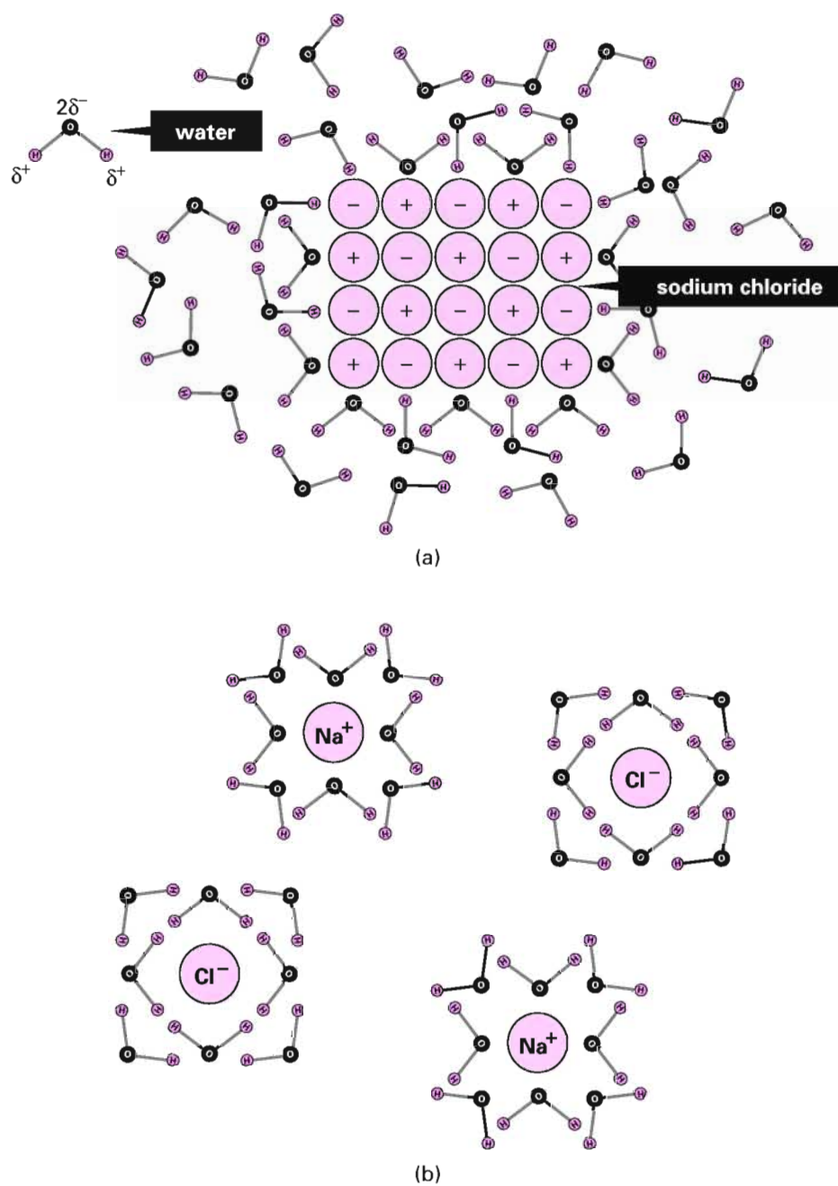
Figure 2.4. Ionic compounds dissolve readily in water.
