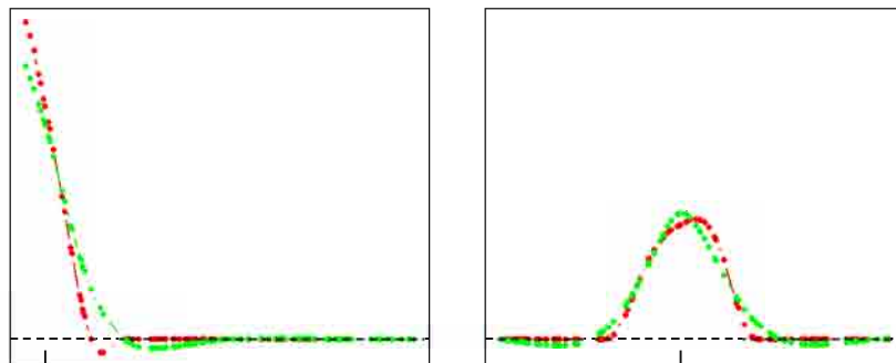
FIGURE 6.7. Equivalent kernels for a local linear regression smoother (tri-cube kernel; red) and a smoothing spline (green), with matching degrees of freedom. The vertical spikes indicate the target points.
