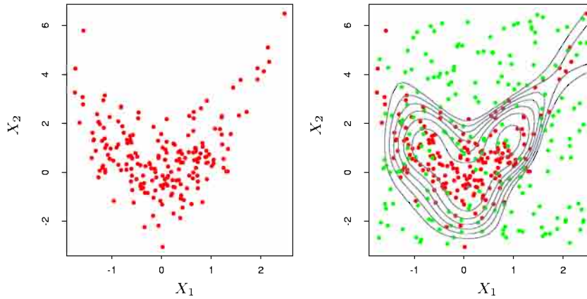
FIGURE 14.3. Density estimation via classification. Left panel: Training set of 200 data points. Right panel: Training set plus 200 reference data points, generated uniformly over the rectangle containing the training data. The training sample was labeled as class 1, and the reference sample class 0, and a semiparametric logistic regression model was fit to the data. Some contours for \hat{g}(x) are shown.
