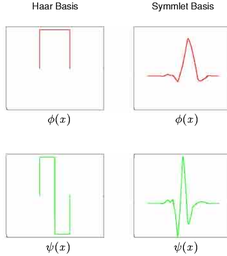
FIGURE 5.15. The Haar and symmlet father (scaling) wavelet \phi(x) and mother wavelet \psi(x) .
