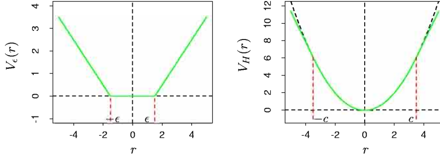
FIGURE 12.6. The left panel shows the \epsilon -insensitive error function used by the support vector regression machine. The right panel shows the error function used in Huber's robust regression (green curve). Beyond |c| , the function changes from quadratic to linear.
