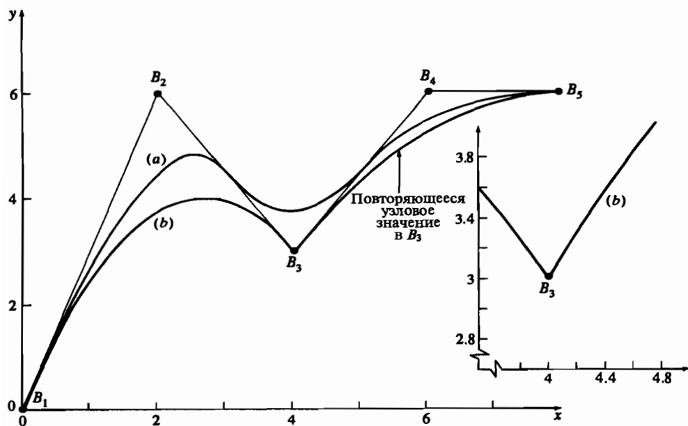
Рис. 5-49 Неравные В-сплайны, k=3 . (a) [X] = [0 \ 0 \ 0 \ 1 \ 2 \ 3 \ 3 \ 3] ; (b) [X] = [0 \ 0 \ 0 \ 1 \ 1 \ 3 \ 3 \ 3] .
