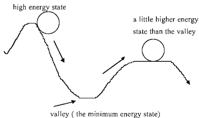
Fig. 4.6: A rolling ball passes through a valley to a higher energy state.
