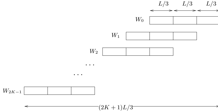
Figure 2: Illustrating forming the product W = UV .
