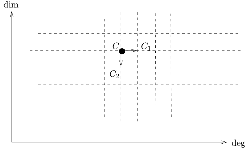
Figure 4: Shifting a cone.
