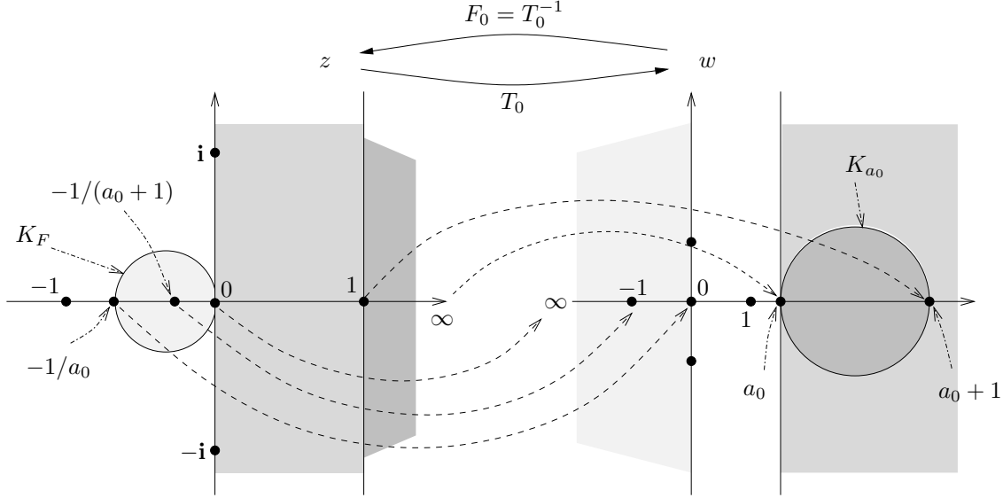
Figure 3: Transformation T_0 : z \mapsto (a_0 z + 1)/z .
