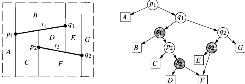
Figure 6.6 The trapezoidal map of two segments and a search structure
