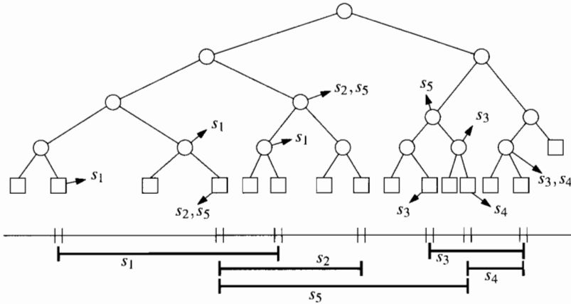
Figure 10.9 A segment tree: the arrows from the nodes point to their canonical subsets.
