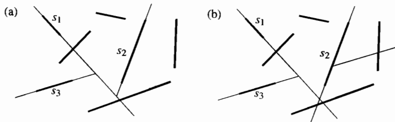
Figure 12.6 The original and the modified algorithm
