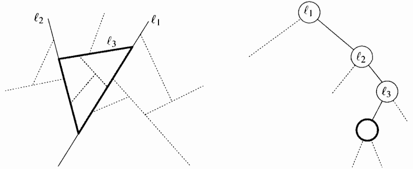
Figure 12.4 The correspondence between nodes and regions
