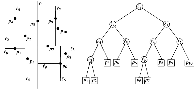
Figure 5.3 A kd-tree: on the left the way the plane is subdivided and on the right the corresponding binary tree
