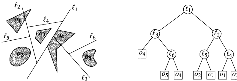
Figure 12.3 A binary space partition and the corresponding tree
