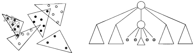
Figure 16.4 A simplicial partition and the corresponding tree
