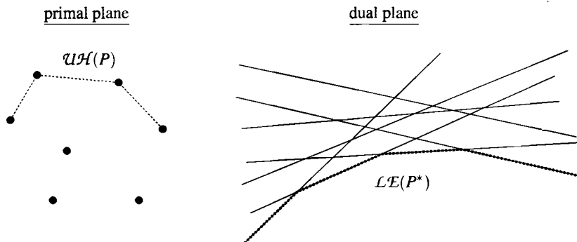
Figure 11.4 Upper hulls correspond to lower envelopes.
