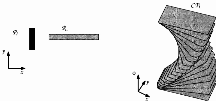
Figure 13.10 The C -obstacle of a rotating and translating robot
