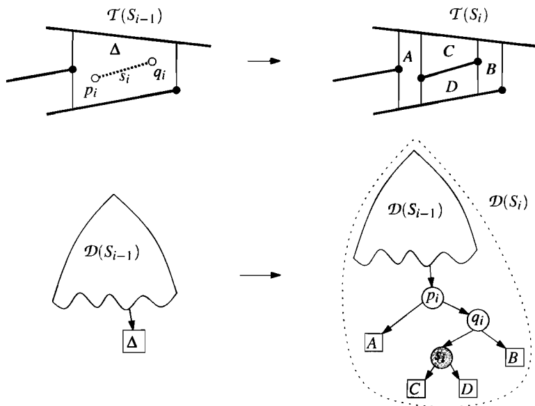
Figure 6.7 The new segment s_i lies completely in trapezoid \Delta .
