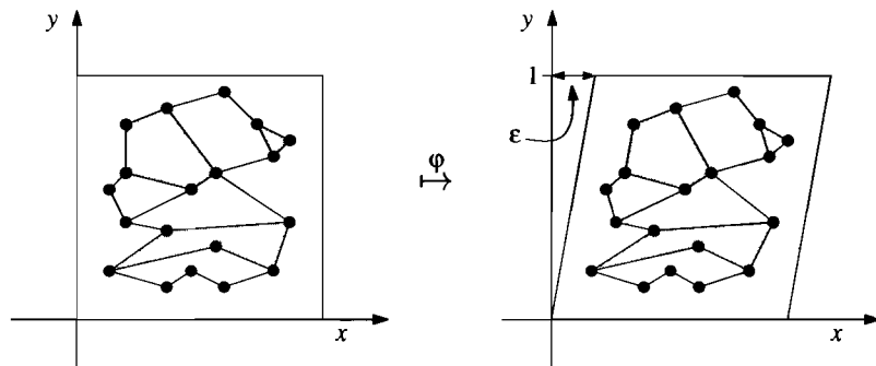
Figure 6.9 The shear transformation
