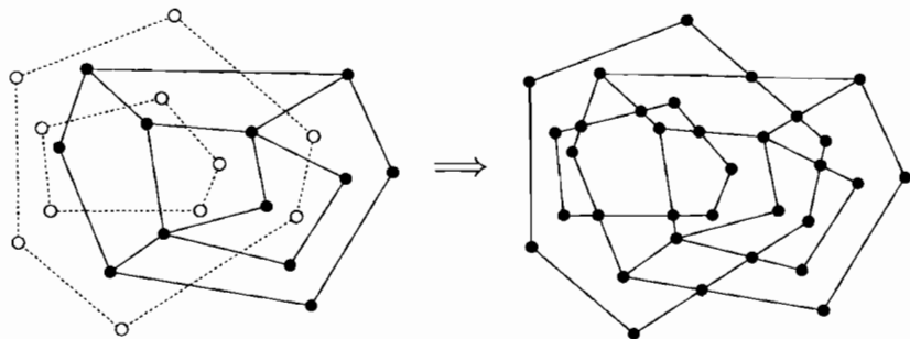
Figure 2.4 Overlaying two subdivisions
