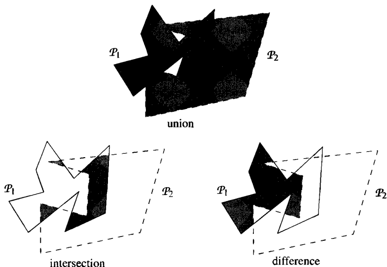
Figure 2.7 The Boolean operations union, intersection and difference on two polygons \mathcal{P}_1 and \mathcal{P}_2
