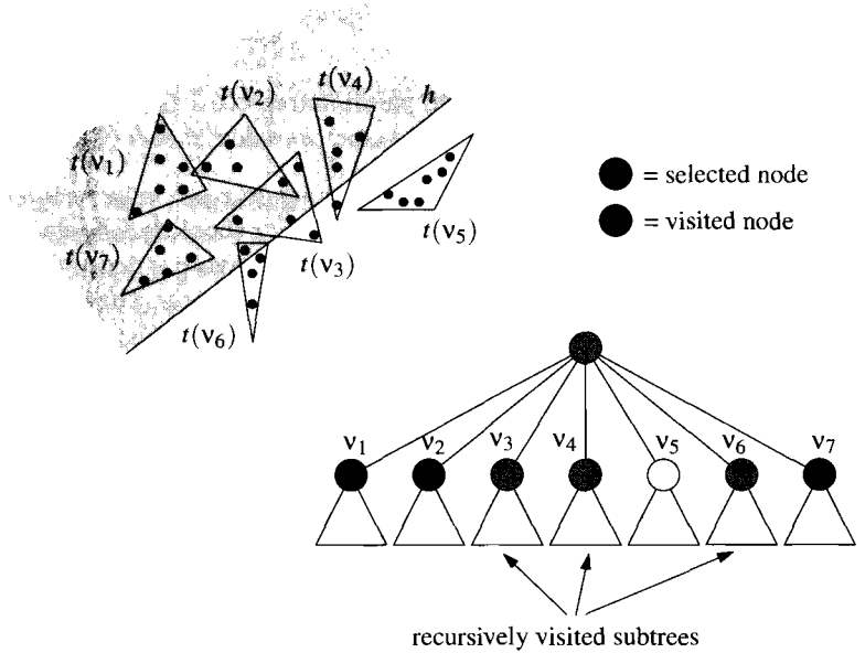
Figure 16.5 Answering a half-plane range query using a partition tree
