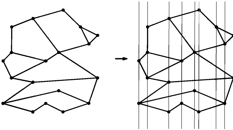
Figure 6.2 Partition into slabs
