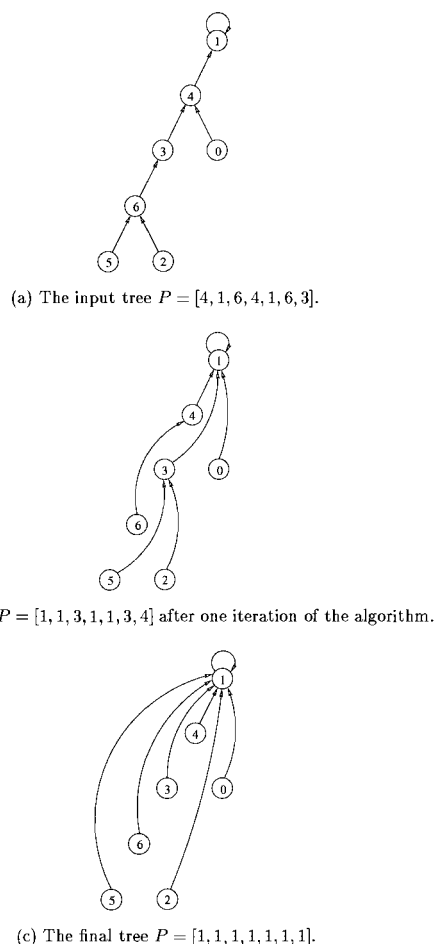
FIGURE 47.5 The effect of two iterations of algorithm POINT_TO_ROOT.
