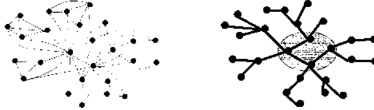
FIGURE 34.1 On the left is an example input graph G . On the right is a spanning tree T that might be found by the approximation algorithm. The shaded circle indicates the nodes in the witness set S .
