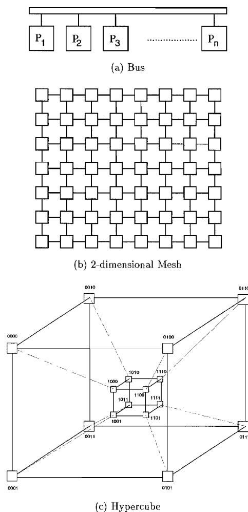
FIGURE 47.2 Bus, mesh, and hypercube network topologies.
