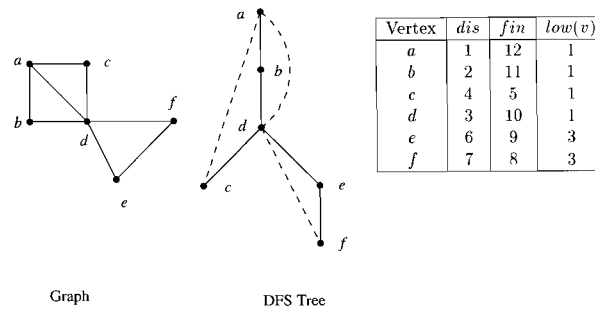
FIGURE 6.2 Identifying cut vertices.
