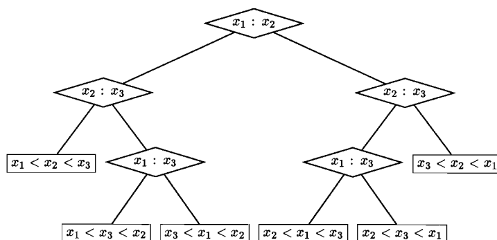
FIGURE 1.4 A decision tree for sorting the three elements x_1 , x_2 , and x_3 .
