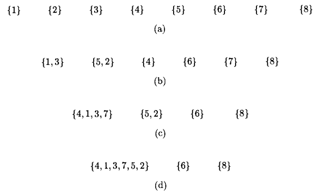
FIGURE 5.1 Examples of set union operations. (a) The initial collection of disjoint sets. (b) The disjoint sets of (a) after performing union (1, 3) and union (5, 2). (c) The disjoint sets of (b) after performing union (1, 7) followed by union (4, 1). (d) The disjoint sets of (c) after performing union (4, 5).
