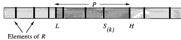
FIGURE 15.1 The LazySelect algorithm.
