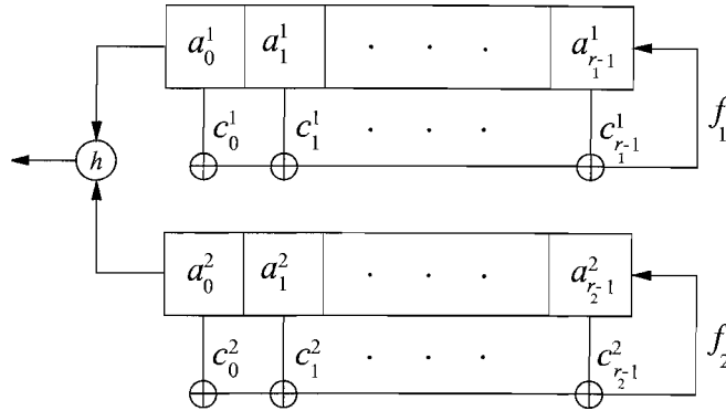
FIGURE 43.4 Nonlinear combiner.
