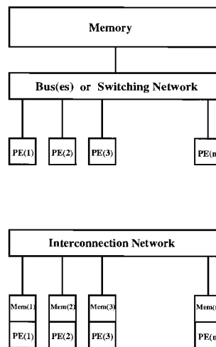
FIGURE 46.1 Shared memory (top) and distributed memory (bottom) machines. ( PE is used to represent a processing element and Mem is used to represent memory.)
