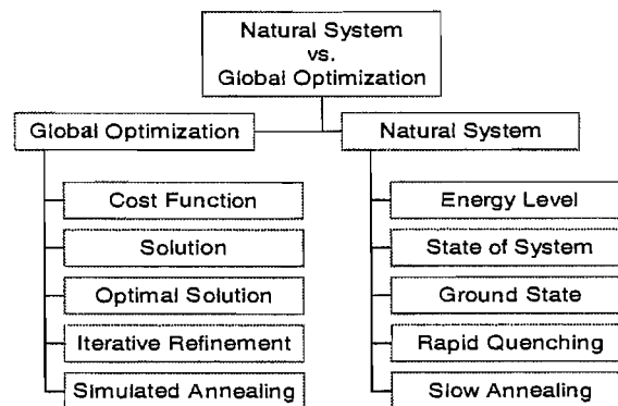
FIGURE 37.2 A one-to-one analogy between a natural process and global optimization.
