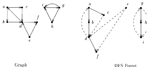
FIGURE 6.3 Sample execution of DFS on a directed graph.
