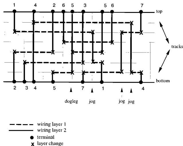
FIGURE 23.10 A channel routing in the 2-layer Manhattan model showing jogs.
