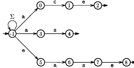
FIGURE 11.8 A straightforward nondeterministic automaton with only one initial state that accepts the language \Sigma^*X for pattern X = \{\text{ace, as, ease}\} . The edge labeled by \Sigma denotes the card \Sigma edges labeled by the card \Sigma distinct symbols in \Sigma .
