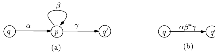
FIGURE 24.7 Converting an NFA to a regular expression.
