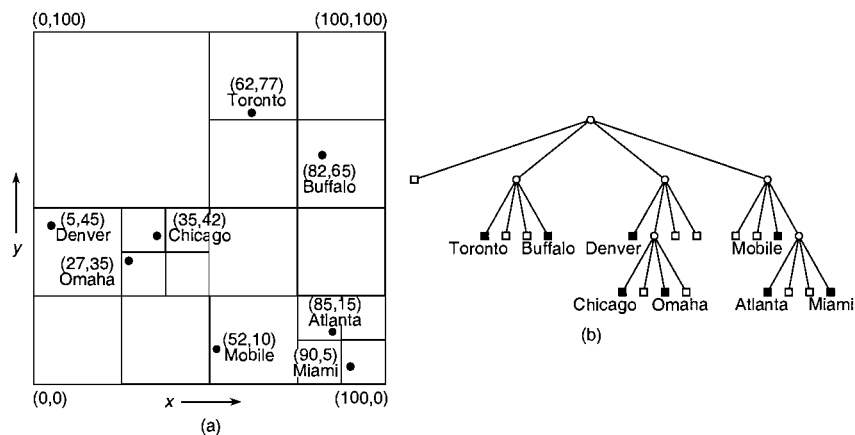
FIGURE 18.3 A PR quadtree and the records it represents corresponding to Fig.18.1: (a) the resulting partition of space, and (b) the tree representation.
