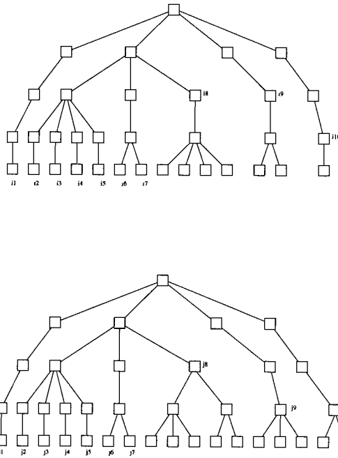
FIGURE 22.6 The matching set M = \{(i_t, j_t)\} of two trees.
