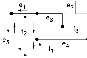
Figure 9.14 A graph and its orthogonal representation.
