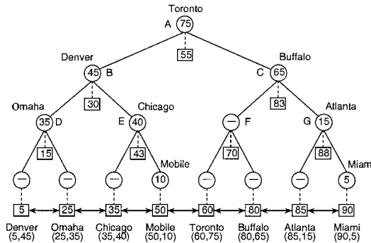
FIGURE 18.4 Priority search tree for the data of Fig. 18.1. Each leaf node contains the value of its x coordinate in a square box. Each nonleaf node contains the appropriate x coordinate midrange value in a box using a link drawn with a broken line. Circular boxes indicate the value of the y coordinate of the point in the corresponding subtree with the maximum value for its y coordinate that has not already been associated with a node at a shallower depth in the tree.
