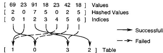
FIGURE 47.6 Each key attempts to write its index into a hash table entry.
