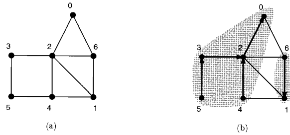
FIGURE 47.10 Tree-based graph contraction. (a) A graph G . (b) The hook edges induced by hooking larger to smaller vertices and the subgraphs induced by the trees.
