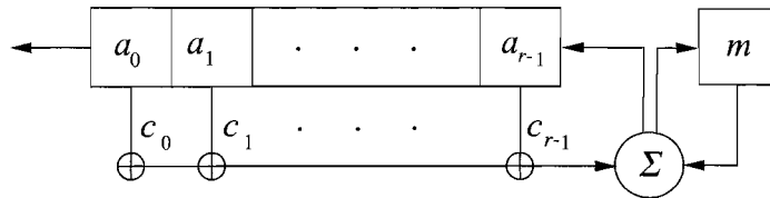
FIGURE 43.3 Feedback with carry shift register.
