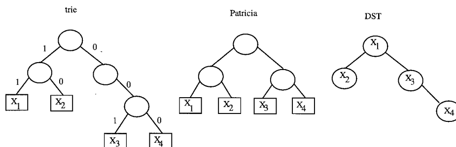
FIGURE 14.1 A trie, Patricia trie, and a digital search tree (DST) built from the following four strings X_1 = 11100\dots , X_2 = 10111\dots , X_3 = 00110\dots , and X_4 = 00001\dots .
