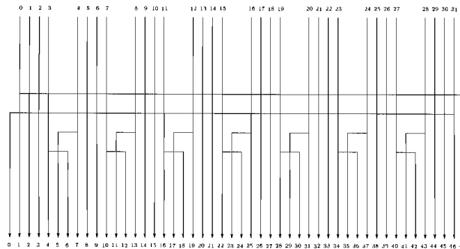
FIGURE 38.2 DES block diagram of f(R, K) .
