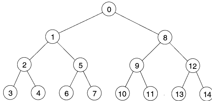
FIGURE 36.3 Order of node generation for depth-first search.
