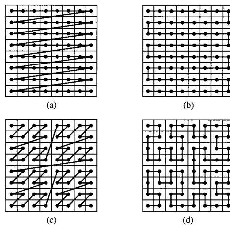
FIGURE 18.9 The result of applying four common different space-ordering methods to an 8 \times 8 collection of cells whose first element is in the upper-left corner: (a) row order, (b) row-prime order, (c) Morton order, (d) Peano-Hilbert.
