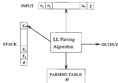
FIGURE 25.3 A schematic illustration of the LL parser.
