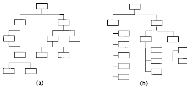
Figure 9.5 (a) Tree drawn with the Reingold-Tilford algorithm and (b) tip-over drawing of a tree.
