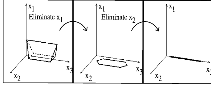
FIGURE 31.1 Variable elimination and projection.
