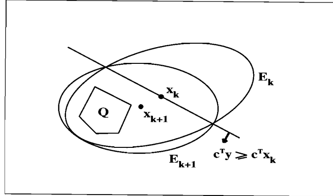
FIGURE 31.3 Shrinking ellipsoids.
