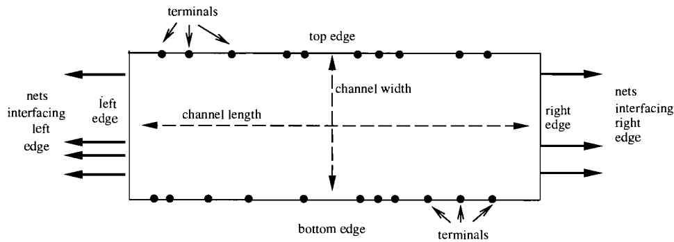
FIGURE 23.8 A channel. Nets interfacing at the left and right edges are not in a given order.
