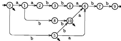
FIGURE 11.12 The suffix automaton \mathcal{S}(y) of the string y = \text{aabbabb} . The states are numbered from 0 to 10, according to the order in which they are created by the construction algorithm described in the present section. The initial state is state 0, terminal states are states 0, 5, 9, and 10. This automaton is the minimal deterministic automaton accepting the language of the suffixes of y .
