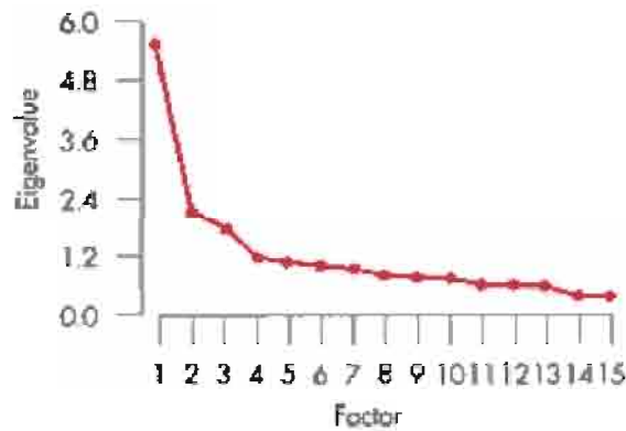
FIGURE 15-4 A scree plot for the 15 factors.
