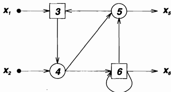
Figure 8.11. A simple recurrent network.
