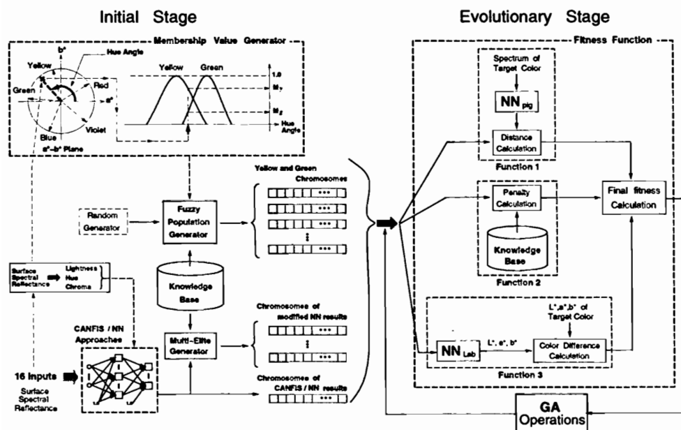
Figure 22.6. Architecture of color paint manufacturing intelligence.
