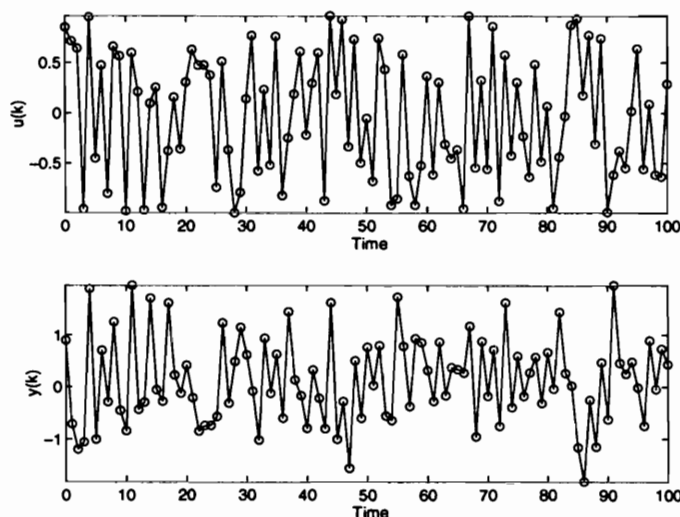
Figure 17.6. Collecting training data for inverse control, where the upper plot is u(k) and the lower one is y(k) . (MATLAB file: inv_sig.m )
