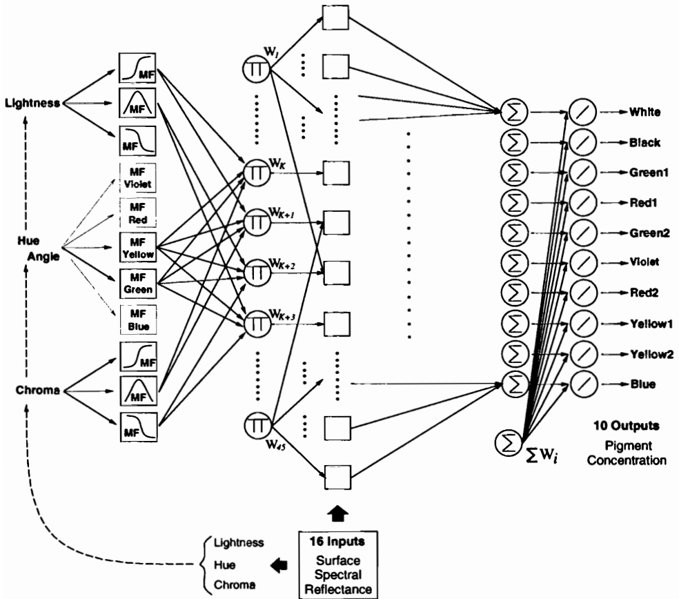
Figure 22.4. CANFIS with 11 MFs (45 fuzzy rules) for color recipe prediction.
