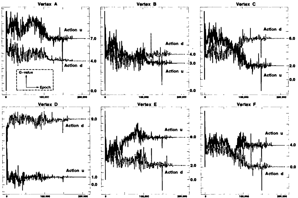
Figure 10.11. The Q-learning curves for the six non-terminal vertices obtained using a Q-net with one hidden layer ( 3 \times 5 \times 1 ). The horizontal axis represents the epoch number and the vertical axis shows the Q-value.
