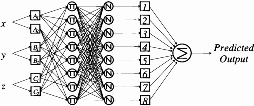
Figure 12.10. The ANFIS model for Example 2. (The connections from inputs to layer 4 are not shown.)
