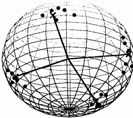
Figure 11.2. Competitive learning with unit-length vectors. The dots represent the input vectors and the crosses denote the weight vectors for the four output units in Figure 11.1. As the learning continues, the four weight vectors rotate toward the centers of the four input clusters. (MATLAB command: compball)
