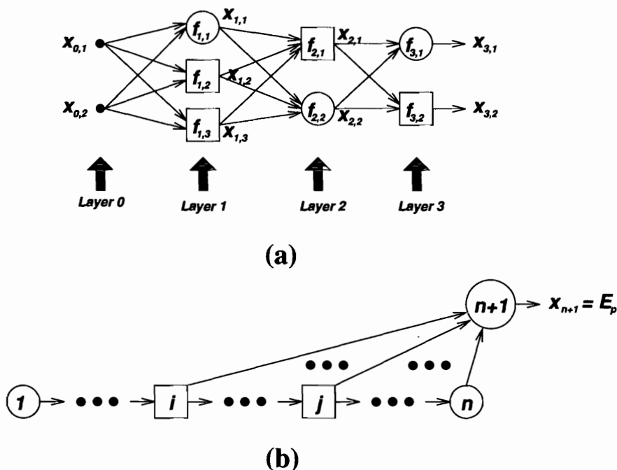
Figure 8.8. Our notational conventions: (a) layered representation; (b) topological ordering representation.
