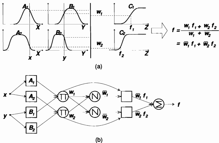
Figure 12.3. (a) A two-input two-rule Tsukamoto fuzzy model; (b) equivalent ANFIS architecture.
