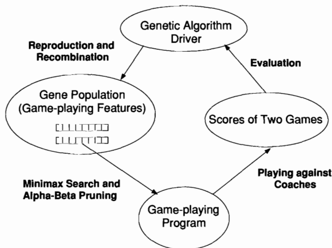
Figure 21.2. GA training of Othello players.
