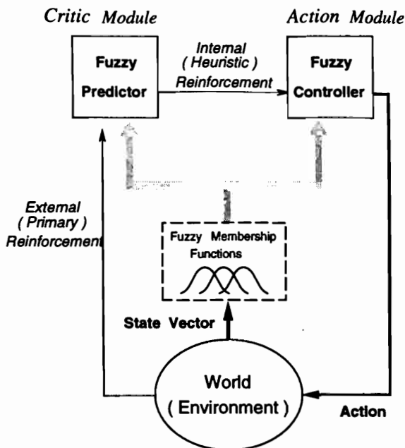
Figure 18.2. A neuro-fuzzy AHC model.
