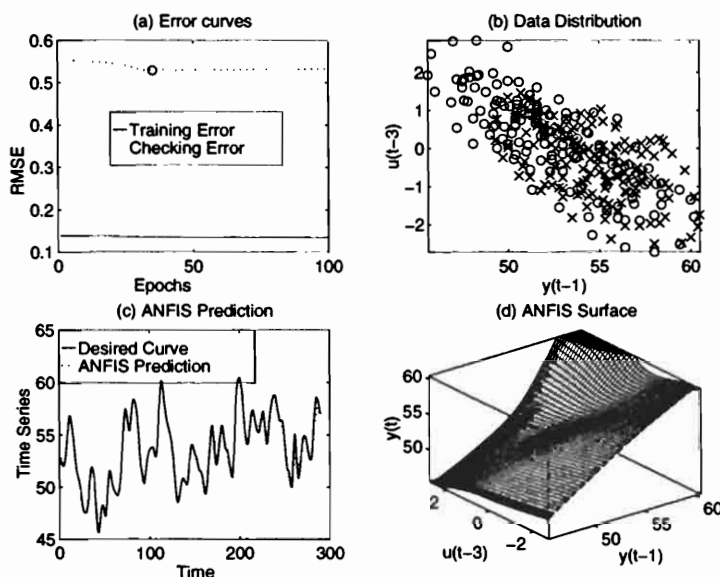
Figure 19.13. ANFIS for Box-Jenkins data: (a) training and checking error curves; (b) training and checking data distribution; (c) desired system response and ANFIS prediction; (d) ANFIS surface. . (MATLAB file: bjtrain.m )
