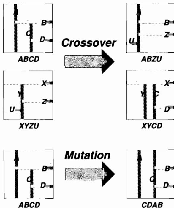
Figure 18.7. Crossover and mutation for input space partitioning.
