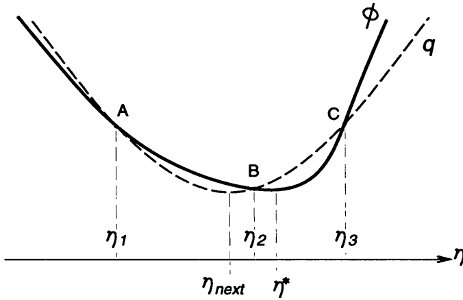
Figure 6.9. Quadratic interpolation .
