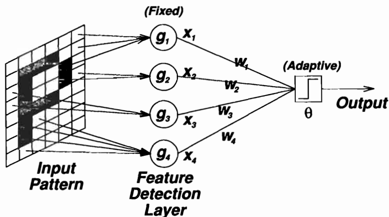
Figure 9.1. The perceptron.
