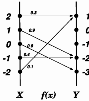
Figure 3.1. Extension principle on fuzzy sets with discrete universes.
