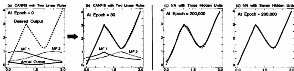
Figure 13.10. Results of N-shape problem obtained by ANFIS: CANFIS with two linear rules (a, b), and a simple backpropagation MLP with three hidden units (c) and with seven hidden units (d).
