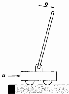
Figure 17.2. The inverted pendulum system.
