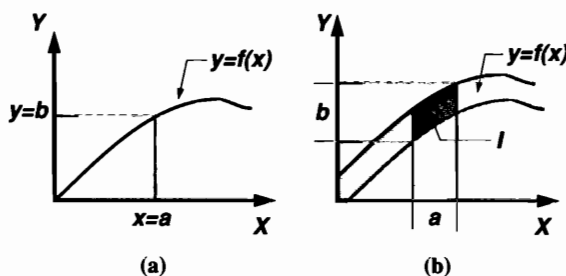
Figure 3.10. Derivation of y = b from x = a and y = f(x) : (a) a and b are points, y = f(x) is a curve; (b) a and b are intervals, y = f(x) is an interval-valued function.
