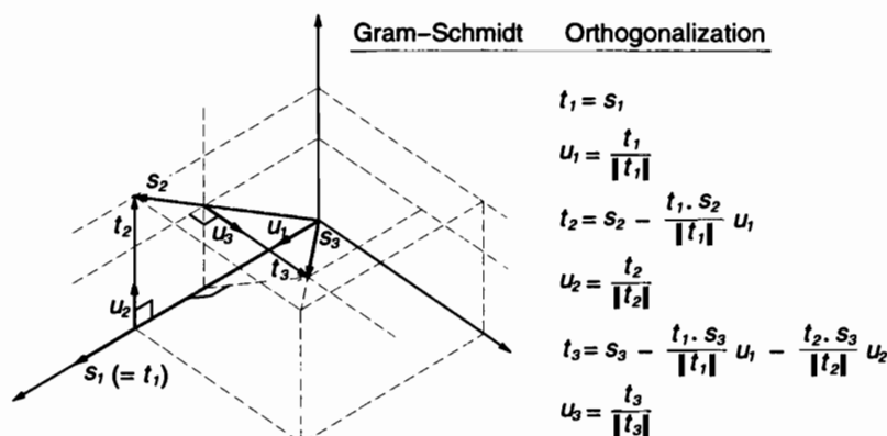
Figure 6.12. The procedures of the Gram-Schmidt orthogonalization. As an example, given three vectors s_1 , s_2 , and s_3 , three mutually orthogonal vectors u_1 , u_2 , and u_3 are produced. In other words, the step-by-step Gram-Schmidt process in Equation (6.42) converts an arbitrary basis \{s_1, s_2, s_3\} into an orthonormal basis \{u_1, u_2, u_3\} .
