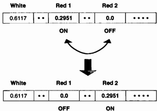
Figure 22.10. Exchanging mutation.
