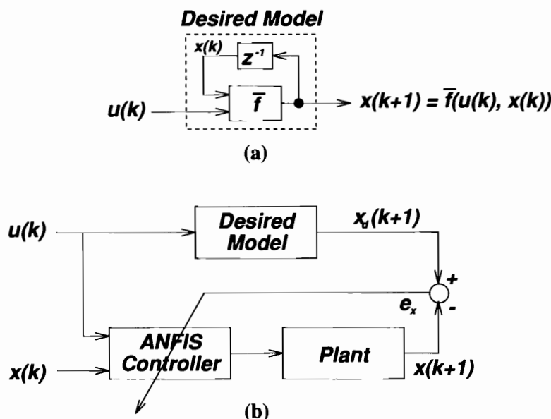
Figure 17.10. (a) Desired model block ; (b) specialized learning with model referencing .
