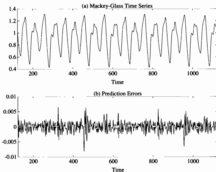
Figure 12.18. Example 3, (a) Mackey-Glass time series from t = 124 to 1123 and six-step-ahead prediction (which is indistinguishable from the time series here); (b) prediction error. (MATLAB file: trn_4in.m )
