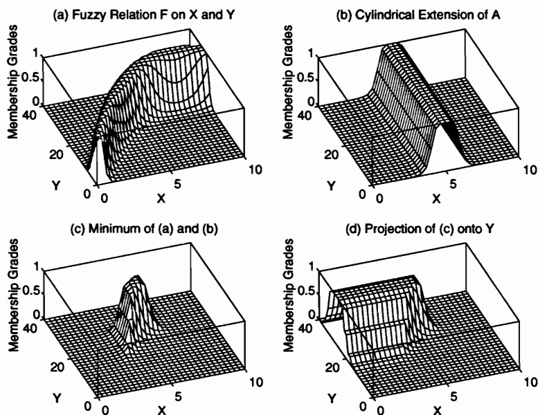
Figure 3.11. Compositional rule of inference. (MATLAB file: cri.m)
