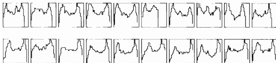
Figure 20.4. The x-axis and y-axis spectra of some training images. Upper row, left to right: the x-axis spectra of digit 0 to digit 9; lower row: the y-axis spectra of the same digits.
