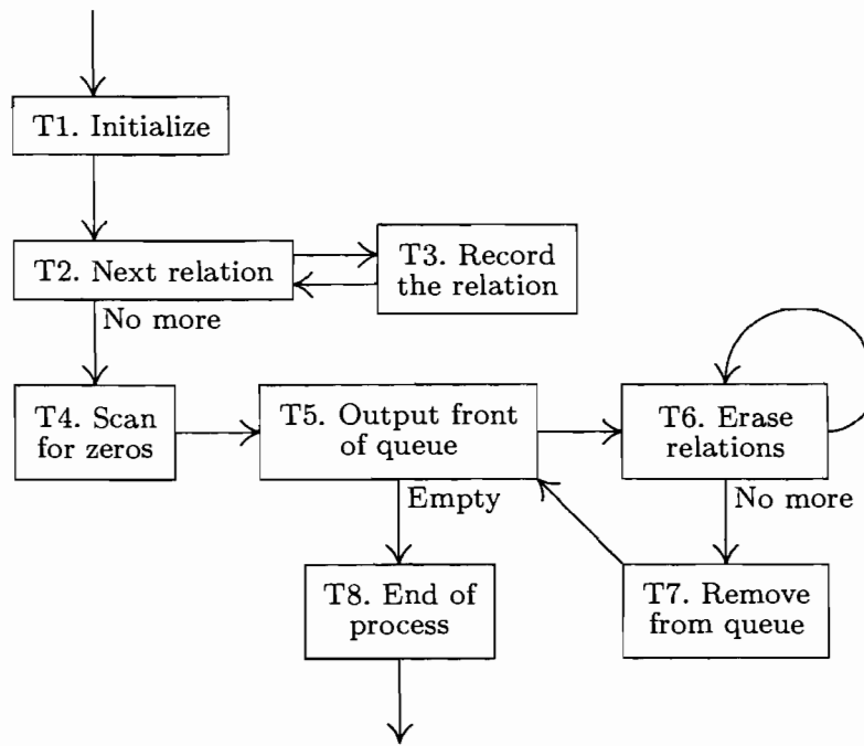
Fig. 9. Topological sorting.
