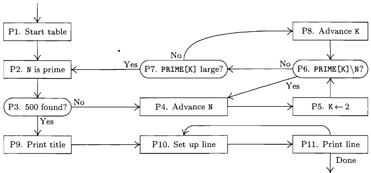
Fig. 14. Algorithm P.
