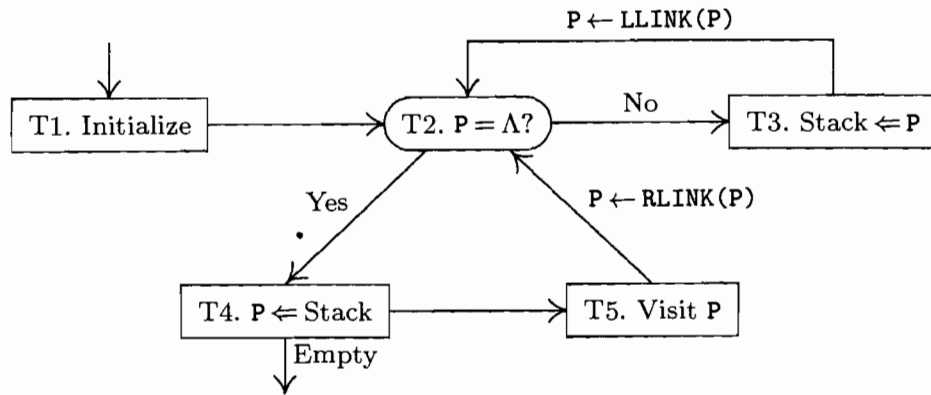
Fig. 23. Algorithm T for inorder traversal.
