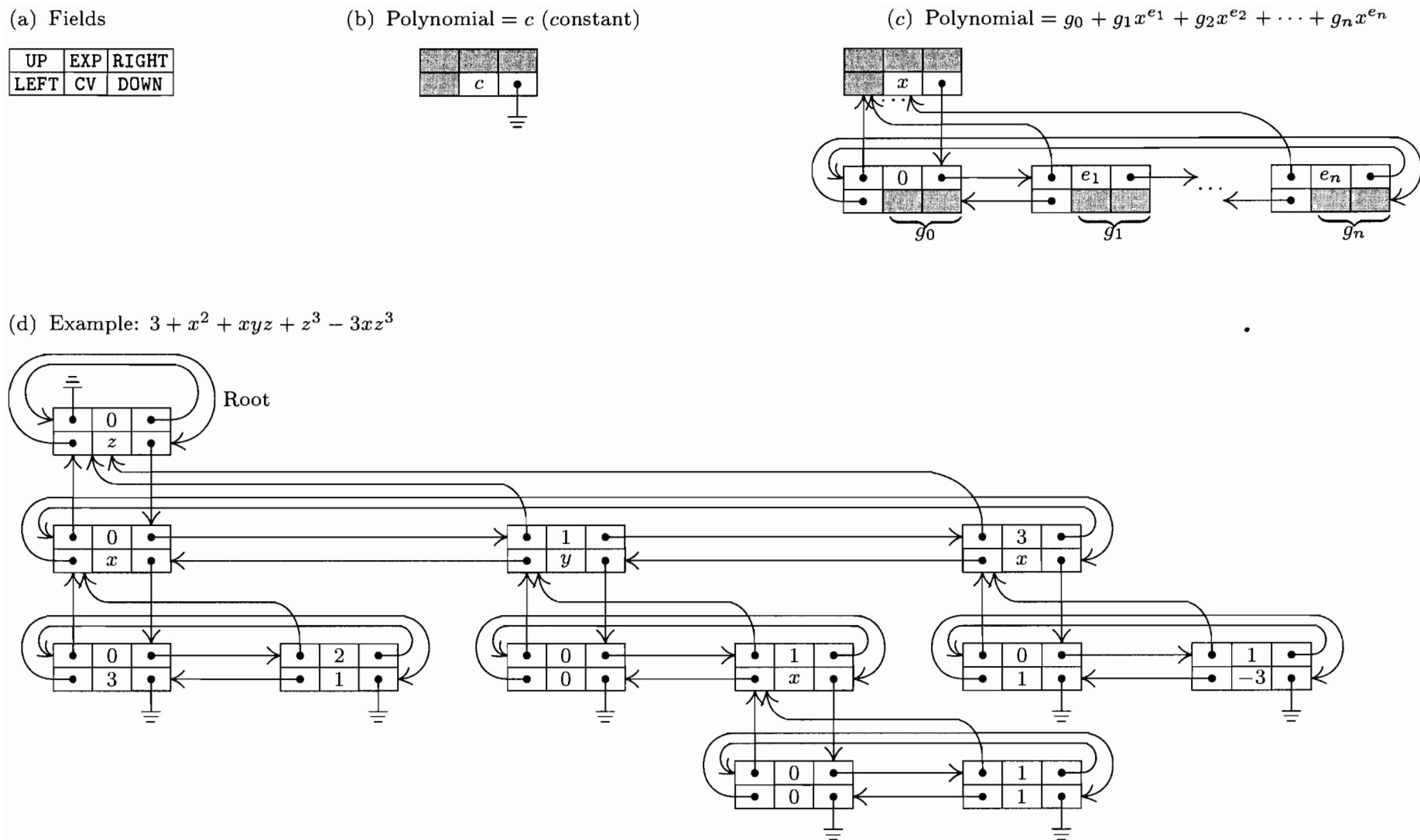
Fig. 28. Representation of polynomials using four-directional links. Shaded areas of nodes indicate information that is irrelevant in the context considered.
