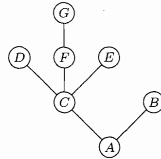
Fig. 16. Another tree.
