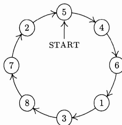
Fig. 17. Josephus's problem, n = 8 , m = 4 .
