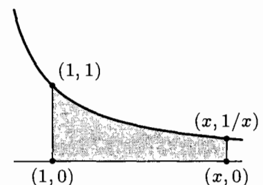
Fig. 6. Natural logarithm.
