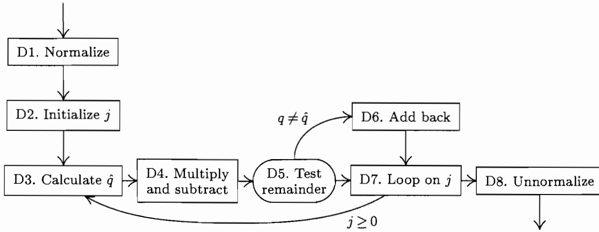
Fig. 7. Long division.
