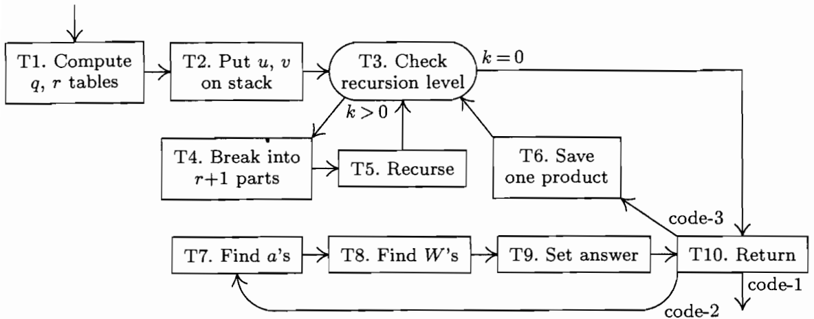
Fig. 8. The Toom-Cook algorithm for high-precision multiplication.
