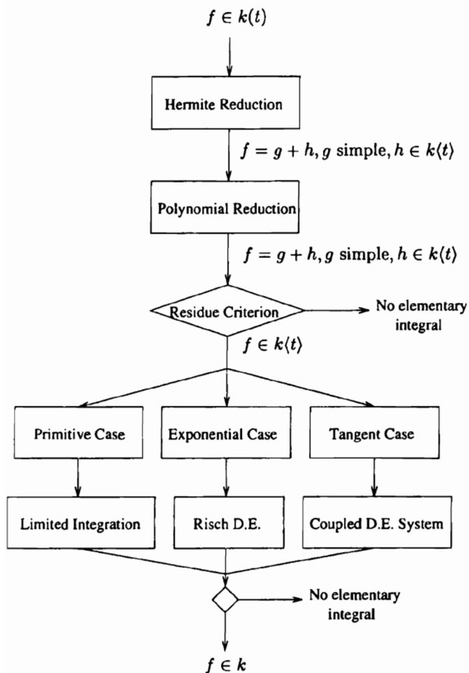
Fig. 5.1. General outline of the integration algorithm
